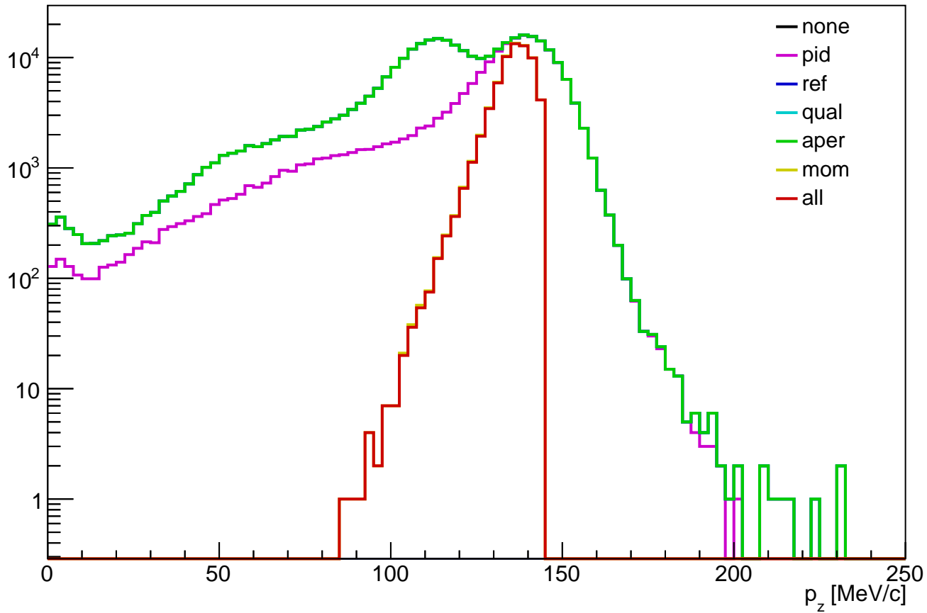
tku pz distribution (truth)
