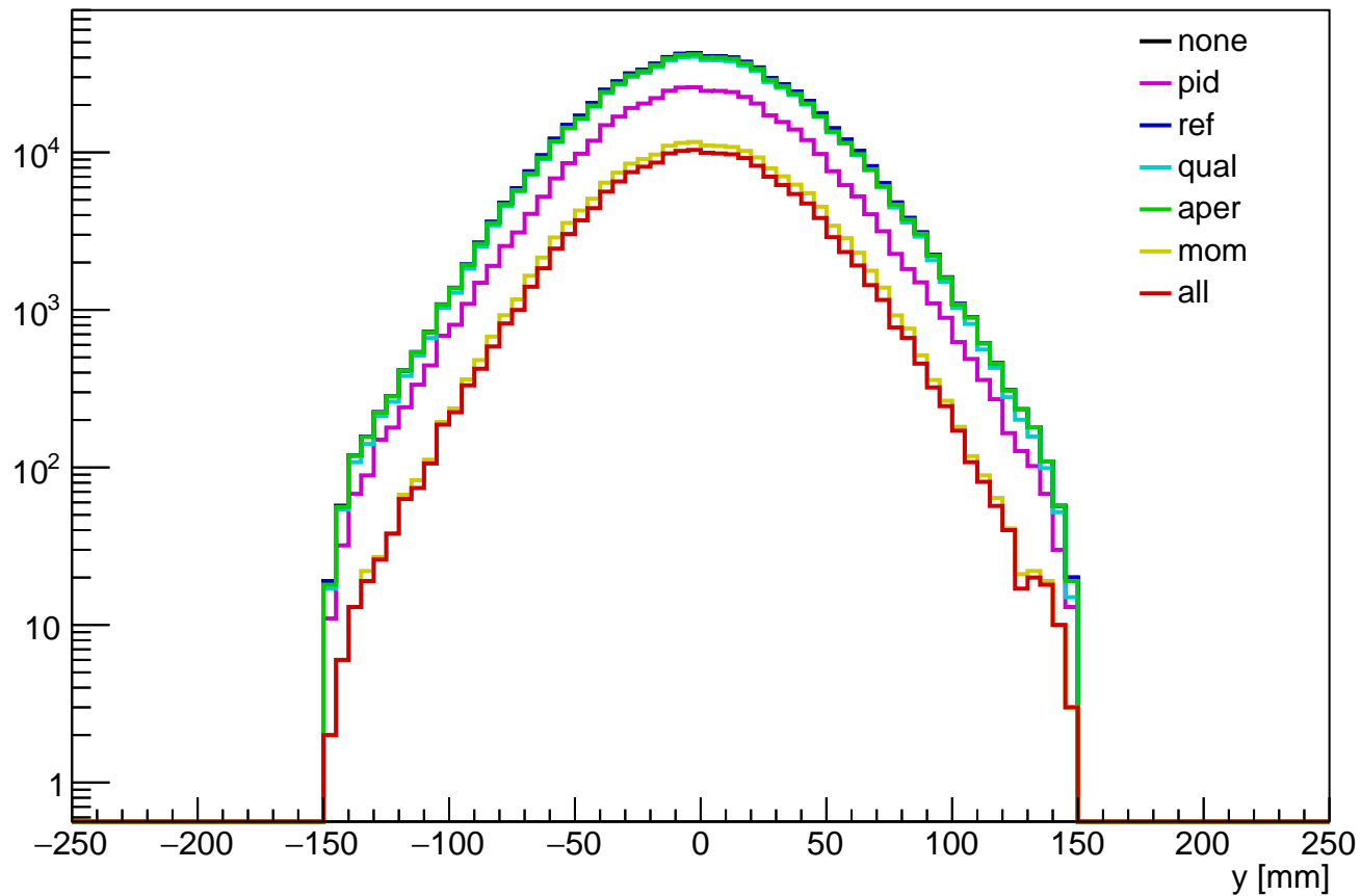
tktu y distribution (data)
