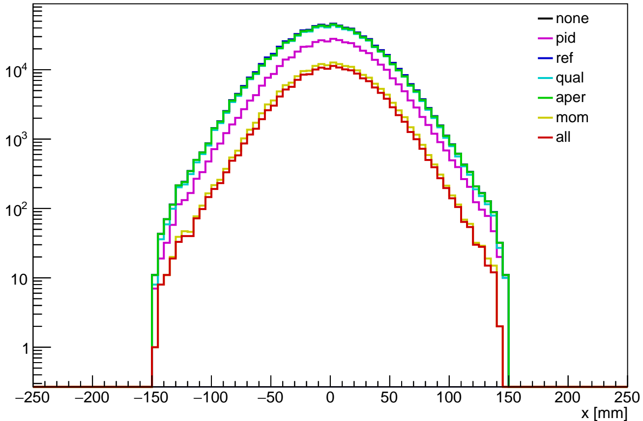
tku x distribution (data)
