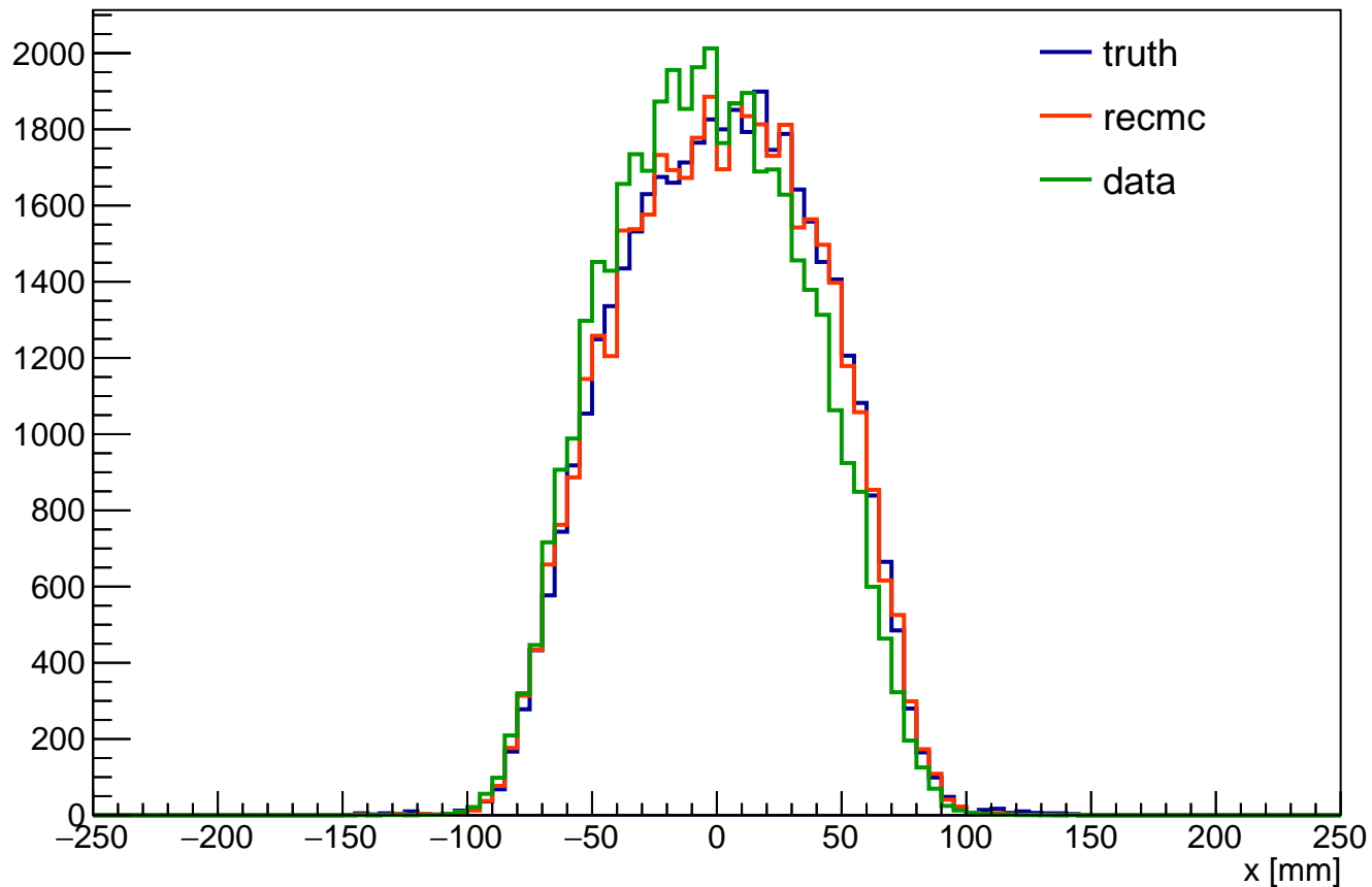
tkd x distribution (all cut)
