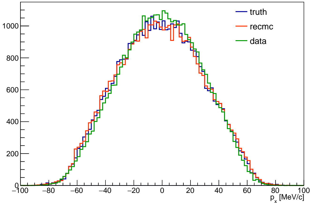
tkd px distribution (all cut)
