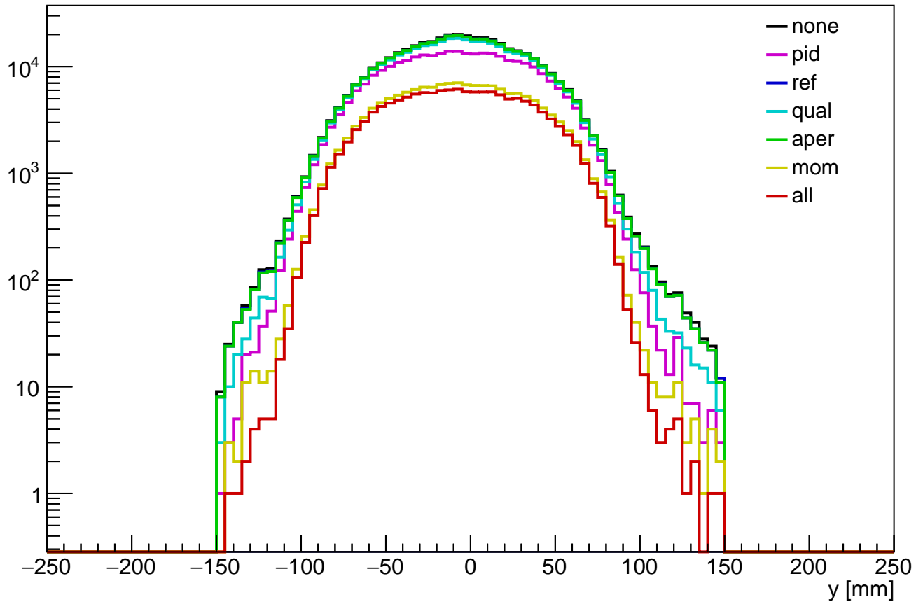
tkd y distribution (data)
