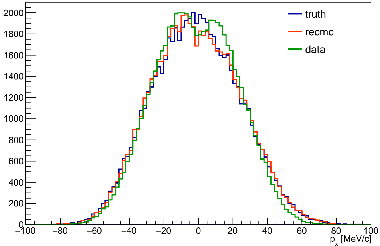
tku px distribution (all cut)
