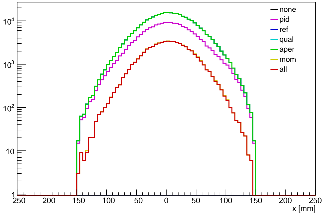
tku x distribution (truth)
