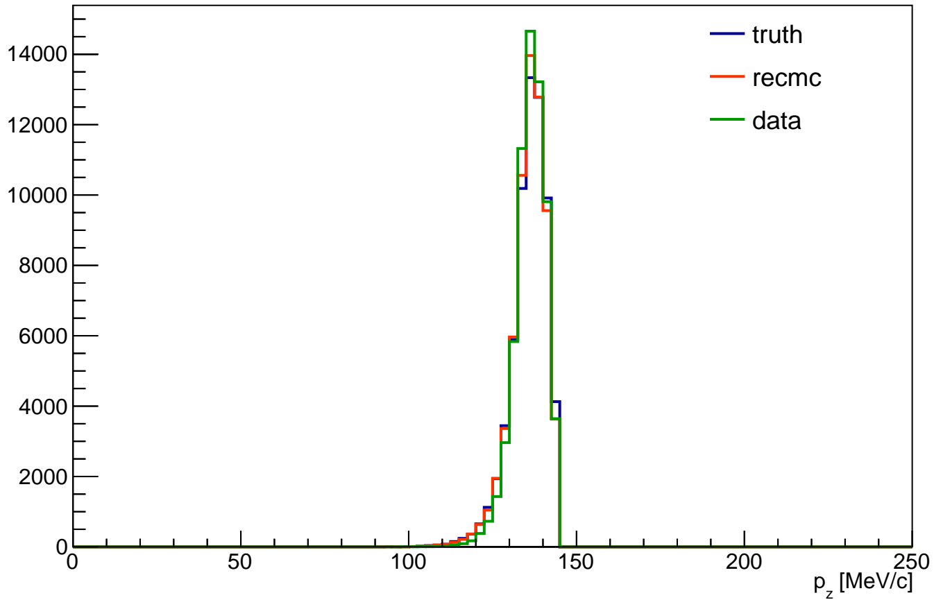
tku pz distribution (all cut)
