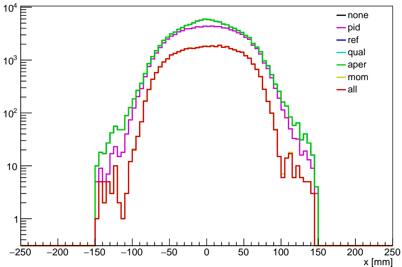
tkd x distribution (truth)
