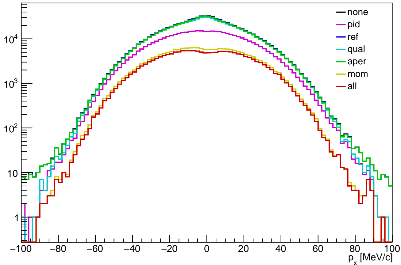
tku px distribution (data)
