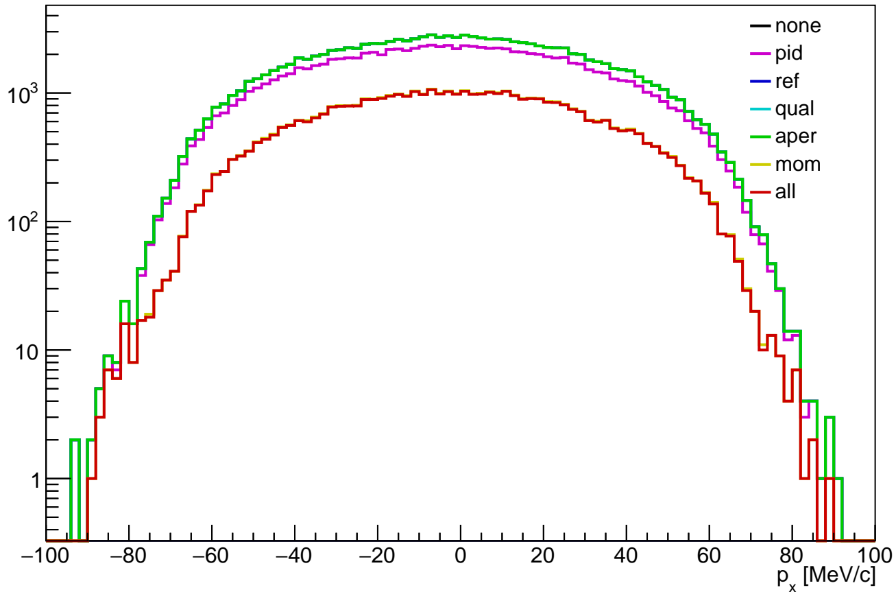
tkd px distribution (truth)
