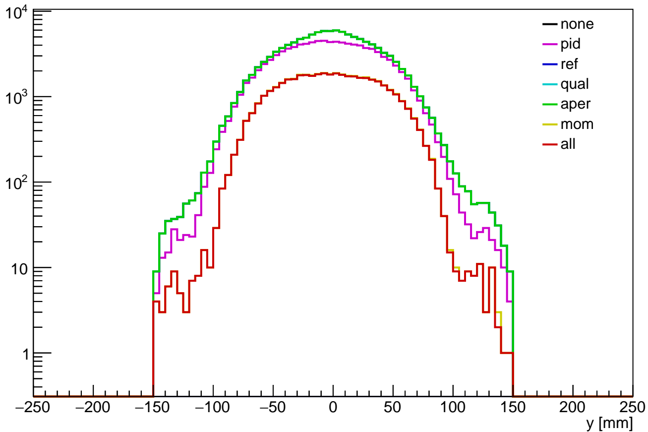
tkd y distribution (truth)
