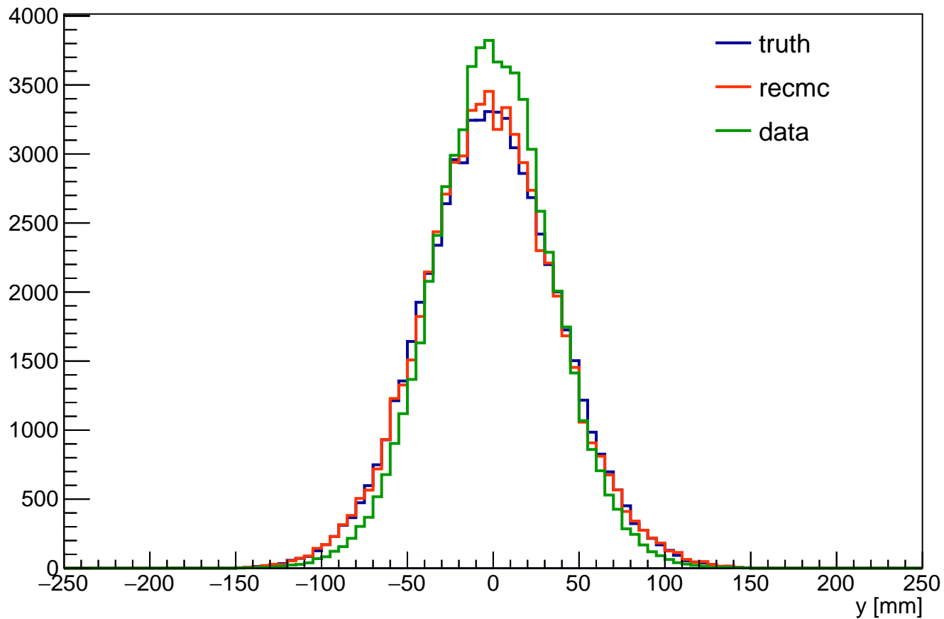
tku distribution (all cut)
