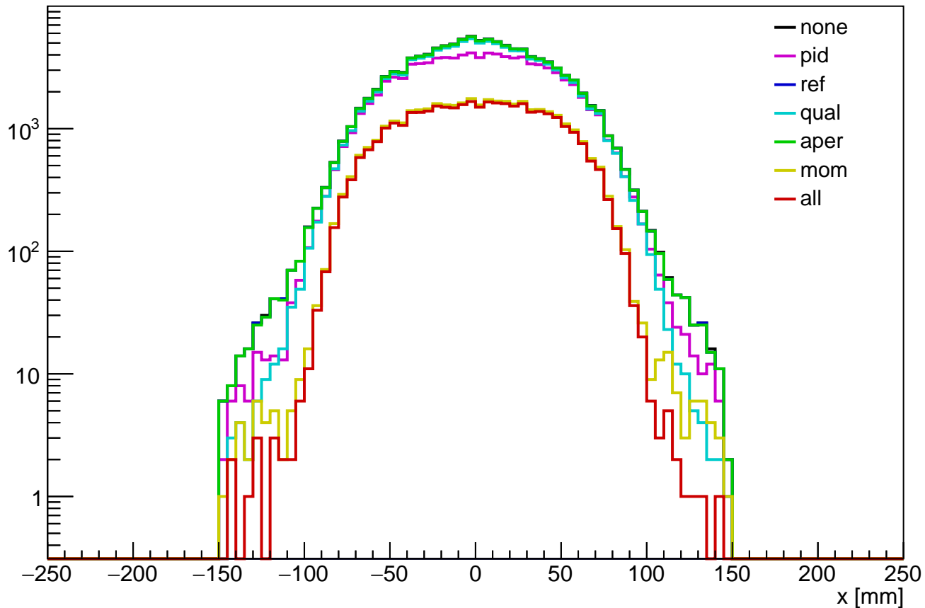
tkd x distribution (recmc)
