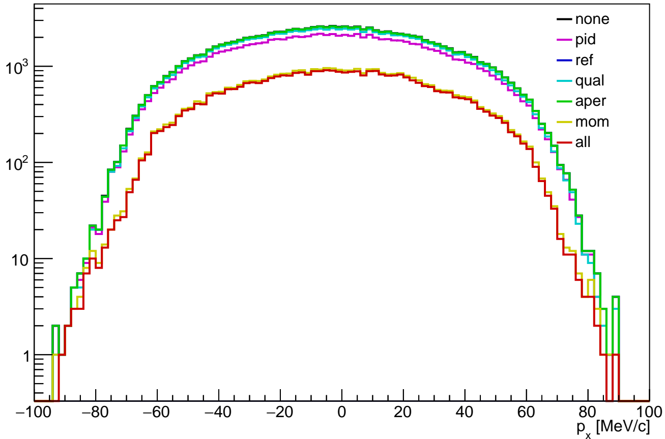
tkd px distribution (recmc)
