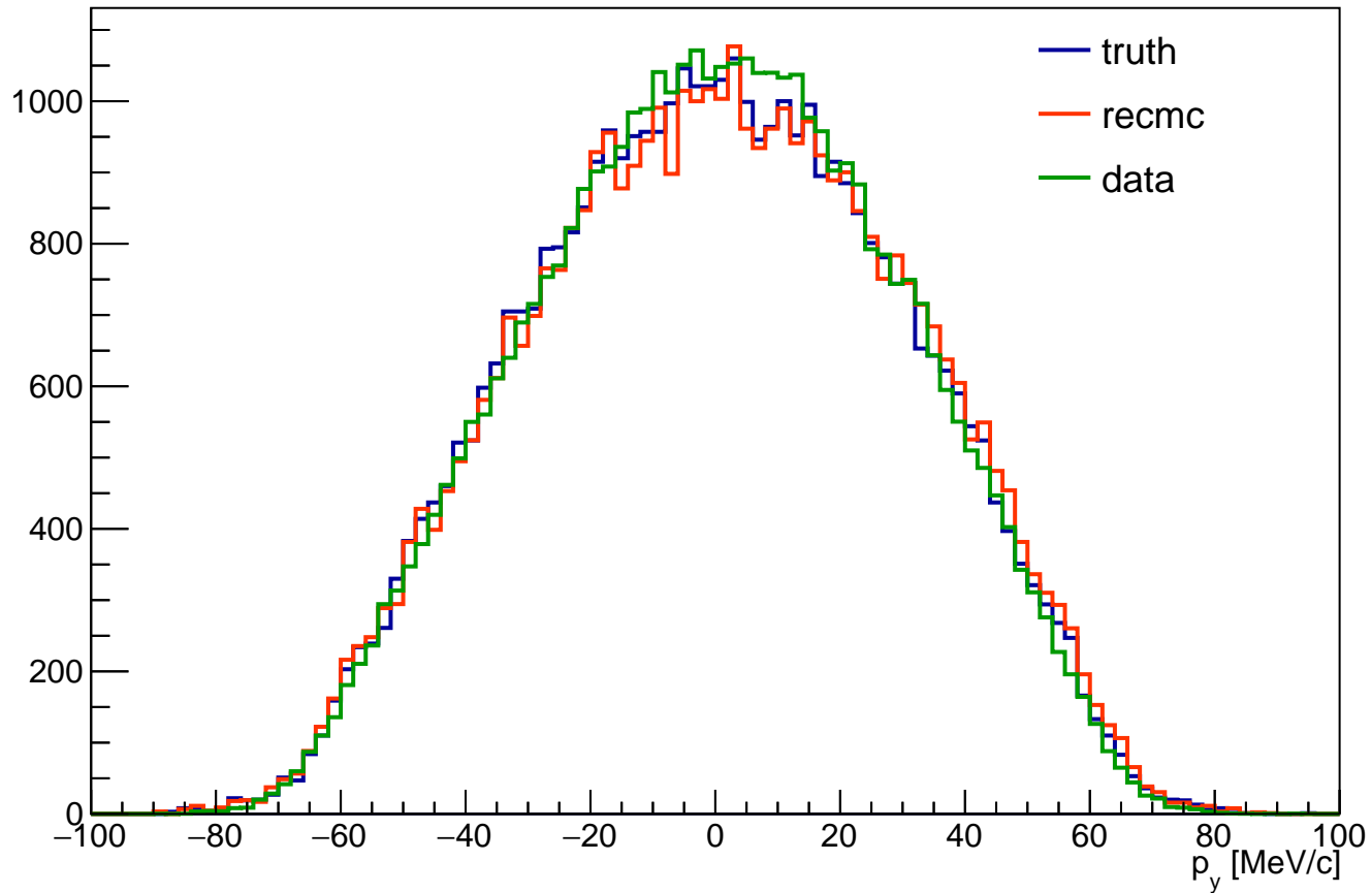
tkd py distribution (all cut)
