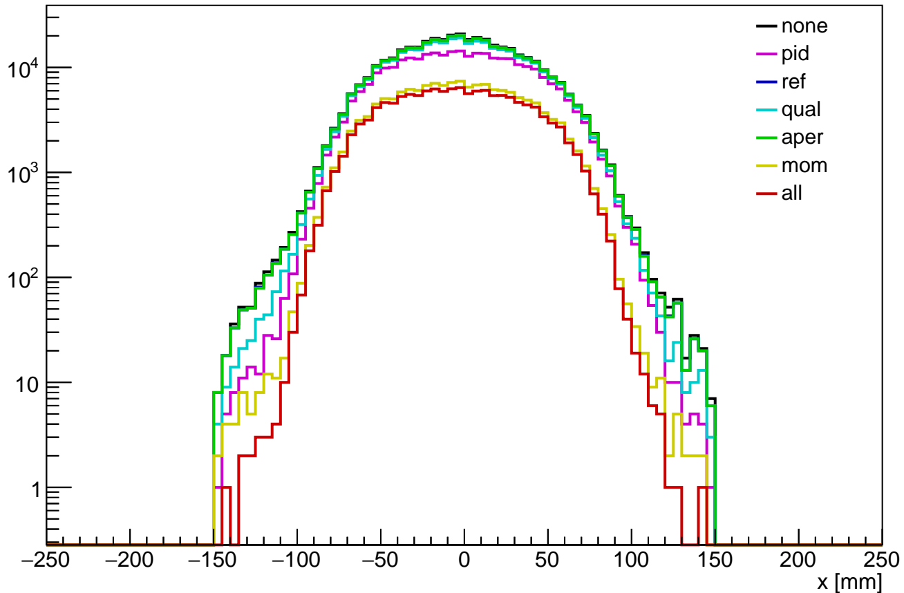
tkd x distribution (data)
