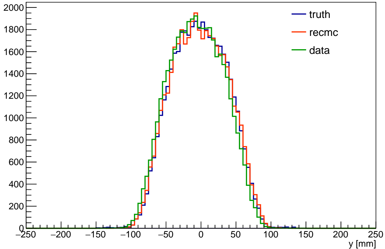
tkd distribution (all cut)
