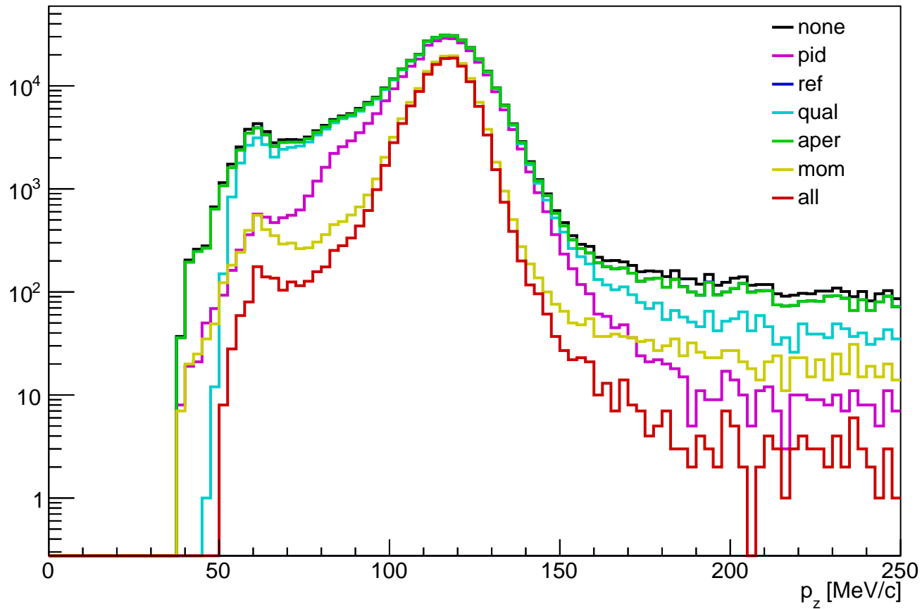
tkd pz distribution (data)
