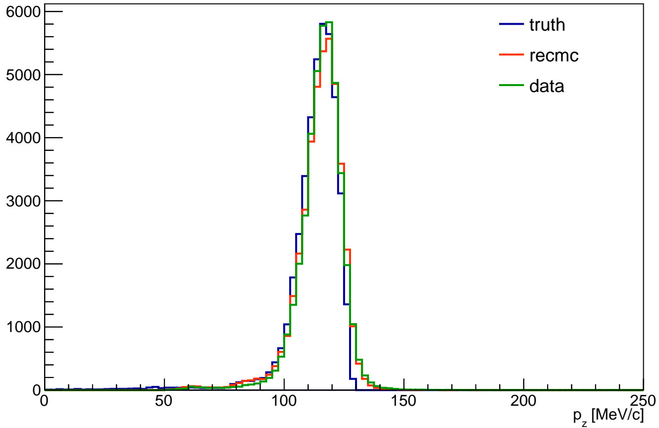
tkd pz distribution (all cut)
