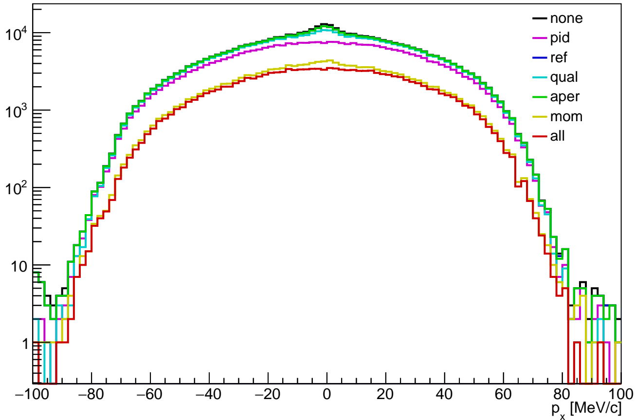
tkd px distribution (data)
