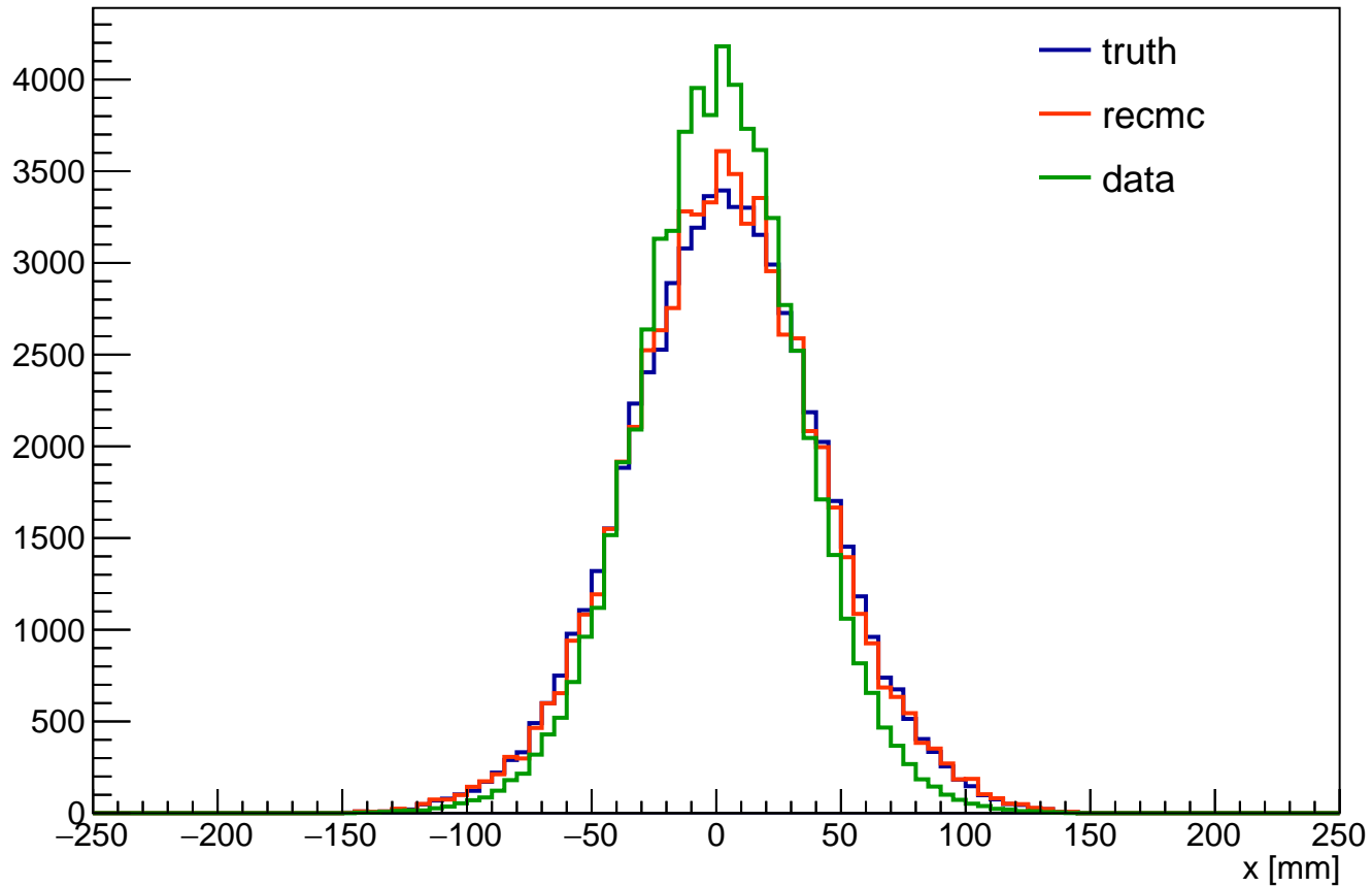
t ku x distribution (all cut)
