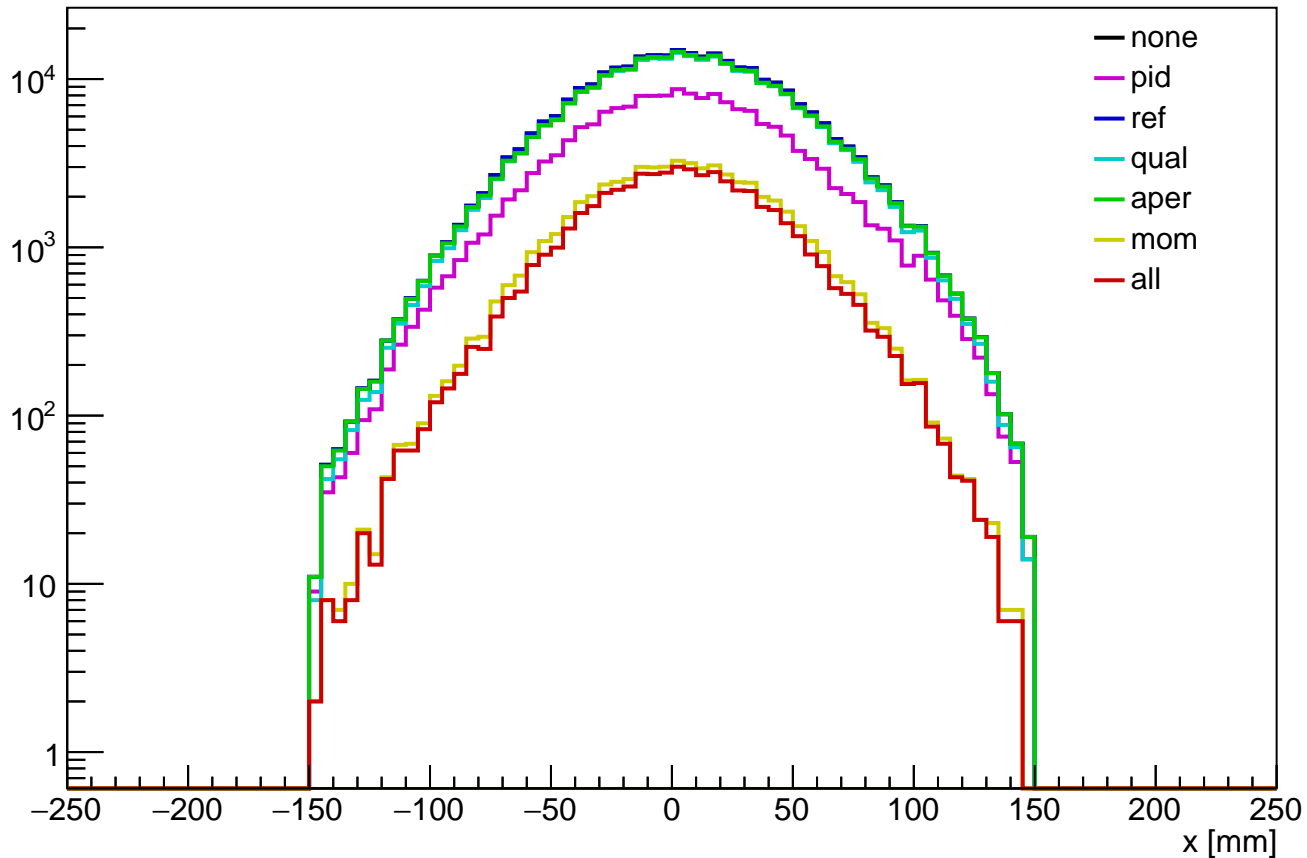
tku x distribution (recmc)
