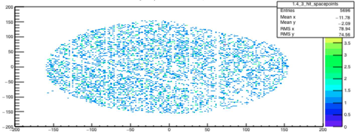
3-Cluster Spacepoints: Tracker 1, Station 4
