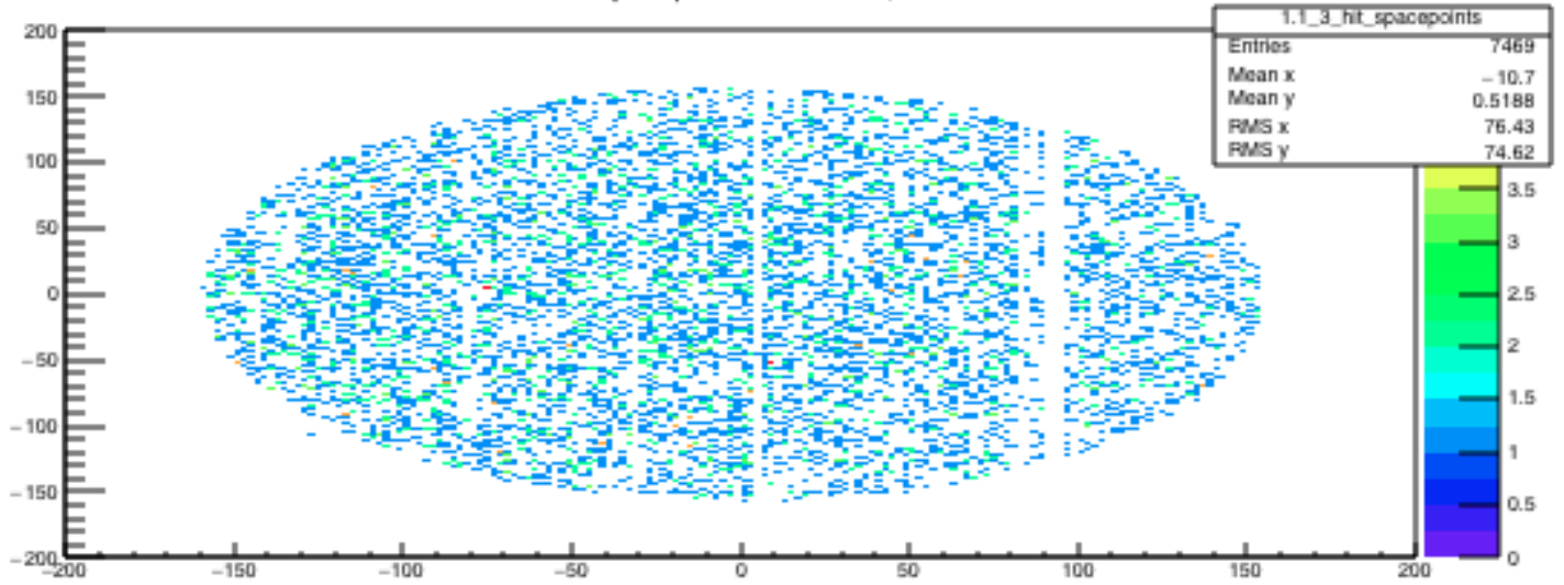
3-Cluster Spacepoints: Tracker 1, Station 1
