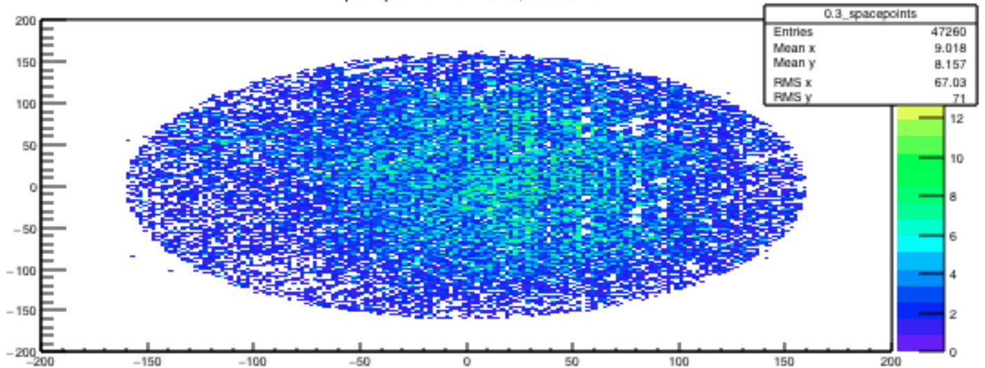
Spacepoints: Tracker 0, Station 3
