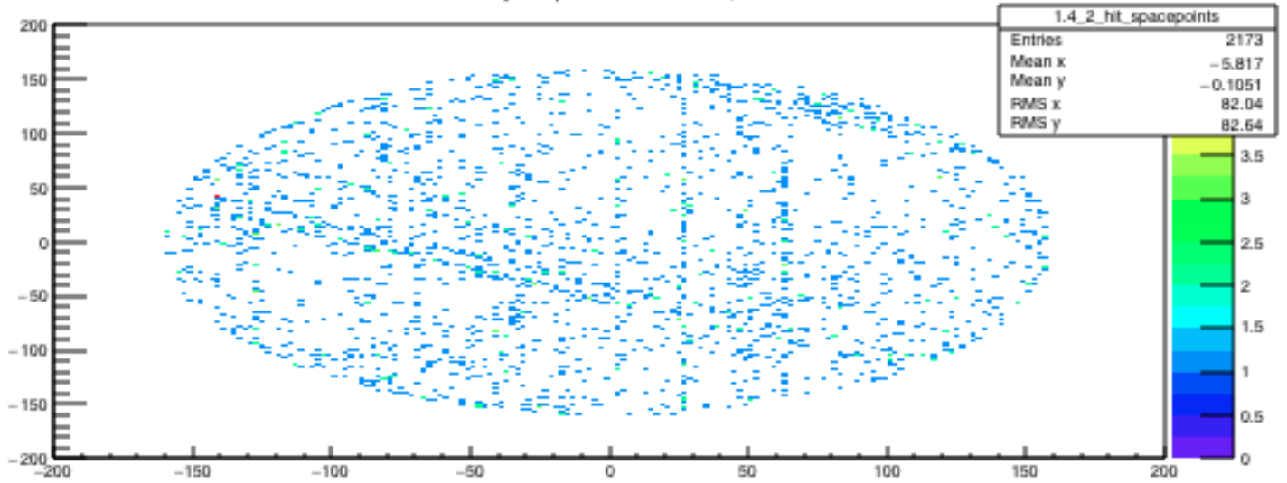
2-Cluster Spacepoints: Tracker 1, Station 4
