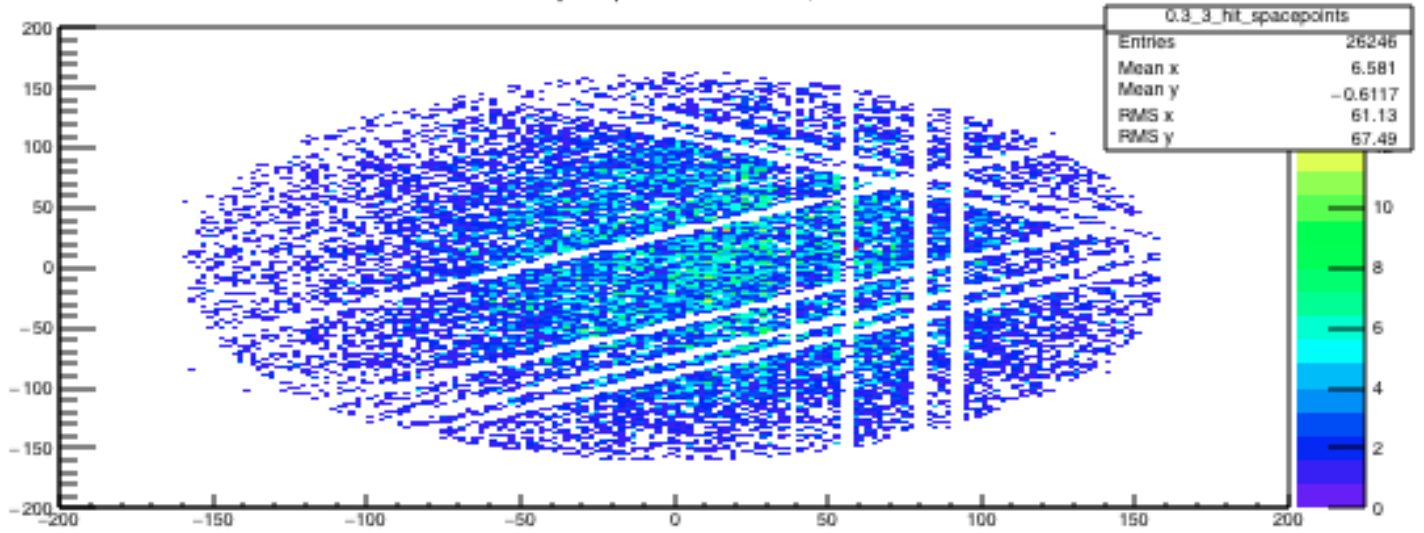
3-Cluster Spacepoints: Tracker 0, Station 3
