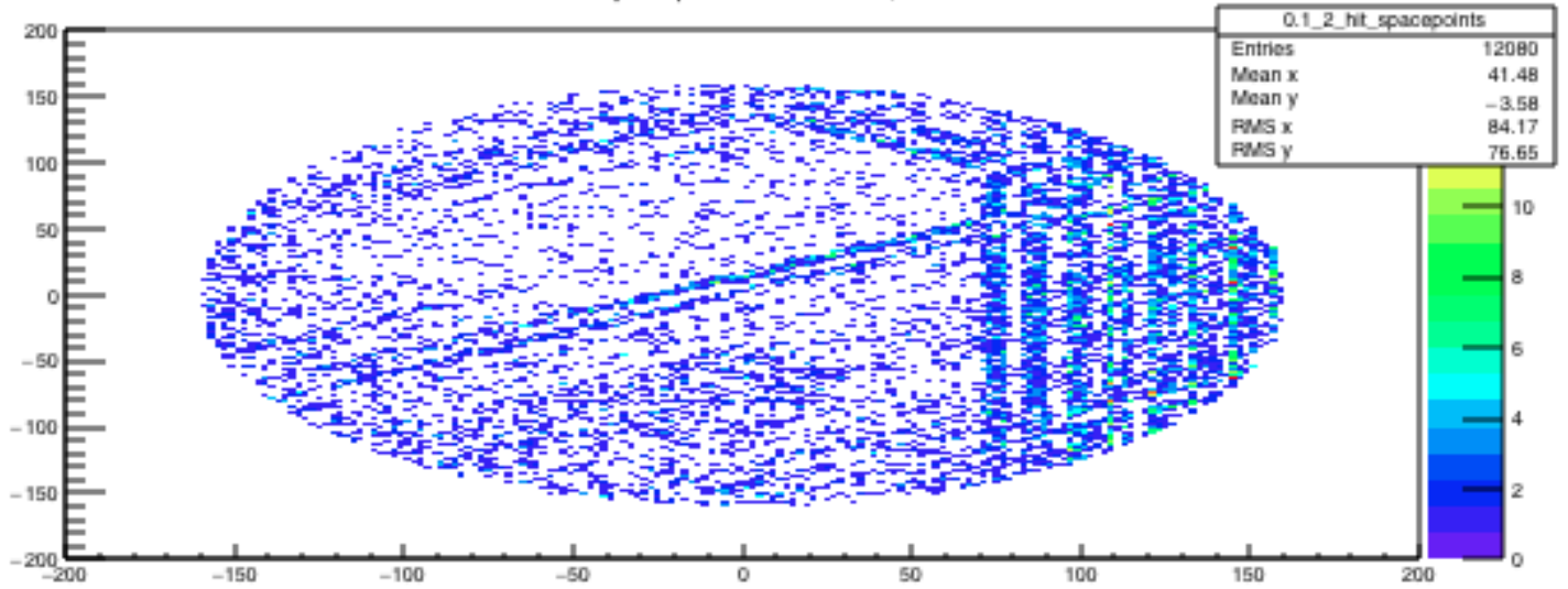
2-Cluster Spacepoints: Tracker 0, Station 1
