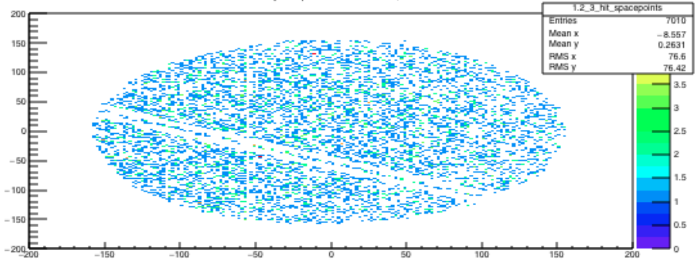
3-Cluster Spacepoints: Tracker 1, Station 2
