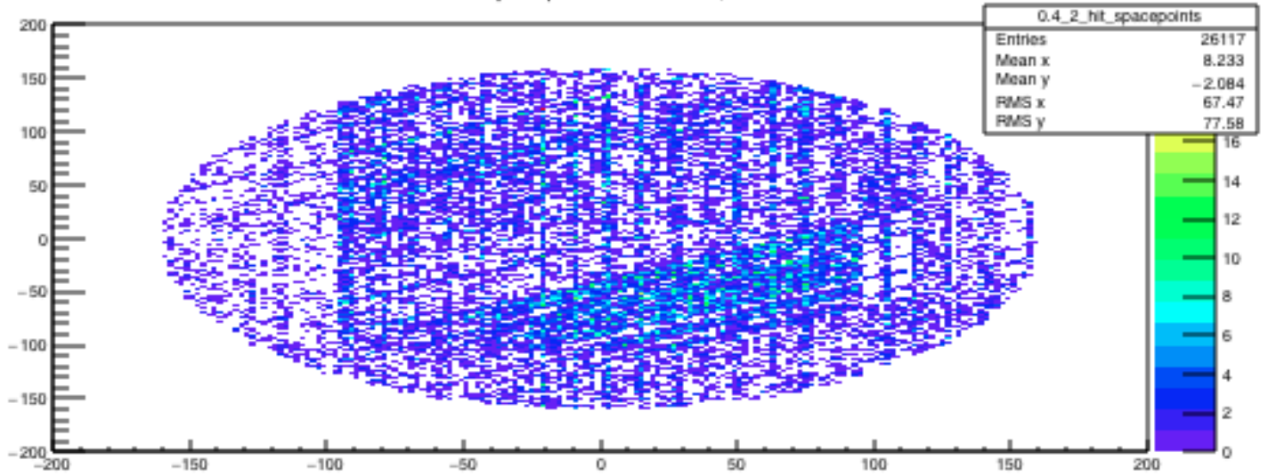
2-Cluster Spacepoints: Tracker 0, Station 4
