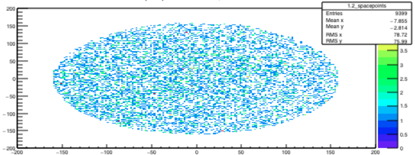
Spacepoints: Tracker 1, Station 2
