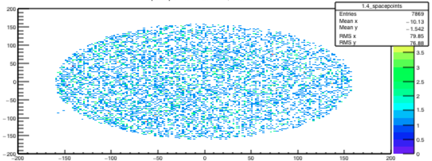
Spacepoints: Tracker 1, Station 4
