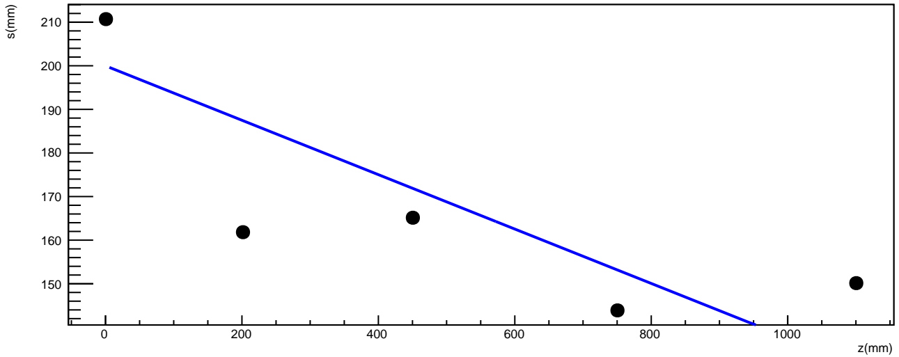
Seed s-z plot for tracker 1
