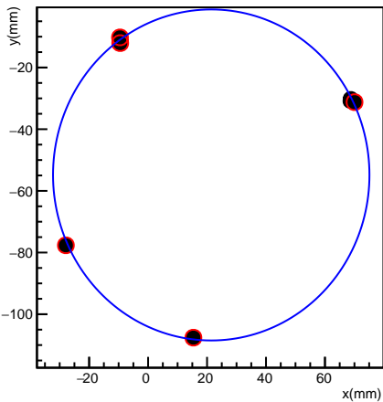
Spacepoint x-y plot for tracker 2
