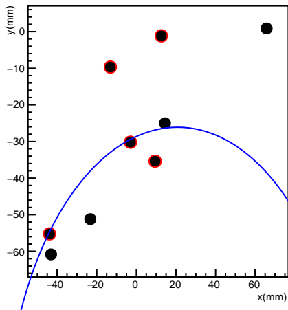
Spacepoint x-y plot for tracker 2
