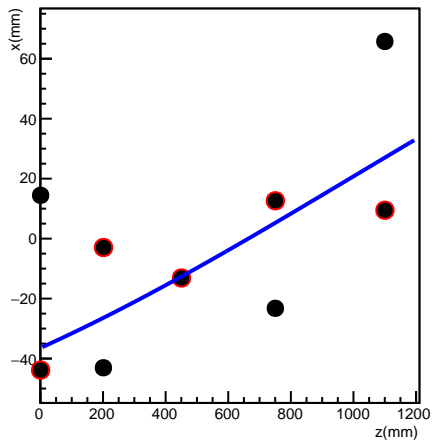
Spacepoint z-x plot for tracker 2
