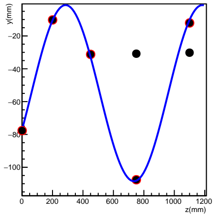
Spacepoint z-y plot for tracker 2
