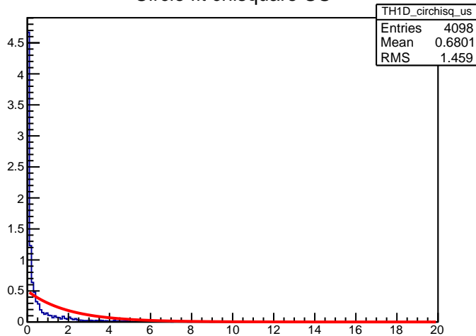
Circle fit chisquare US
