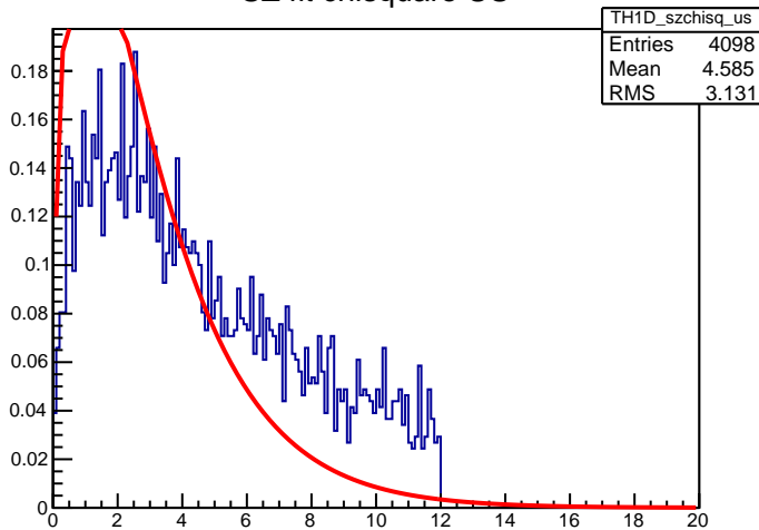
SZ fit chisquare US
