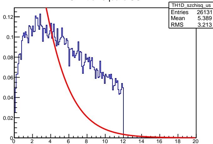
SZ fit chisquare US
