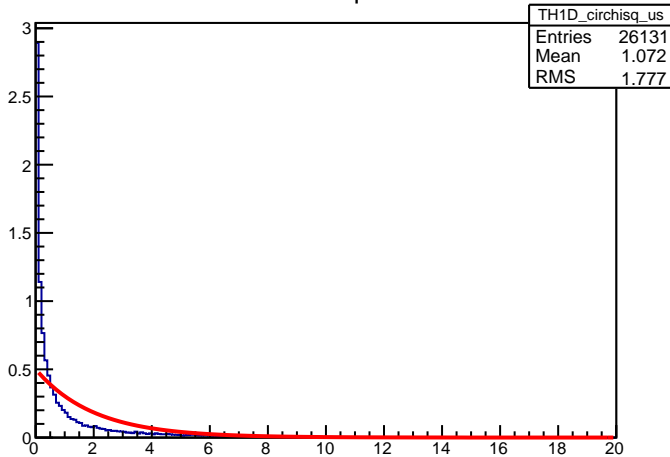
Circle fit chisquare US
