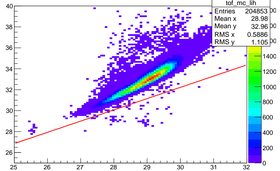
tof12:tof01
