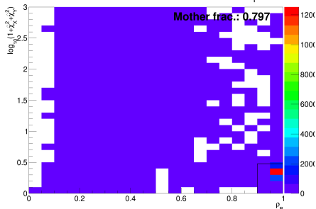
Normalised \chi^2 against plane density \rho_p
