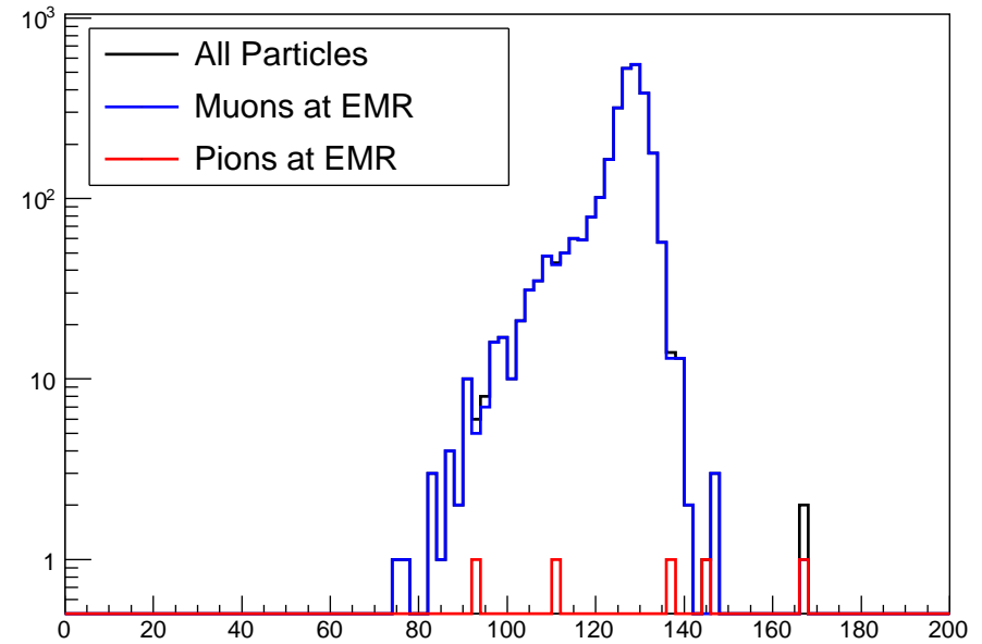
Mass From EMR Range and TOF12
