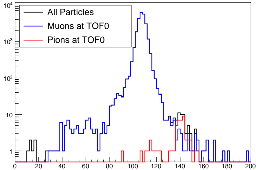
Mass From Tracker Momentum and TOF0
