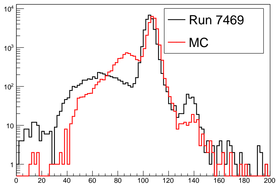
Mass From Tracker Momentum and TOF01
