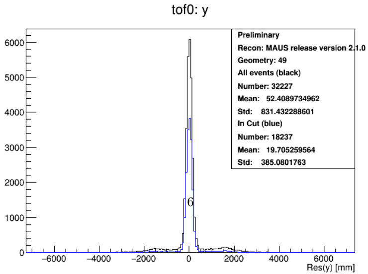
Figure 4: TOF0 residuals.
