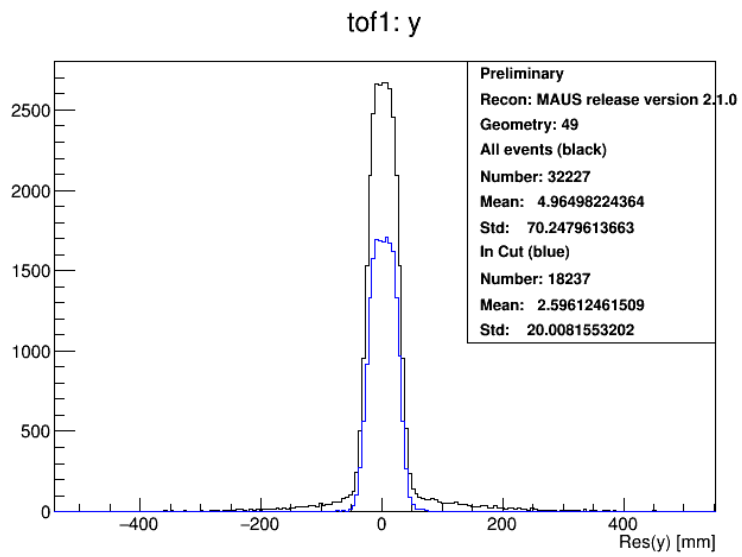
Figure 2: TOF1 residuals.
