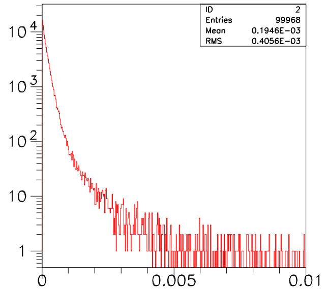
Theta squared
