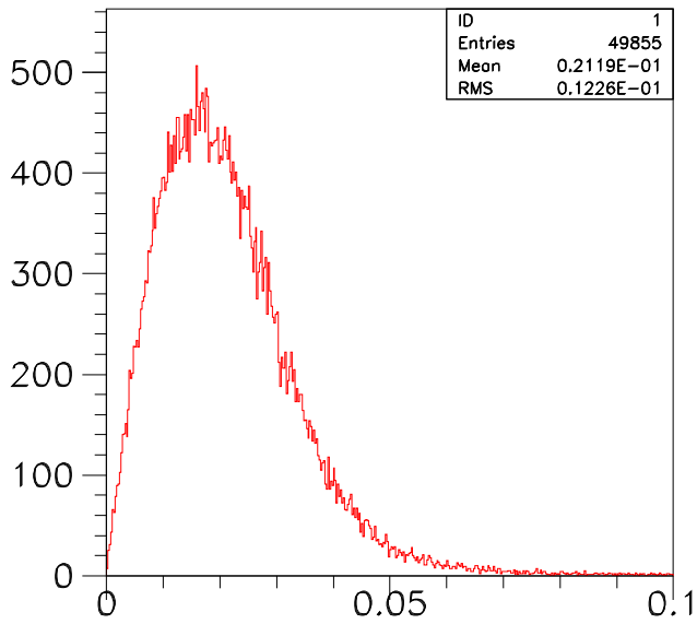
Theta, radians
