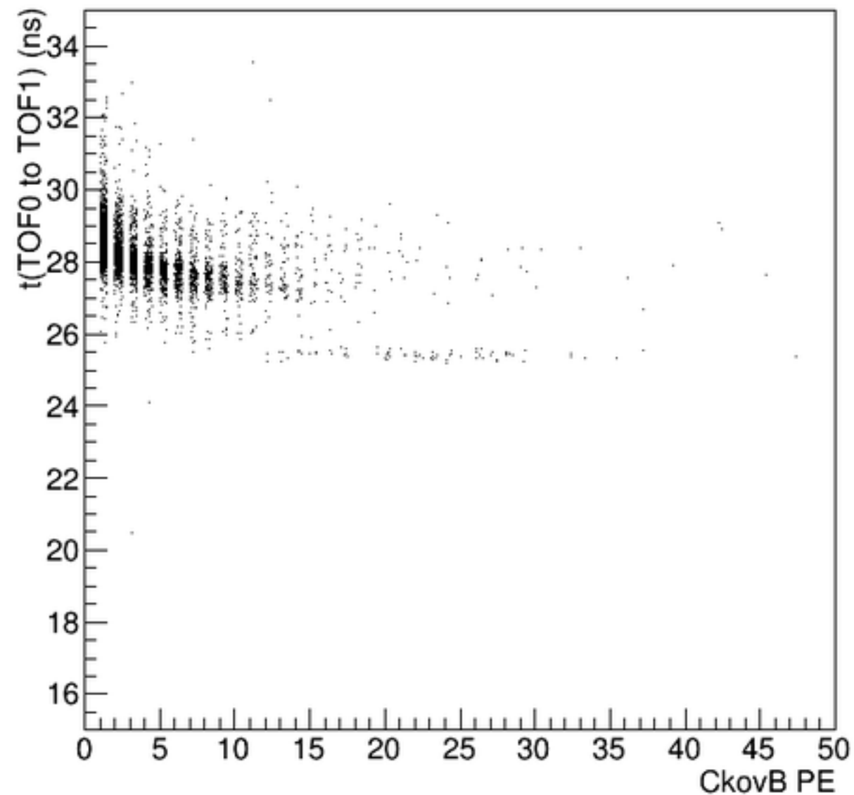
tof_B
