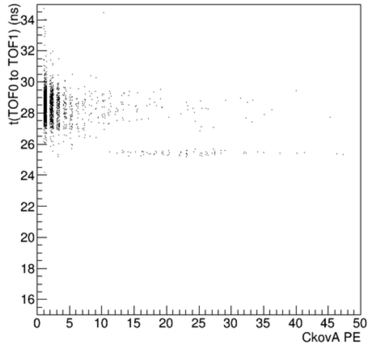
tof_A
