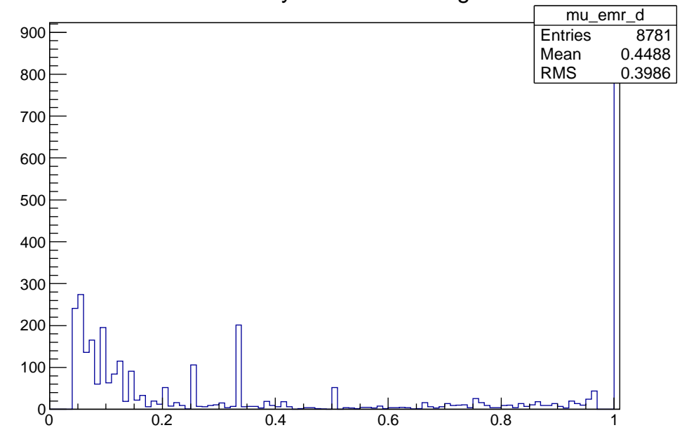
EMR Density after TOF+Range cut
