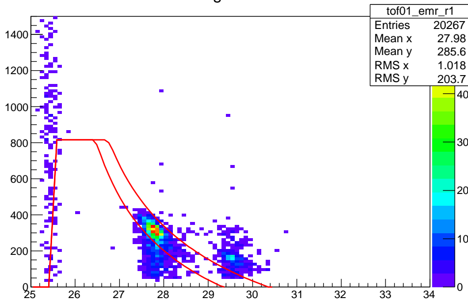
EMR Range 1 vs. TOF01
