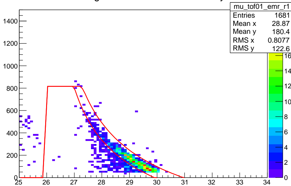
EMR Range 1 vs. TOF01 after Density cut
