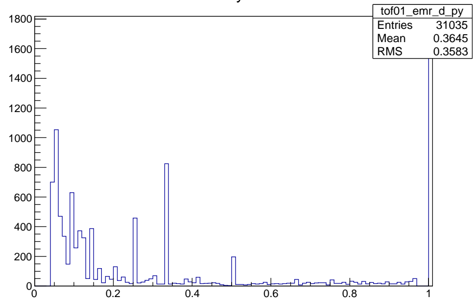
EMR Density vs. TOF01
