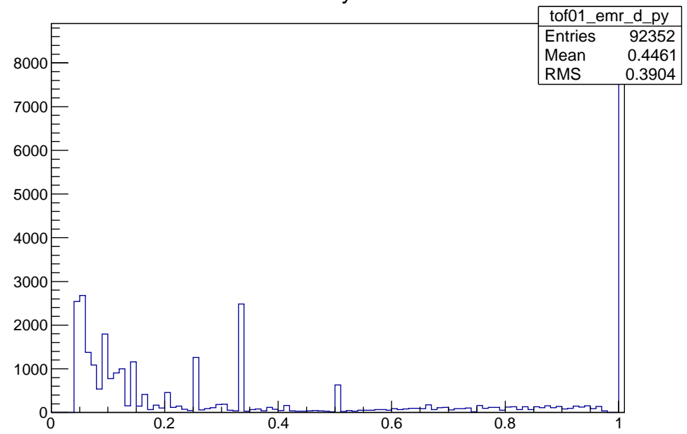
EMR Density vs. TOF01
