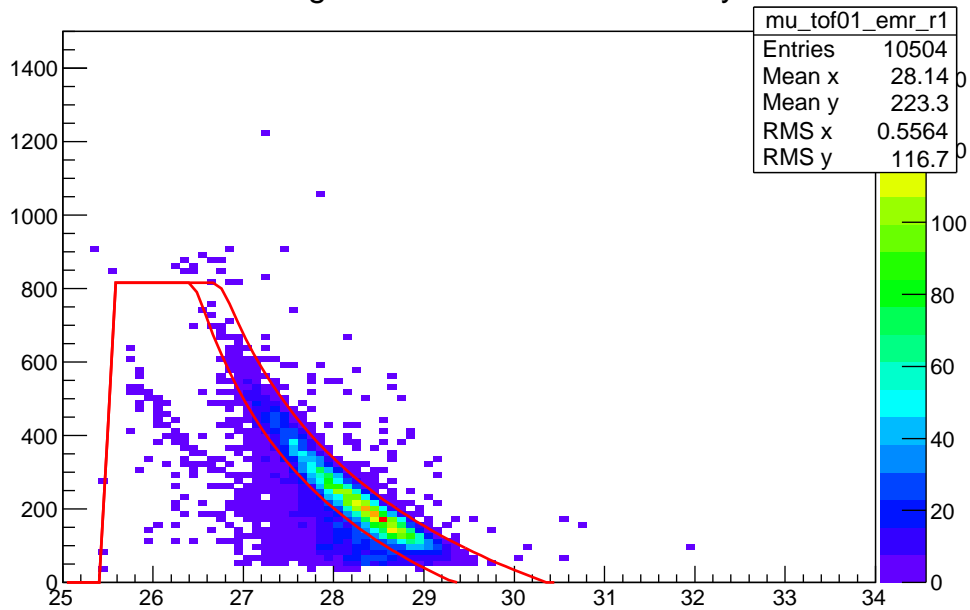
EMR Range 1 vs. TOF01 after Density cut
