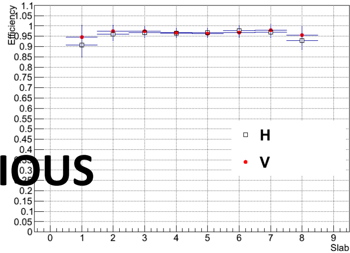
TOF2 Spacepoint Efficiency
