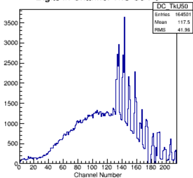
Digits in Channel TkU S5 P0
