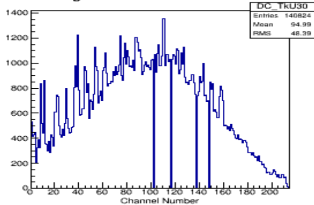
Digits in Channel TkU S3 P0
