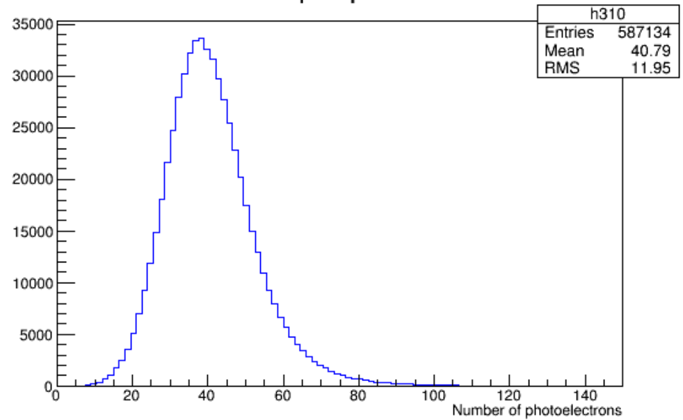
Seed Spacepoint NPE
