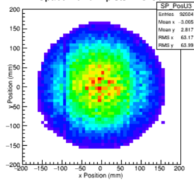
Space Point Triplets TKU S3
