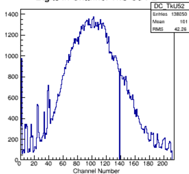
Digits in Channel TkU S5 P2
