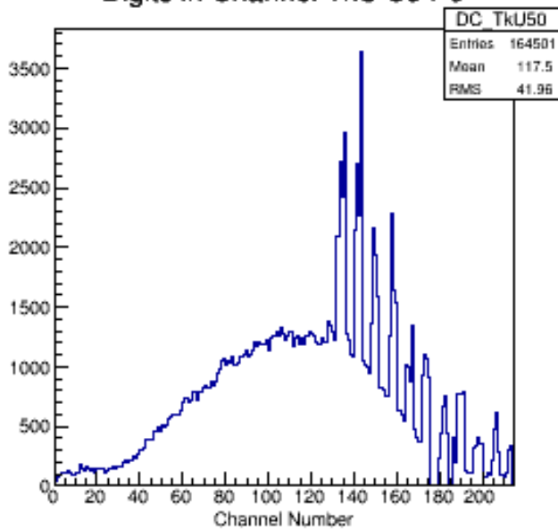
Digits in Channel TkU S5 P0
