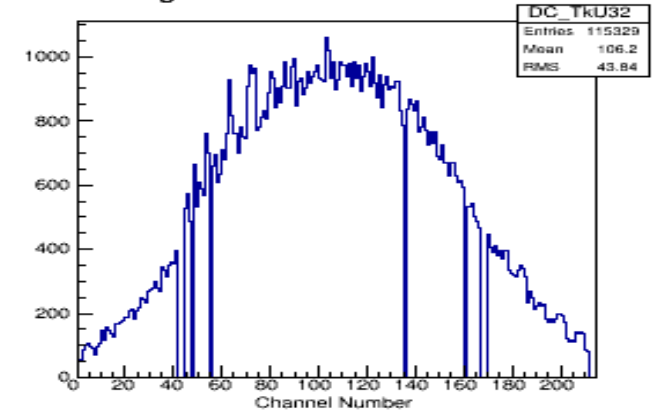
Digits in Channel TkU S3 P2
