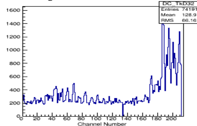
Digits in Channel Tkd S3 P2
