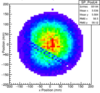
Space Point Triplets TKU S4
