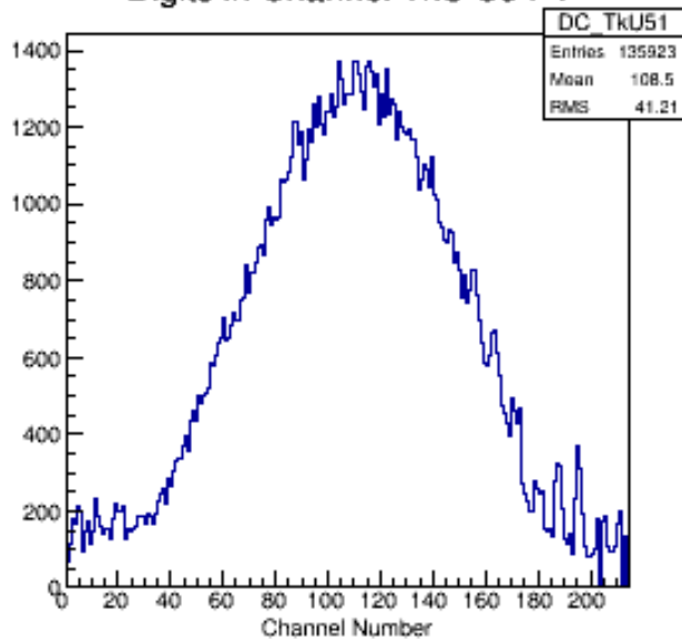
Digits in Channel TkU S5 P1
