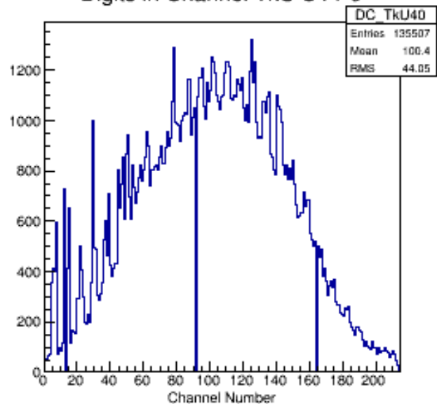
Digits in Channel TkU S4 P0
