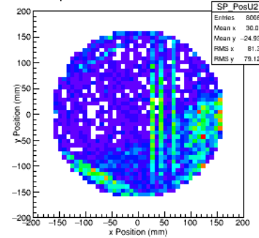
Space Point Doublets TKU S5
