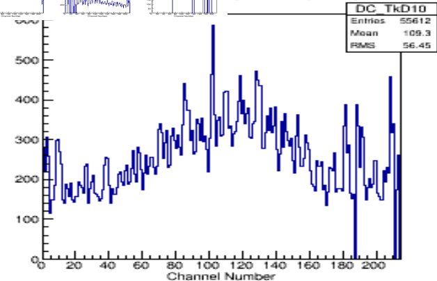
Digits in Channel Tkd S1 P0
