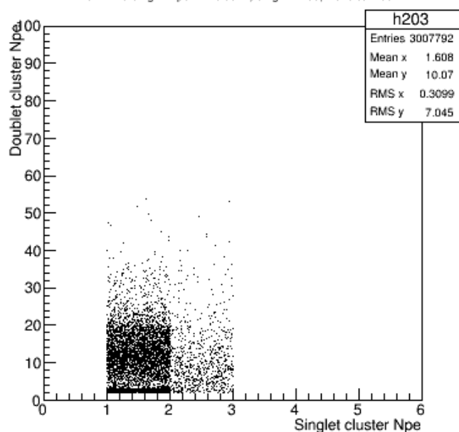
Doublet Vs Singlet Npe Per Cluster, Singlet=Blue, Doublet=Red
