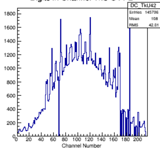
Digits in Channel TkU S4 P2
