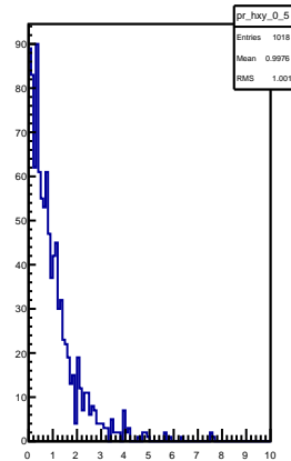
PatRec xy residuals T0 S5
