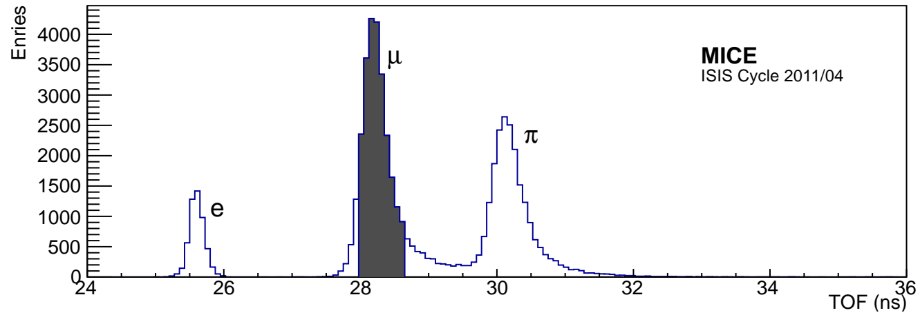
Particles TOF for P_{D_2} = 320 \text{ MeV/c}
