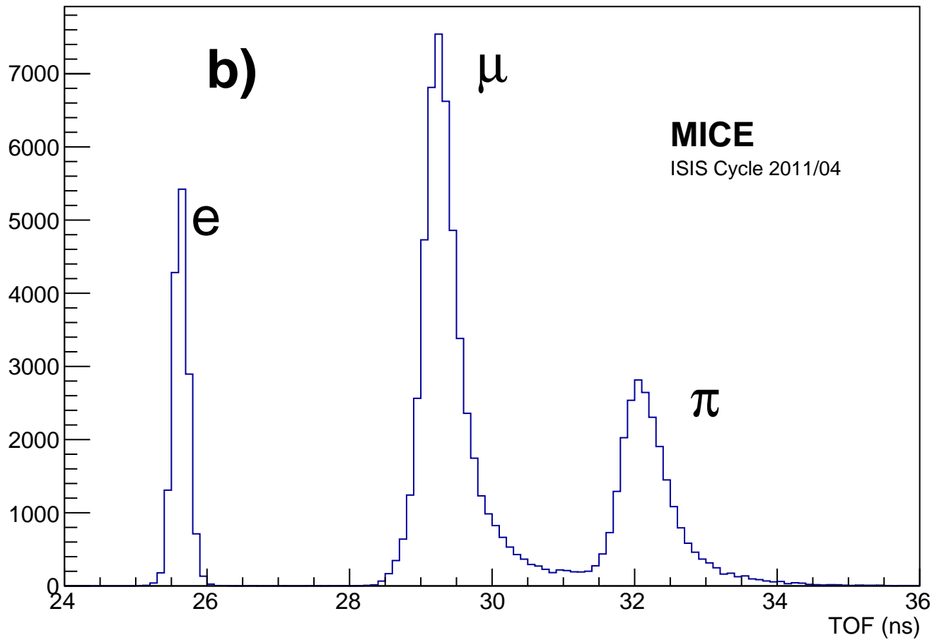
Time-of-flight distribution for beam momentum P_{D2} = 222 \text{ MeV}/c
