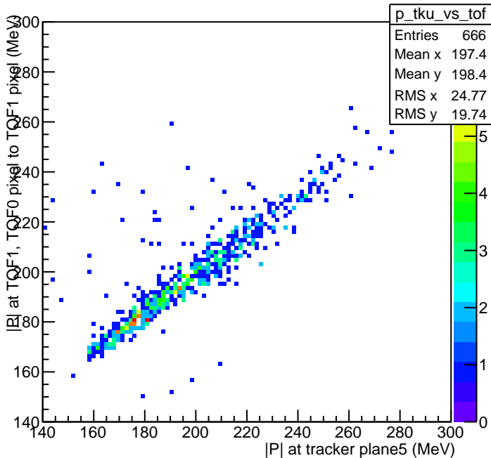
Tracker vs. TOF momentum (pixel calc)
