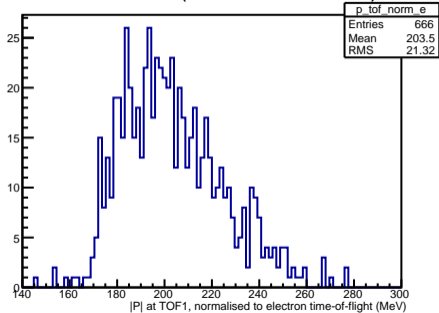
TOF momentum (normalised to electron tof)
