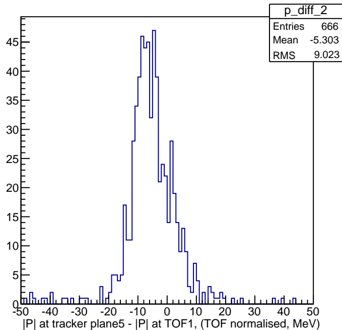
Tracker - TOF momentum (normalised method)
