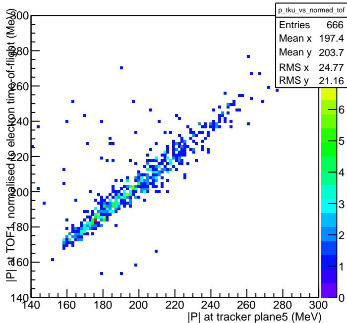
Tracker vs. TOF momentum (normalised calc)
