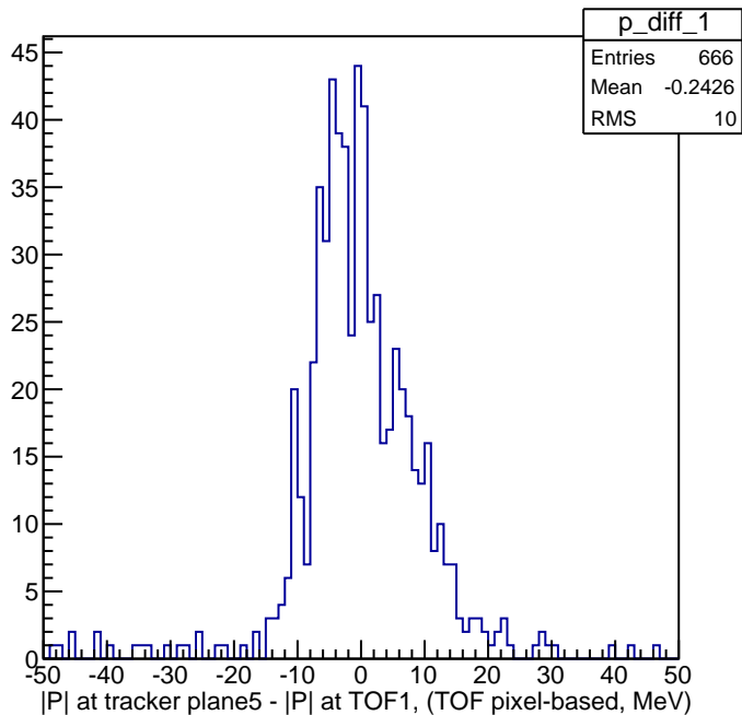
Tracker - TOF momentum (pixel method)
