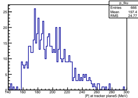
Momentum at tracker
