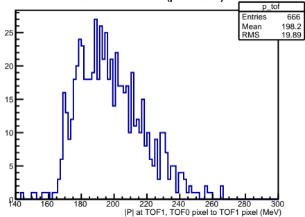
TOF momentum (pixel calc)
