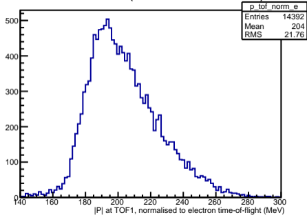
TOF momentum (normalised to electron tof)
