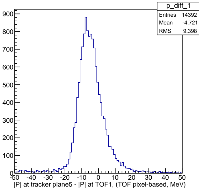
Tracker - TOF momentum (pixel method)
