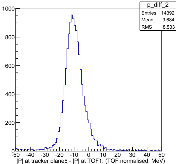
Tracker - TOF momentum (normalised method)
