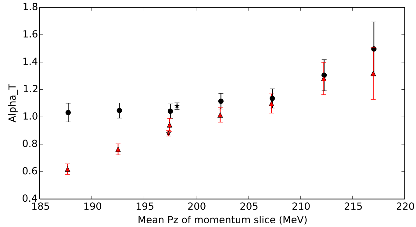
Selected particles at plane 5 and the reference plane, with mean p_z = 200 , \sigma_{p_z} = 10\text{MeV}
