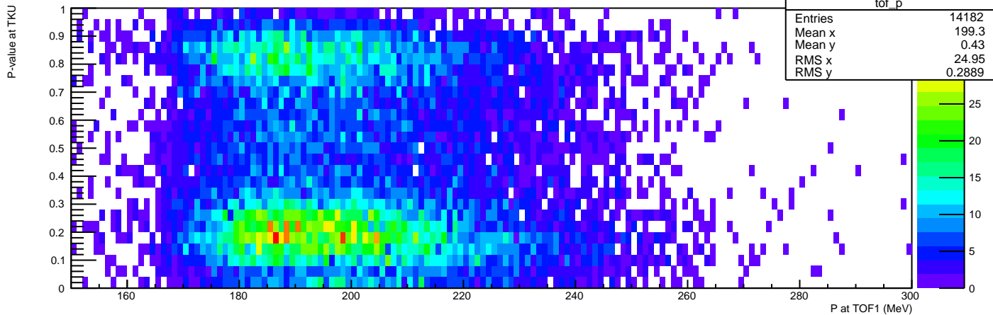
P-values wrt TOF momentum
