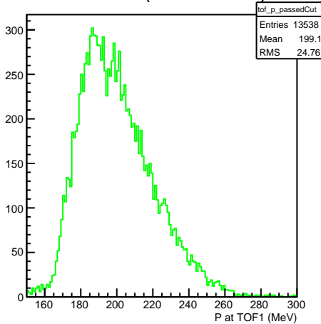
P at TOF1 (P-value &gt; 0.05)
