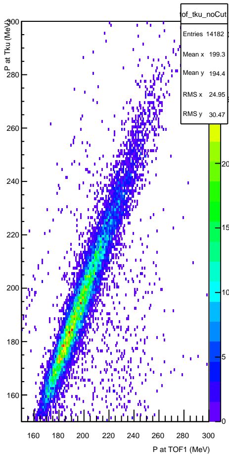
TOF P vs Tku P (No P-value cut)
