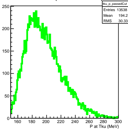
P at Tku (P-value &gt; 0.05)
