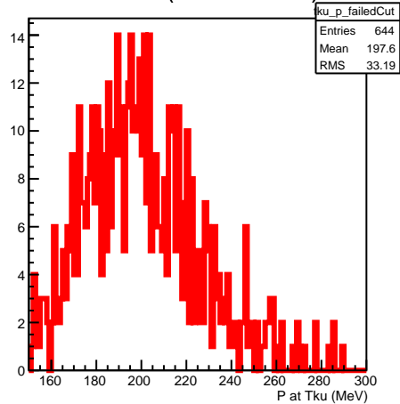
P at Tku (P-value &lt; 0.05)
