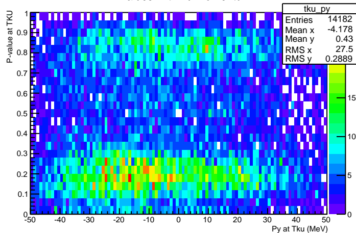
P-values wrt Tku momentum
