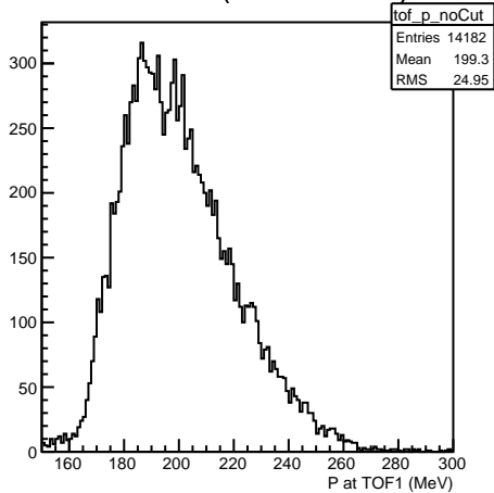
P at TOF1 (No P-value cut)
