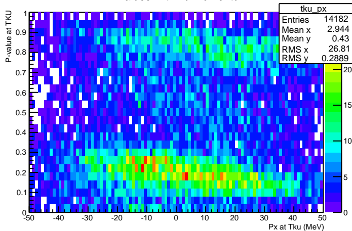
P-values wrt Tku momentum
