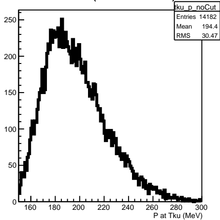
P at Tku (No P-value cut)
