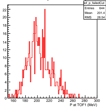
P at TOF1 (P-value &lt; 0.05)
