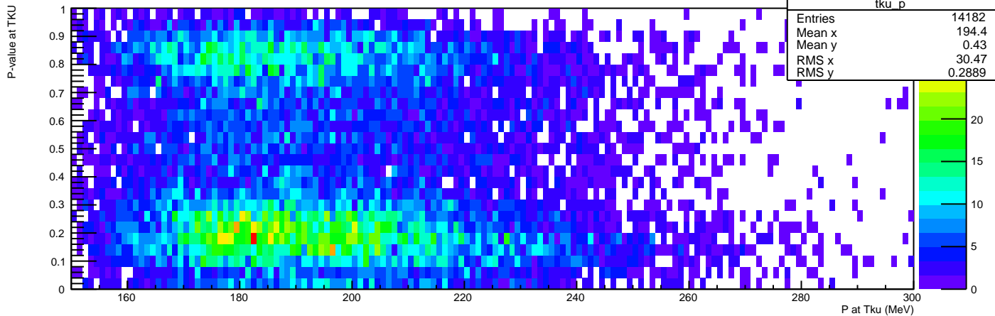
P-values wrt Tku momentum
