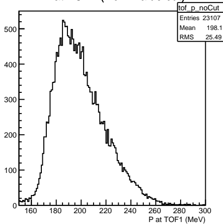
P at TOF1 (No P-value cut)
