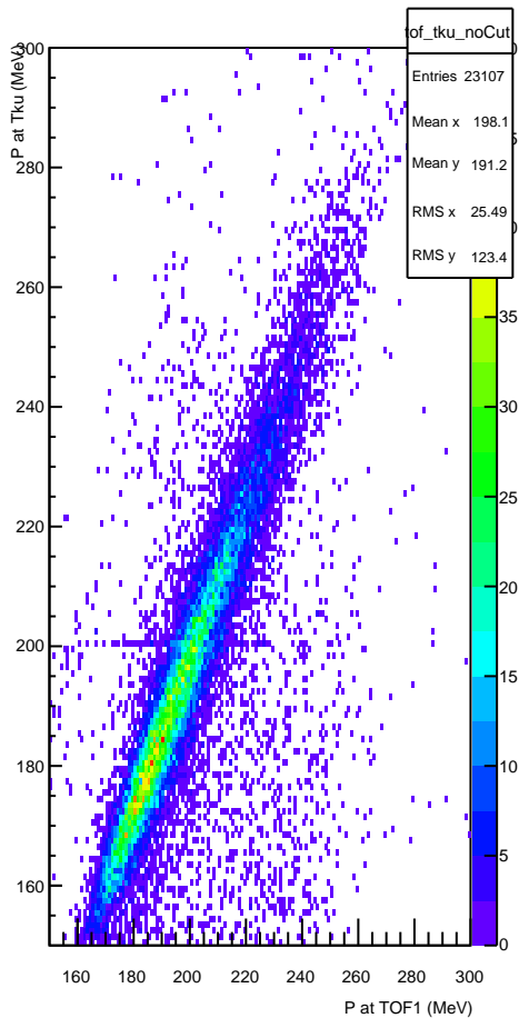
TOF P vs Tku P (No P-value cut)
