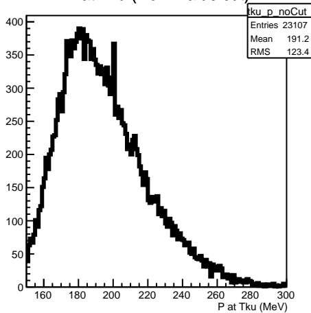
P at Tku (No P-value cut)
