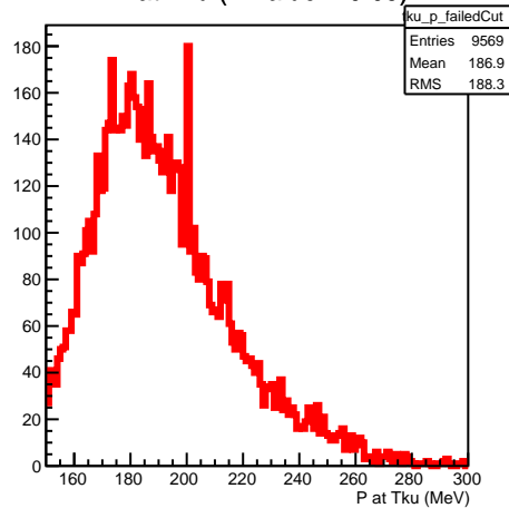
P at Tku (P-value &lt; 0.05)
