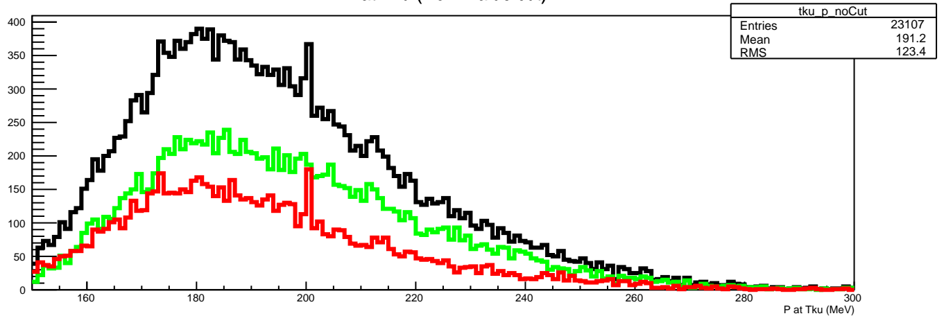
P at Tku (No P-value cut)
