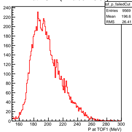
P at TOF1 (P-value &lt; 0.05)
