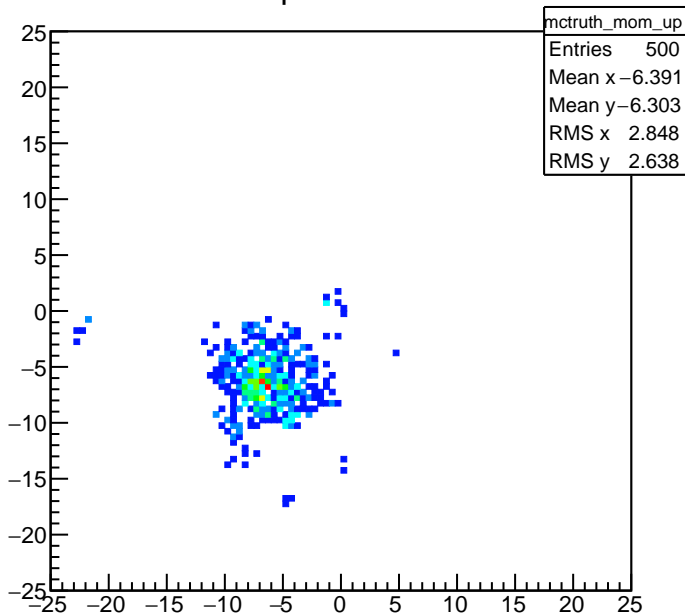
MC Truth Upstream Momentum
