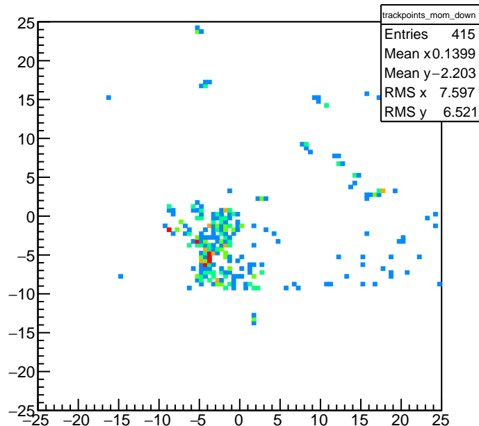
Track Point Downstream Momentum
