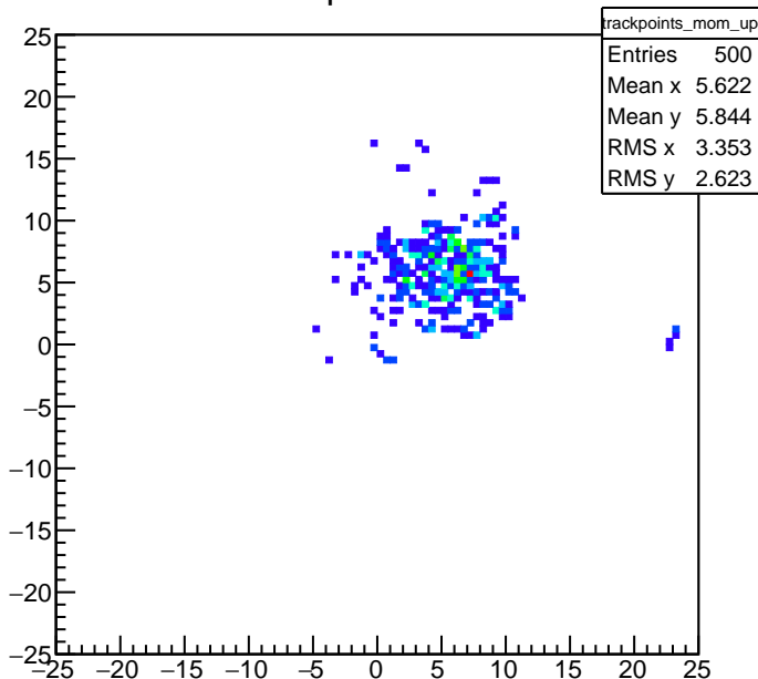
Track Point Upstream Momentum
