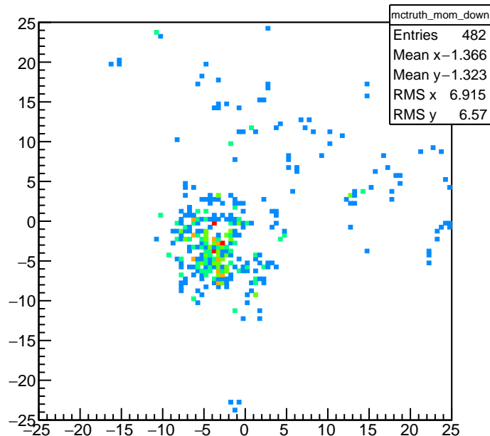
MC Truth Downstream Momentum
