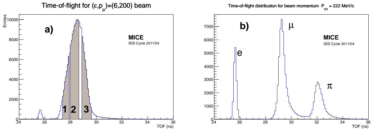
Figure 3: (a) Time of flight distributions between TOF0 and TOF1 for a positive muon beam with a nominal momentum of 200 \text{ MeV}/c (the left peak is due to electrons). The labels 1, 2 and 3 in the muon peak refer to the three time-of-flight intervals, highlighted in grey, used in the analysis. (b) Positive “calibration” beam taken with p_{D2} = 222 \text{ MeV}/c , showing clear electron, muon and pion peaks.
