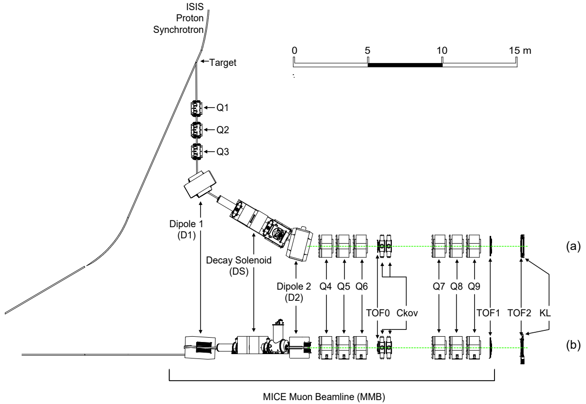
Figure 2: Top view of the MICE Muon Beam and its instrumentation for the pion contamination measurement.
