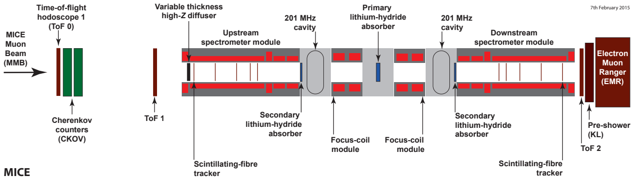
Figure 1: Schematic view of the MICE experiment, with three LiH absorbers (one primary absorber in the centre and two secondary absorbers), two RF cavities and two Focus Coil solenoid magnets that define the MICE optics, sandwiched between two identical trackers, inside superconducting solenoids.
