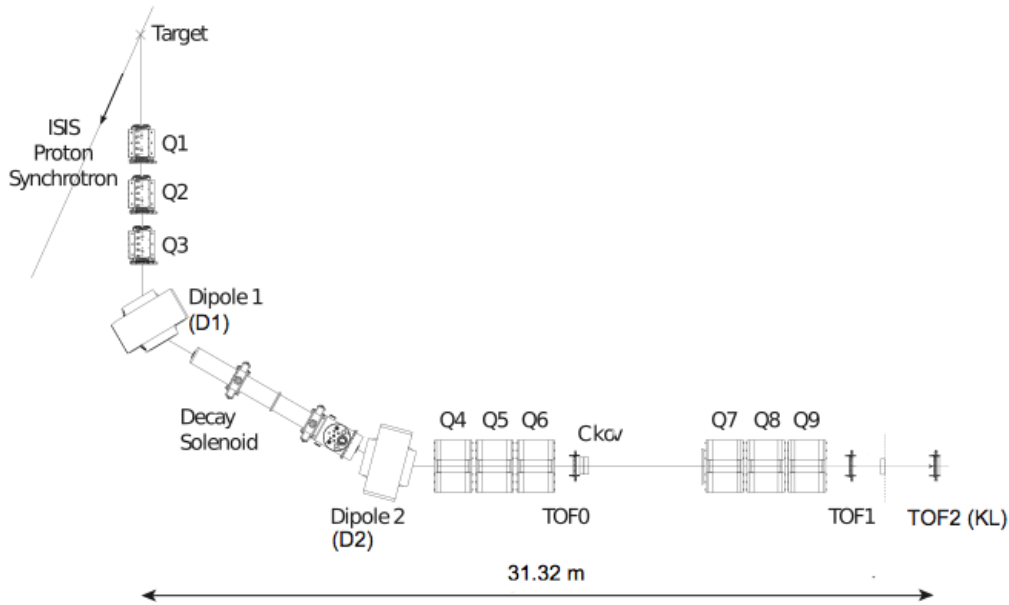
Figure 2: Top view of the MICE Muon Beam and its instrumentation for the pion contamination measurement.
