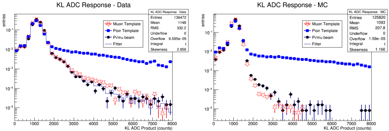
Figure 13: Left: Muon template (red stars) and pion template (blue squares) for the sum of the three TOF data intervals from calibration runs, compared to MICE \pi \rightarrow \mu beam data (black dots) using the cut of number of KL hits > 0 . Right: Monte Carlo simulation of the muon template (red stars) and pion template (blue squares) for the sum of the three TOF data intervals, compared to the simulated MICE \pi \rightarrow \mu beam data (black dots). The histograms are the result of the fits of the \pi \rightarrow \mu beam to the fraction of pions and muons based on the two templates. Plots are normalised to unity.
