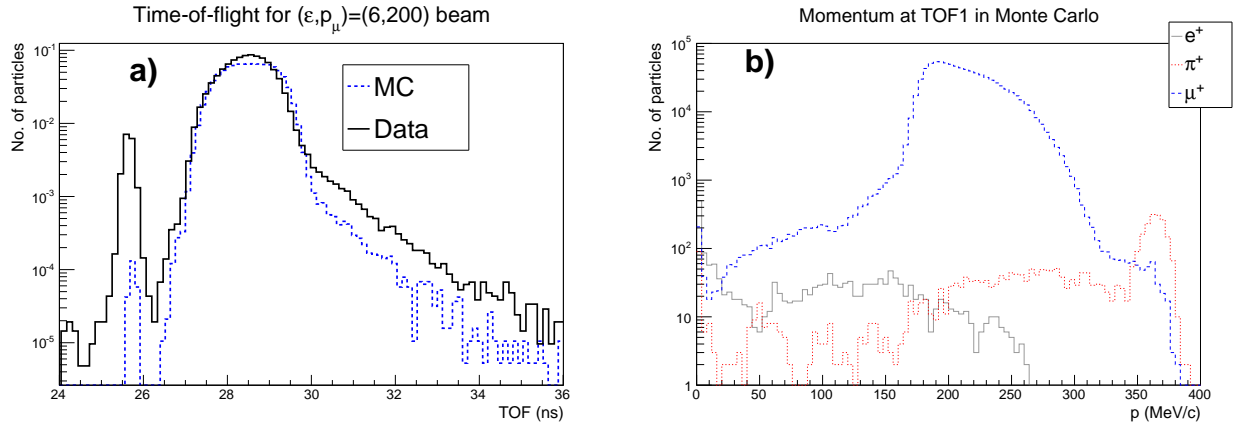
Figure 3: a) Time-of-flight distributions between TOF0 and TOF1 for data and Monte Carlo simulation for a 6\pi mm · rad positive muon beam with nominal beam momentum p_\mu = 200 MeV/c. b) Momentum distribution for beam particles at TOF1 for a simulated positive 6\pi mm · rad beam at 200 MeV/c (the time-of-flight between TOF0 and TOF1 is required to satisfy 26.2 < \text{TOF} < 32 ns).
