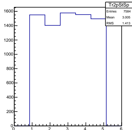
Space Points (3 Clusters) in Tracker2 per Station
