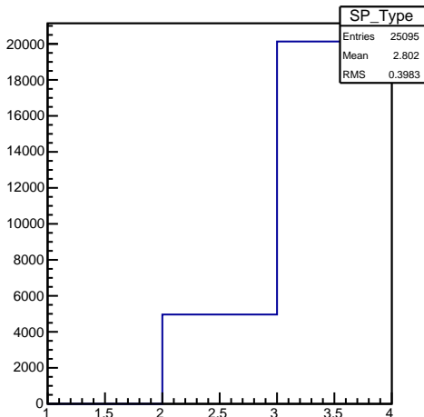
Space Point Type Across All Stations
