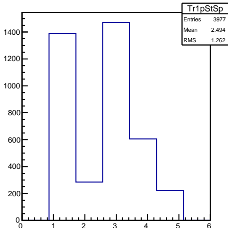
Space Points (2 Clusters) in Tracker2 per Station
