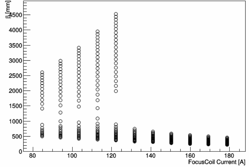
Momentum=200.0 MeV/c
