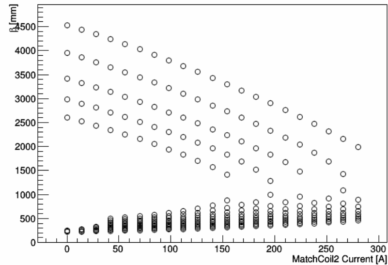
Momentum=200.0 MeV/c
