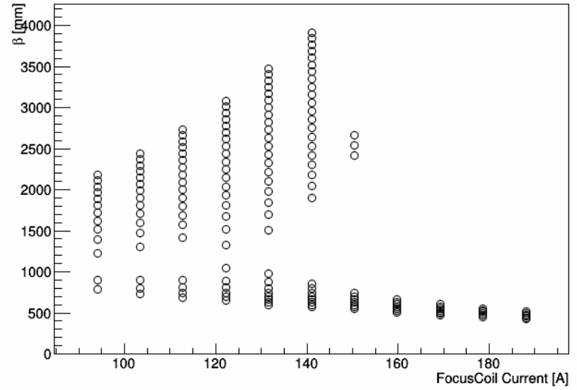
Momentum=240.0 MeV/c
