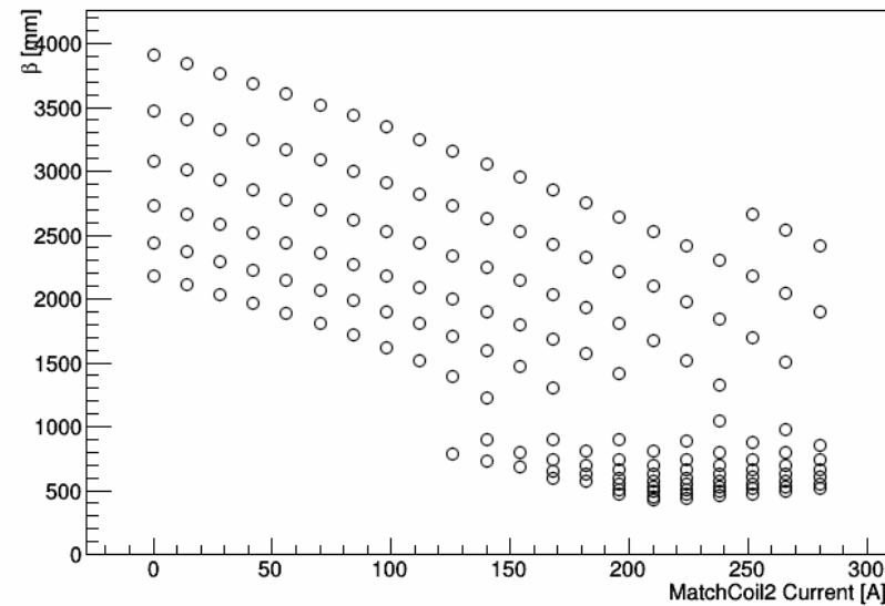
Momentum=240.0 MeV/c
