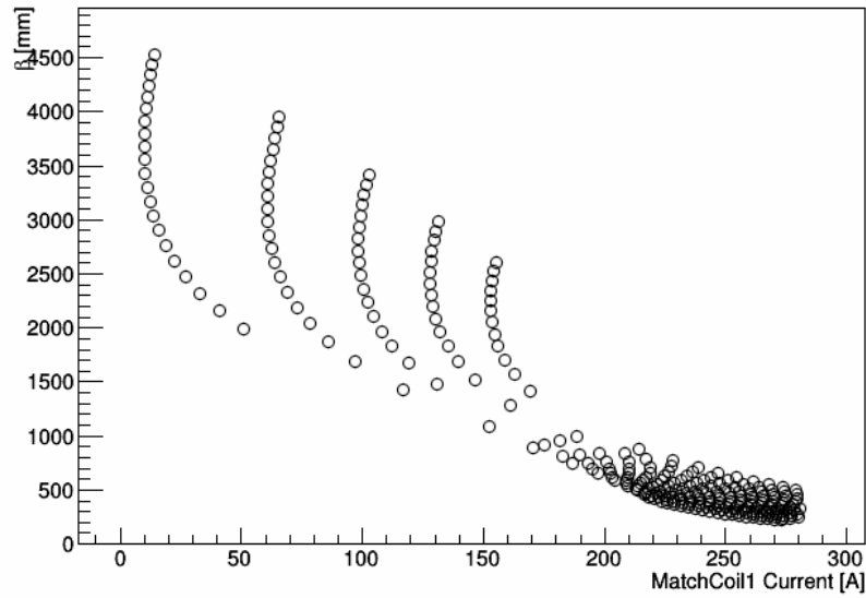
Momentum=200.0 MeV/c
