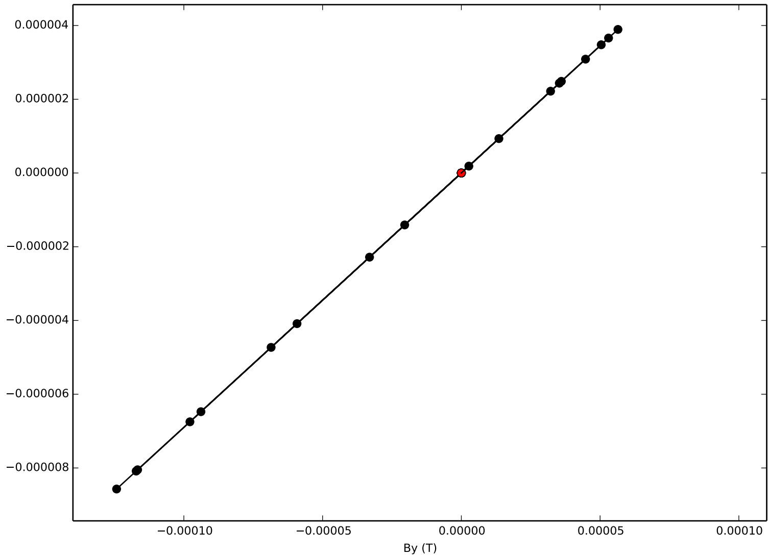
Residual vectors over all z
