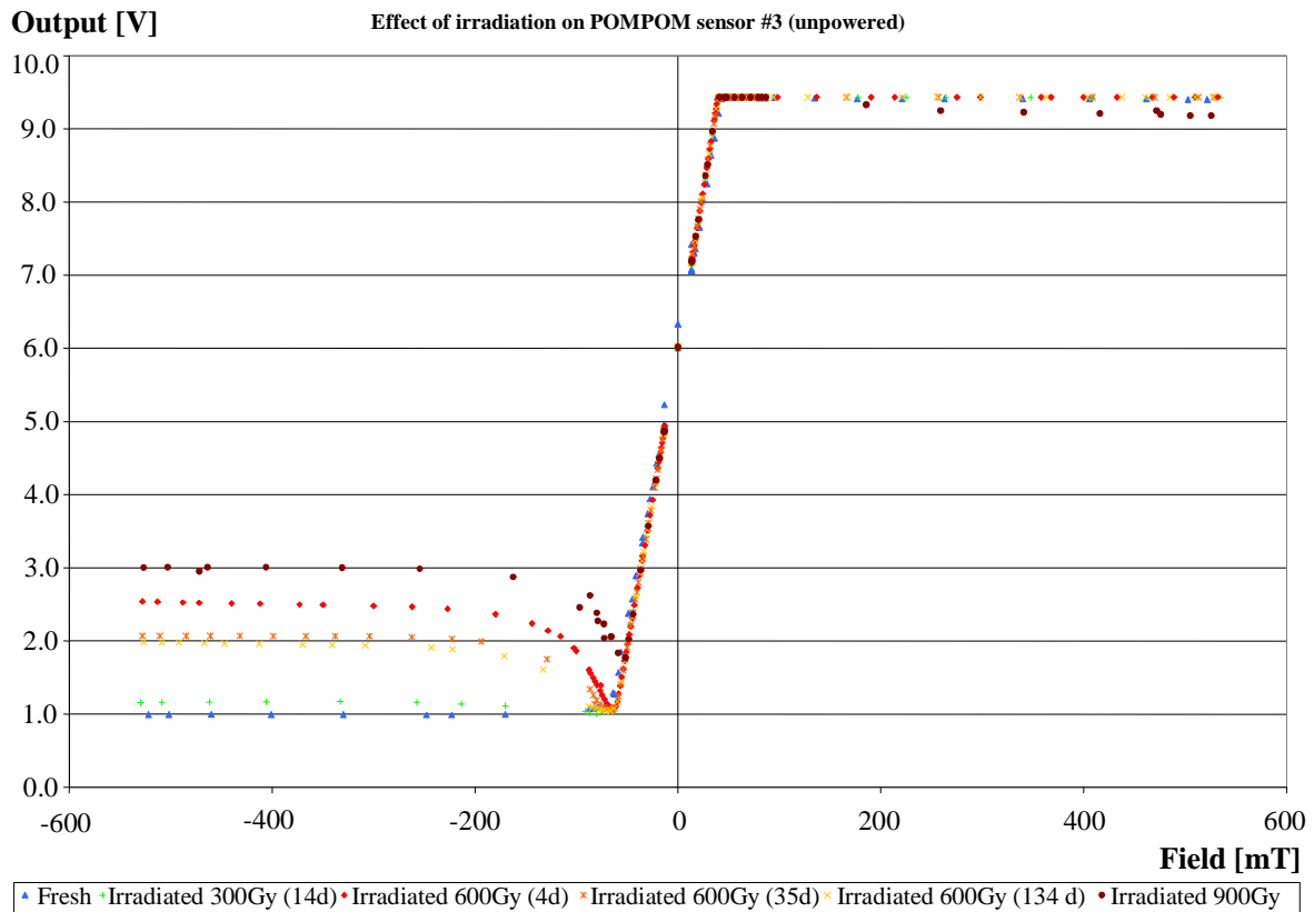
Figure 3: Effect of successive 300 Gy irradiations ( ^{60}\text{Co} ) on sensor #3. Intervals between exposure and measurement are given in days, where relevant. The immediate effects of the second dose (to 600 Gy) abate within a few weeks, but the remaining damage lasts for months. The final (900 Gy) results were taken just a few hours after the irradiation; the scatter is from the real changes in device response with time as it recovers.
