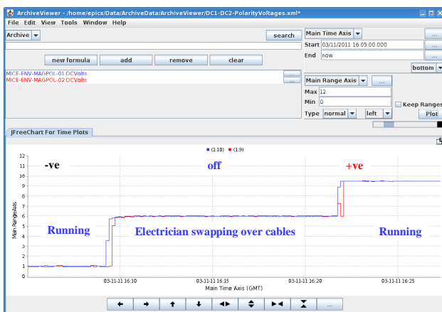
Figure 4: Stripchart showing POMPOM raw outputs during a changeover of supply polarity.
