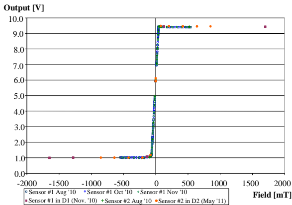
Figure 1: Sensor response in lab tests and in beamline. The error bars are smaller than the symbols at this scale.
