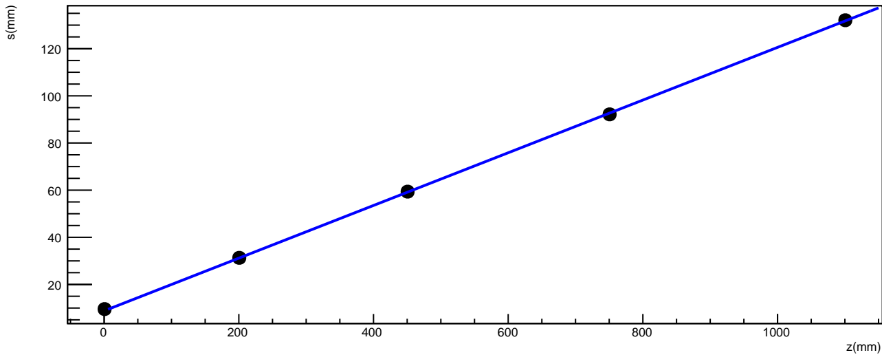
Seed s-z plot for tracker 2
