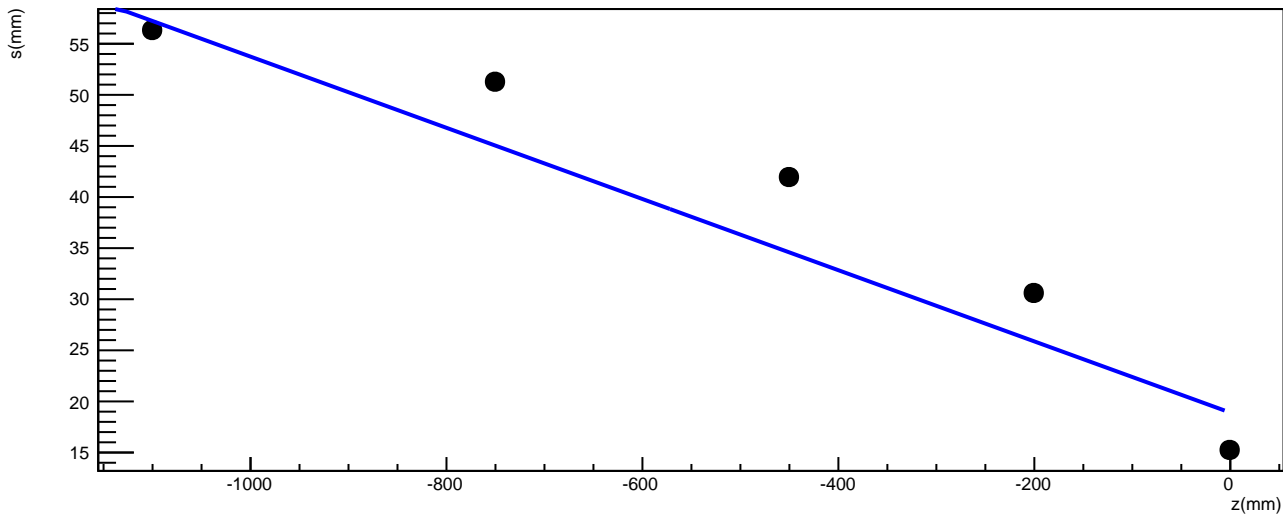
Seed s-z plot for tracker 1
