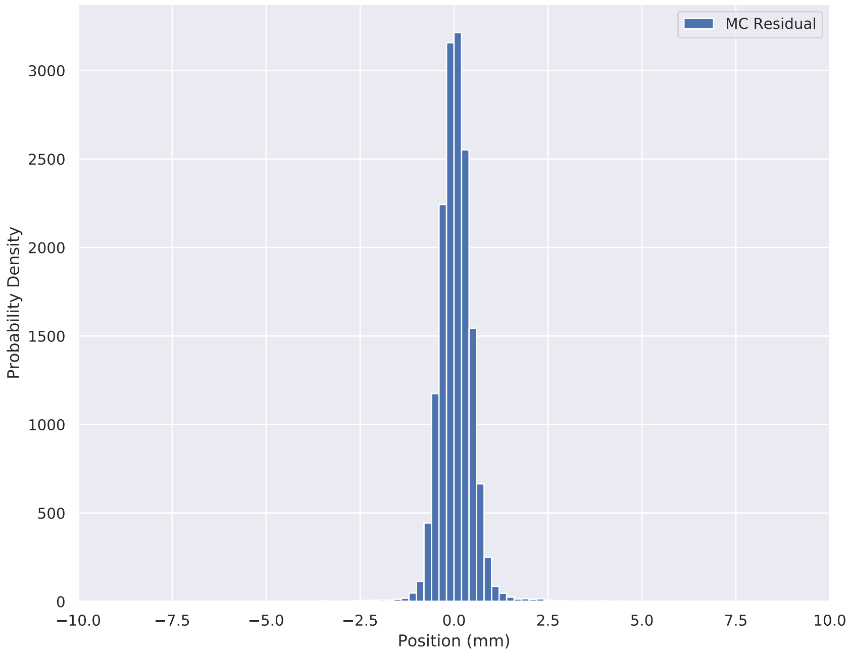
6-140 Wedge Solenoid X Residual (Full Upstream) TKU S2
