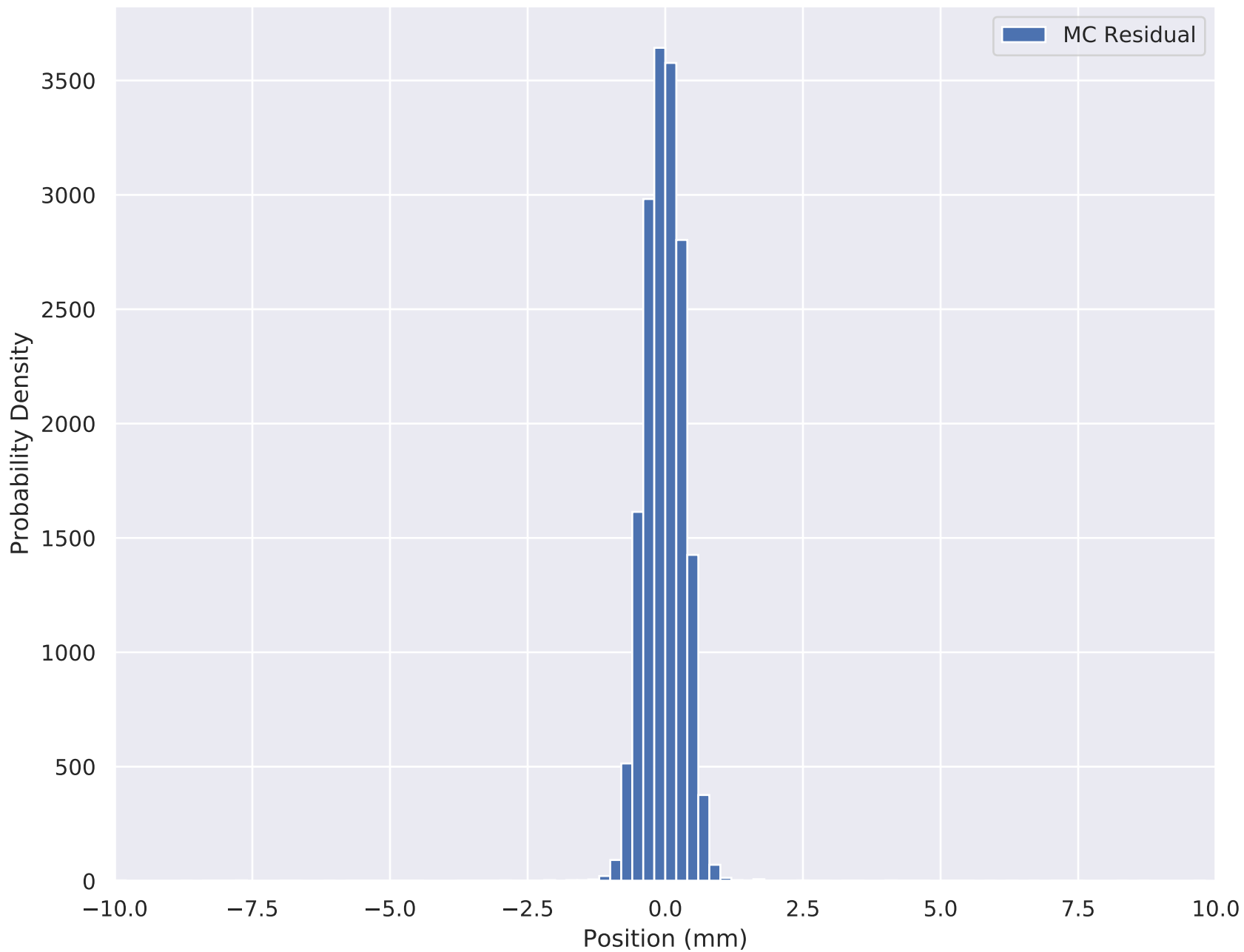
6-140 Wedge Solenoid X Residual (Full Upstream) TKU S5
