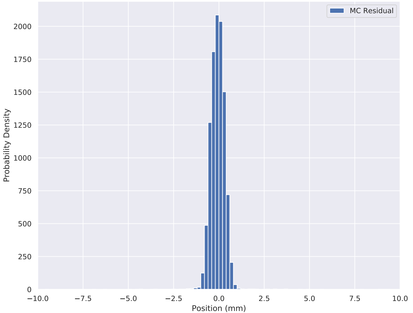
6-140 Wedge Solenoid X Residual (TOF2 cut) TKU S1
