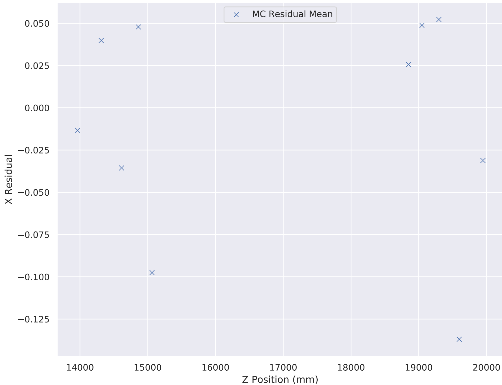
6-140 Wedge Solenoid X Residual Mean (TOF2 cut)
