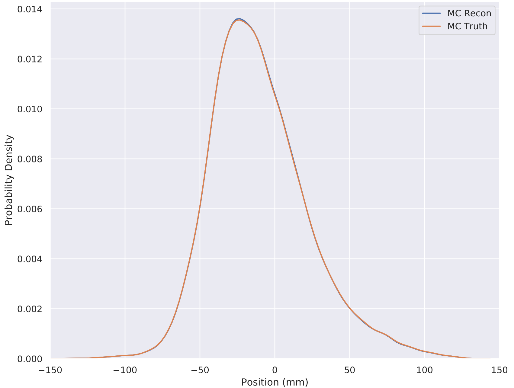
6-140 Wedge Solenoid X Position (TOF2 cut) TKD S2
