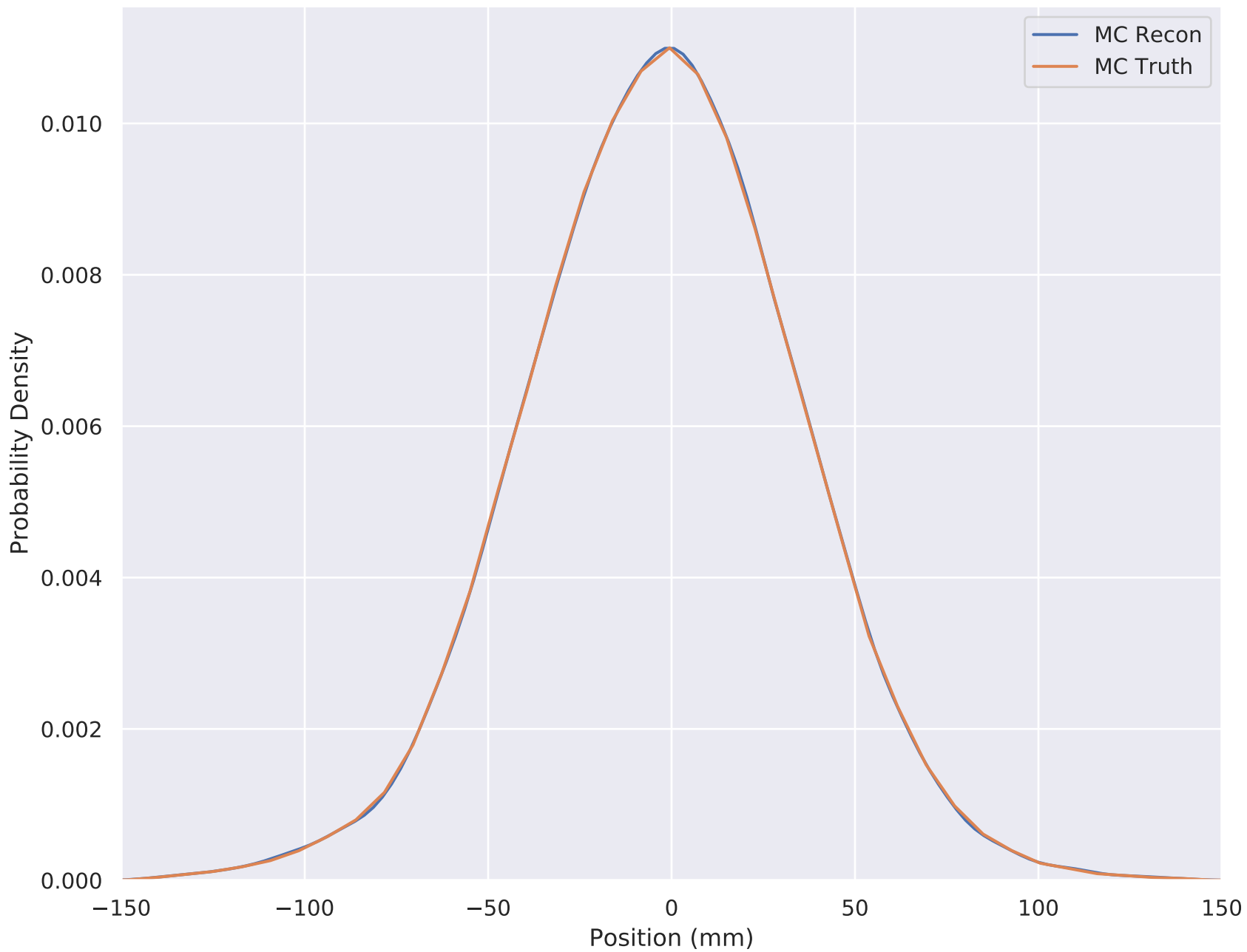
6-140 Wedge Solenoid X Position (Full Upstream) TKU S1
