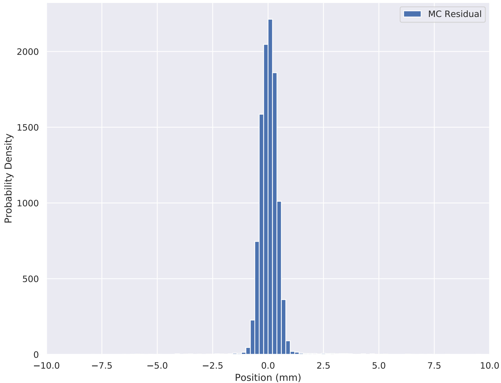
6-140 Wedge Solenoid X Residual (TOF2 cut) TKU S4
