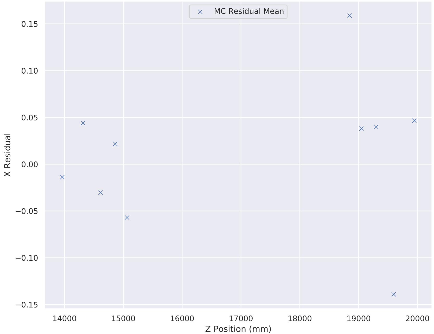
6-140 Wedge Solenoid X Residual Mean (Downstream cut)
