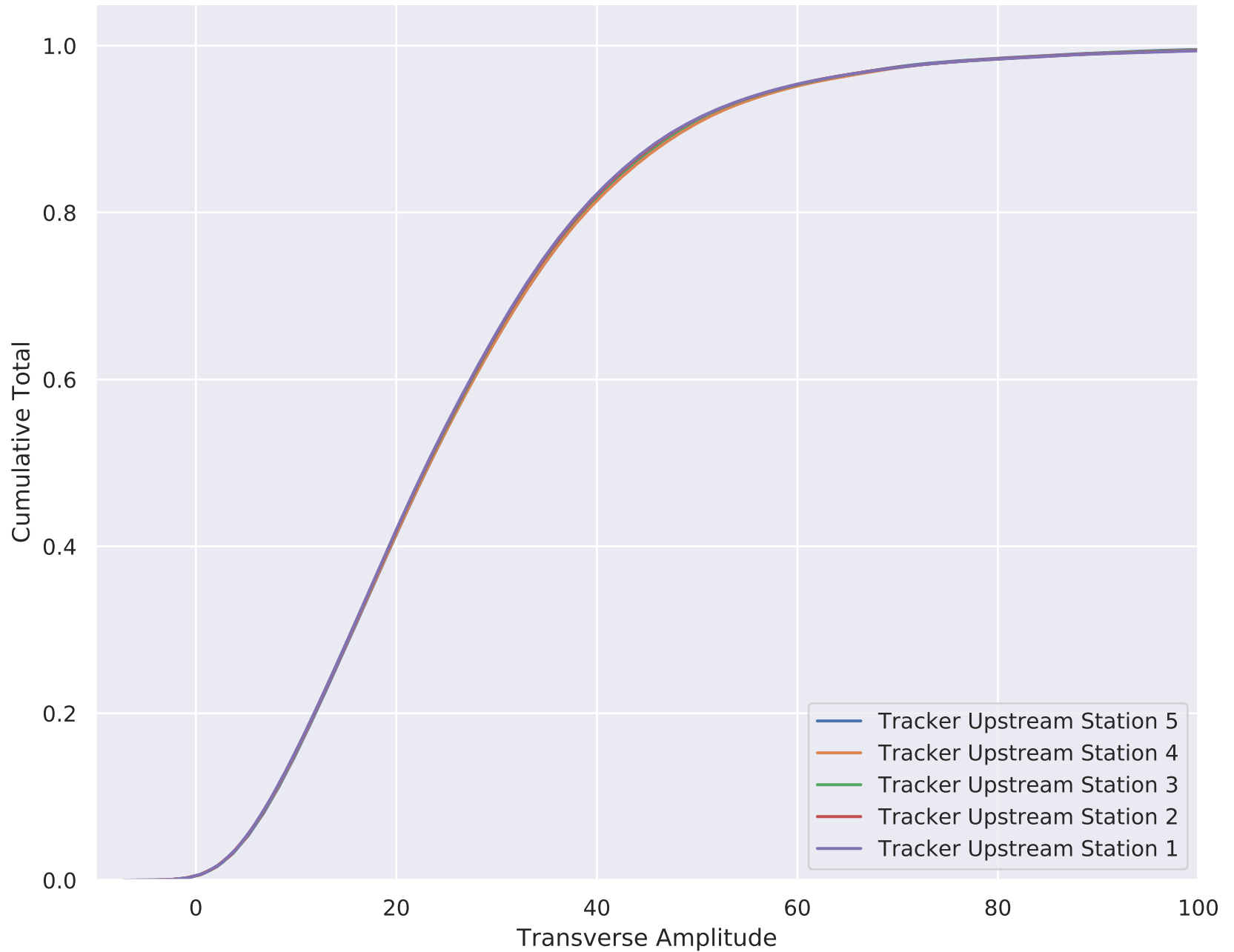
6-140 Wedge Solenoid Amplitude MC Recon (Full Upstream)
