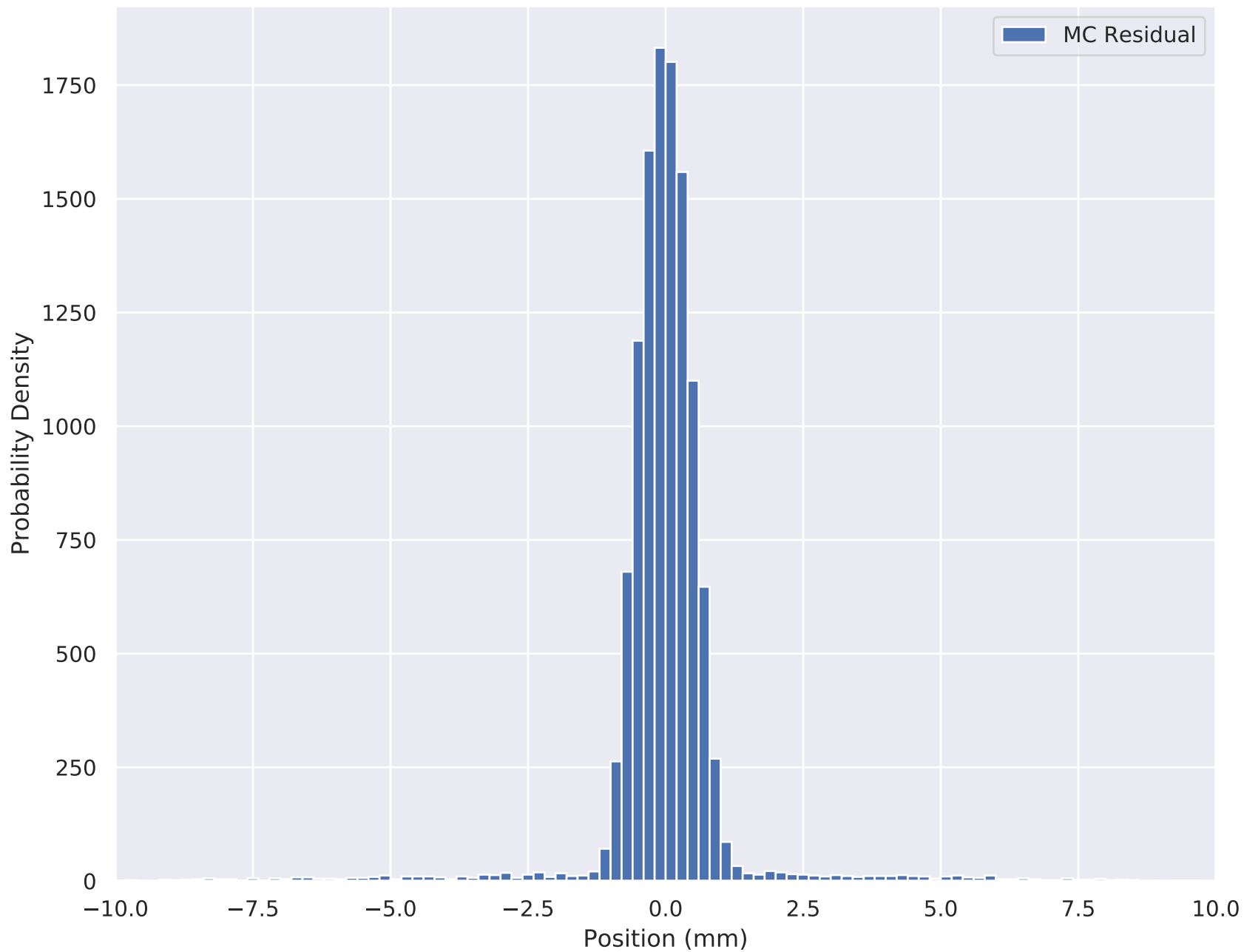
6-140 Wedge Solenoid X Residual (Downstream cut) TKD S5
