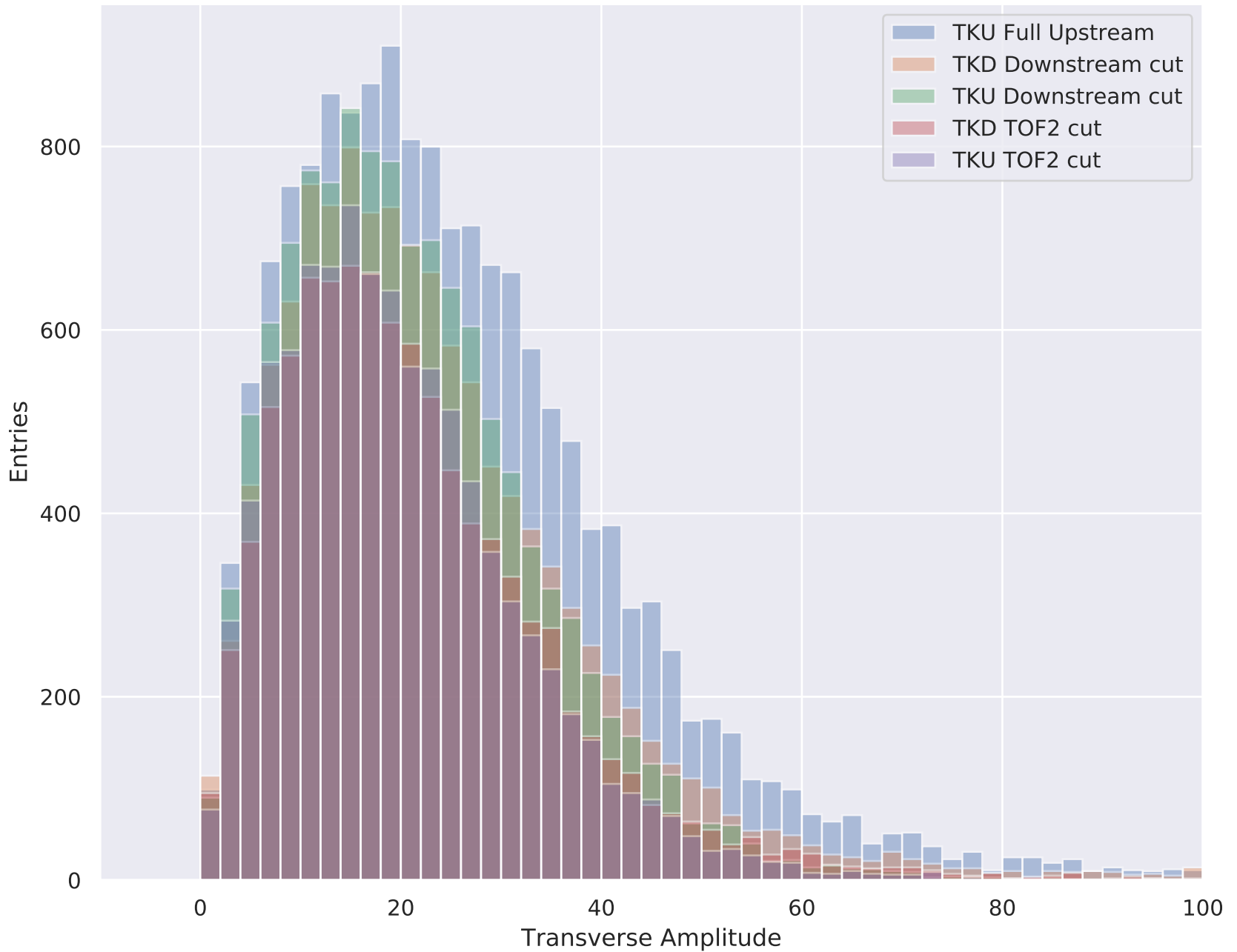
6-140 Wedge Solenoid Amplitudes MC Recon
