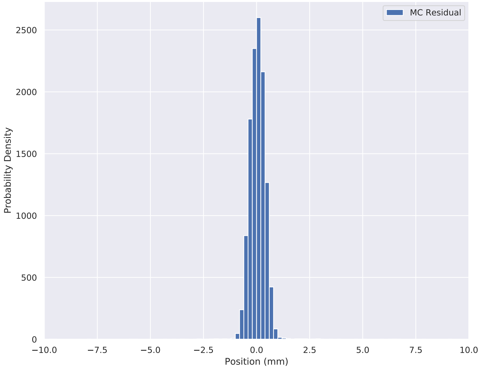
6-140 Wedge Solenoid X Residual (Downstream cut) TKU S4
