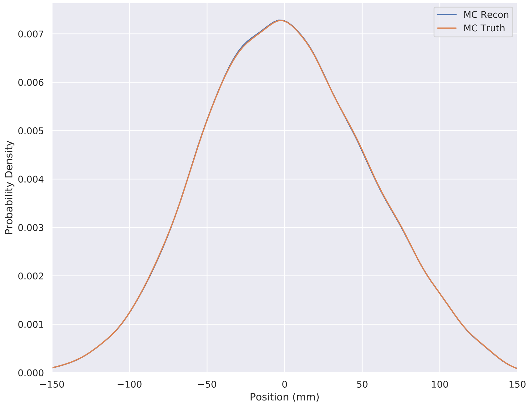
6-140 Wedge Solenoid X Position (Downstream cut) TKD S3
