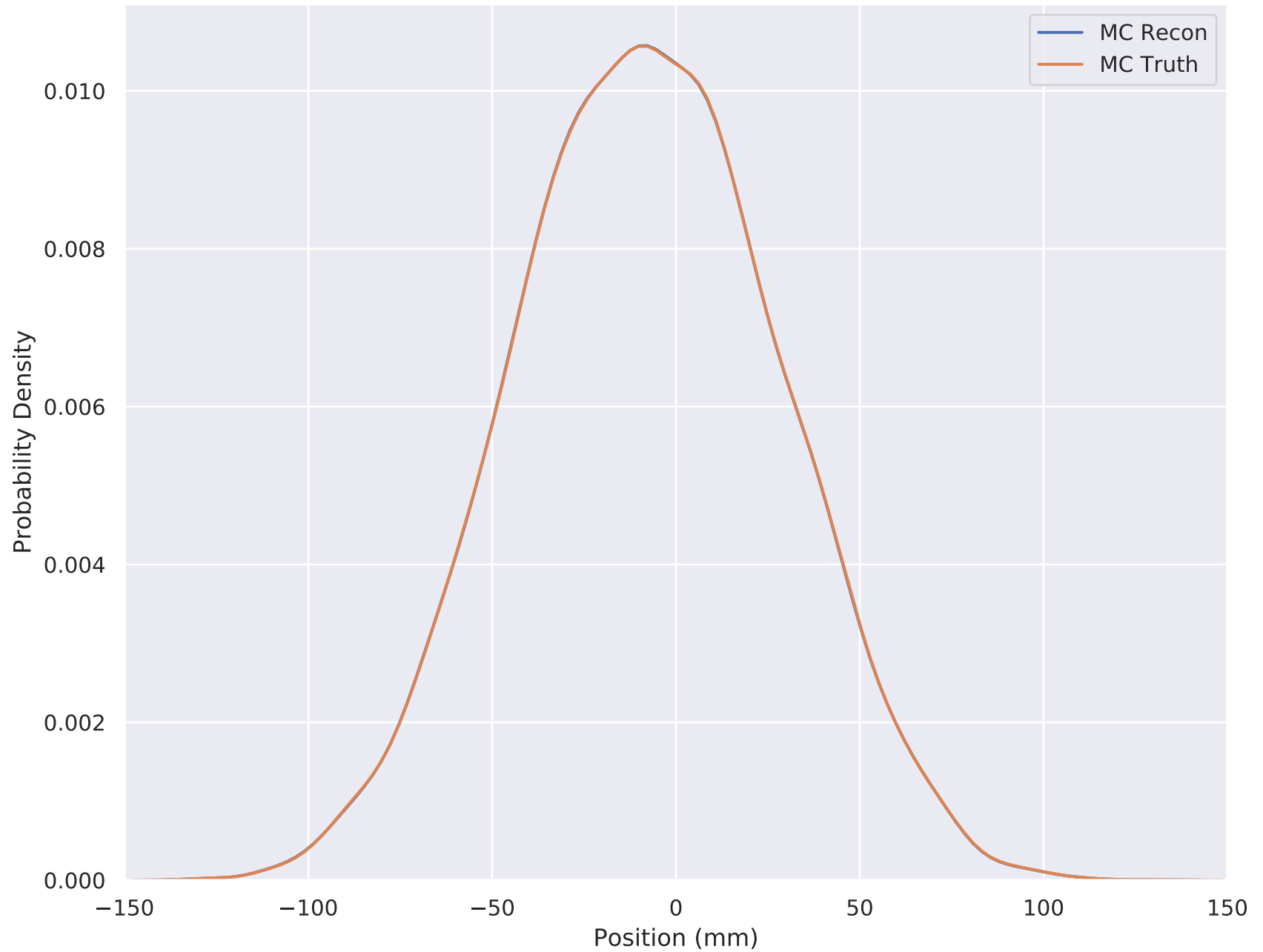
6-140 Wedge Solenoid X Position (Downstream cut) TKU S4
