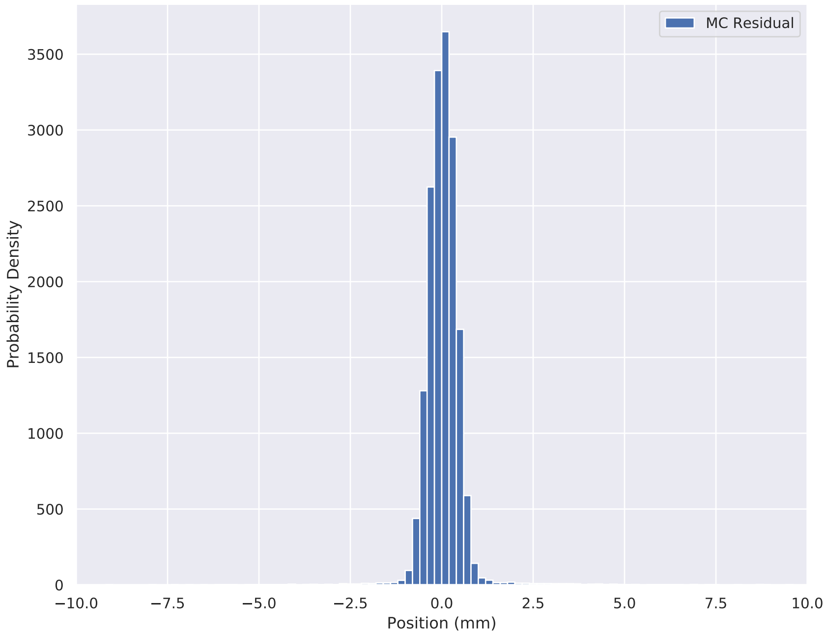
6-140 Wedge Solenoid X Residual (Full Upstream) TKU S4
