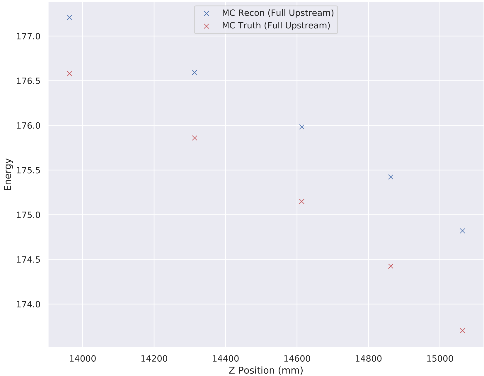
6-140 Wedge Solenoid Energy (Full Upstream)
