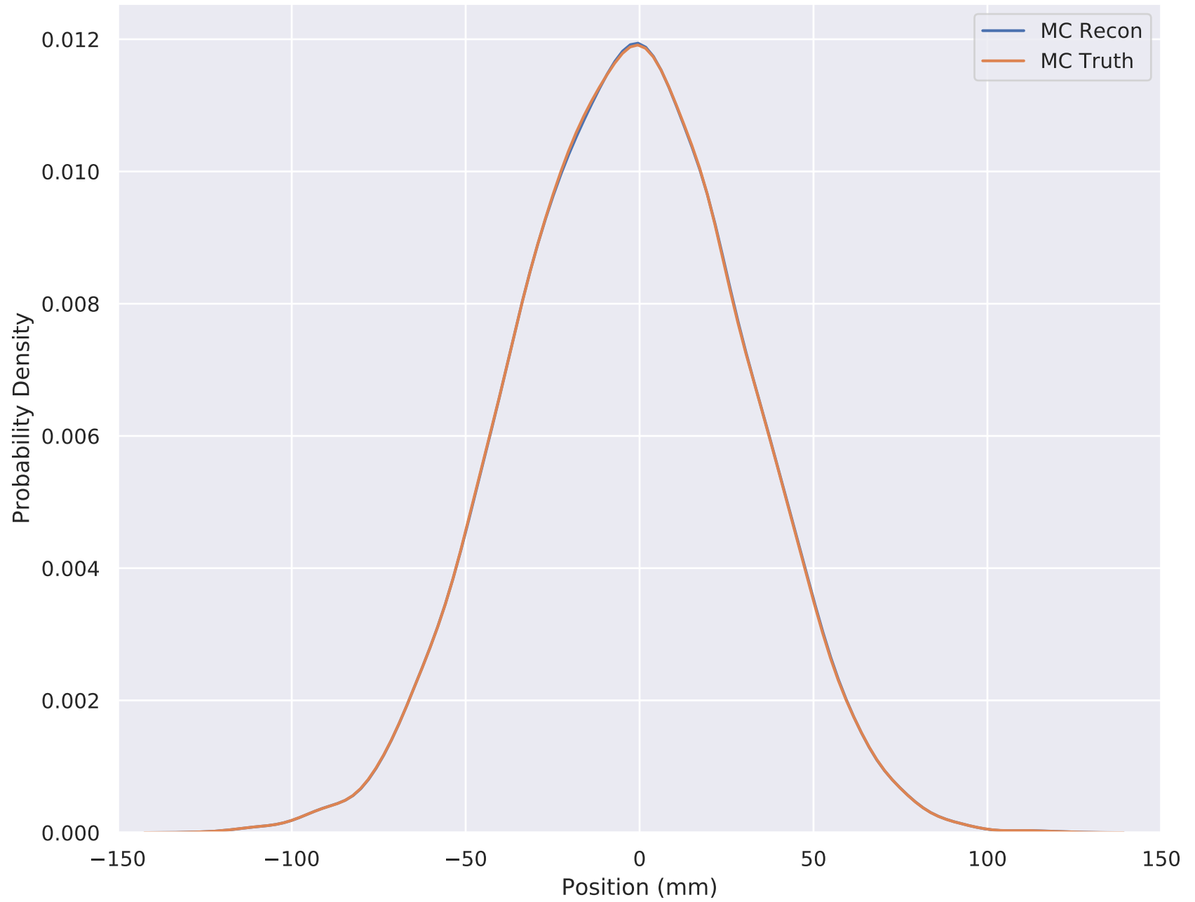
6-140 Wedge Solenoid X Position (Downstream cut) TKU S1
