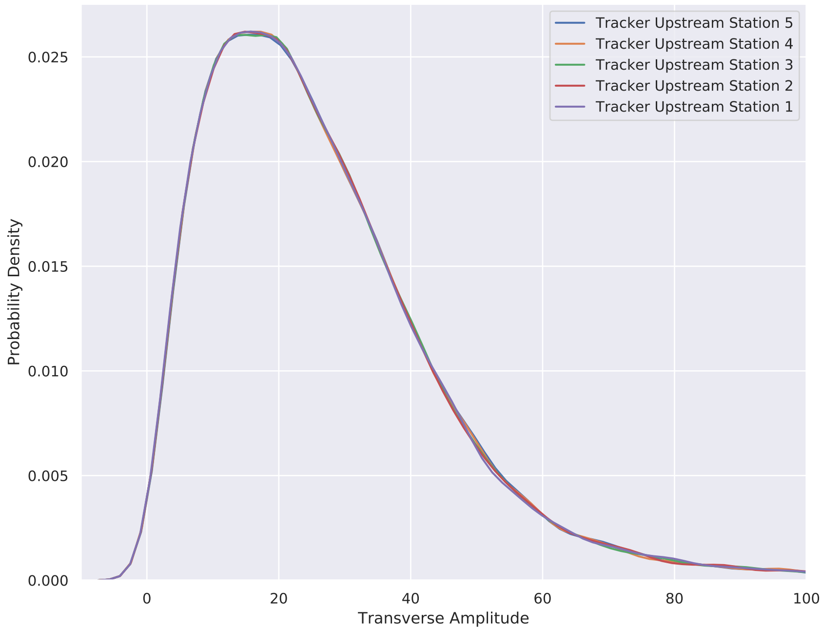
6-140 Wedge Solenoid Amplitude MC Recon (Full Upstream)
