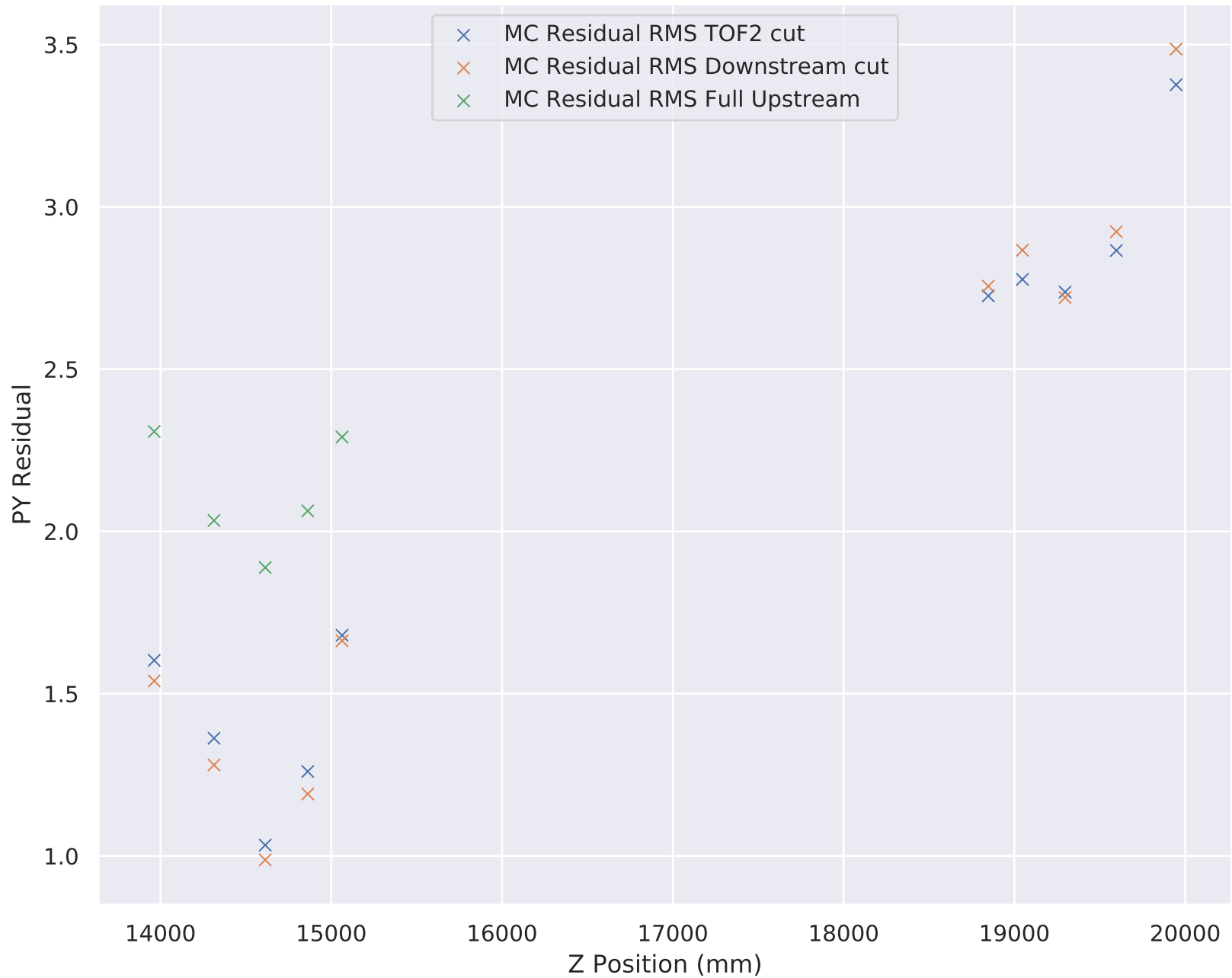
6-140 Wedge Solenoid PY Residual RMS
