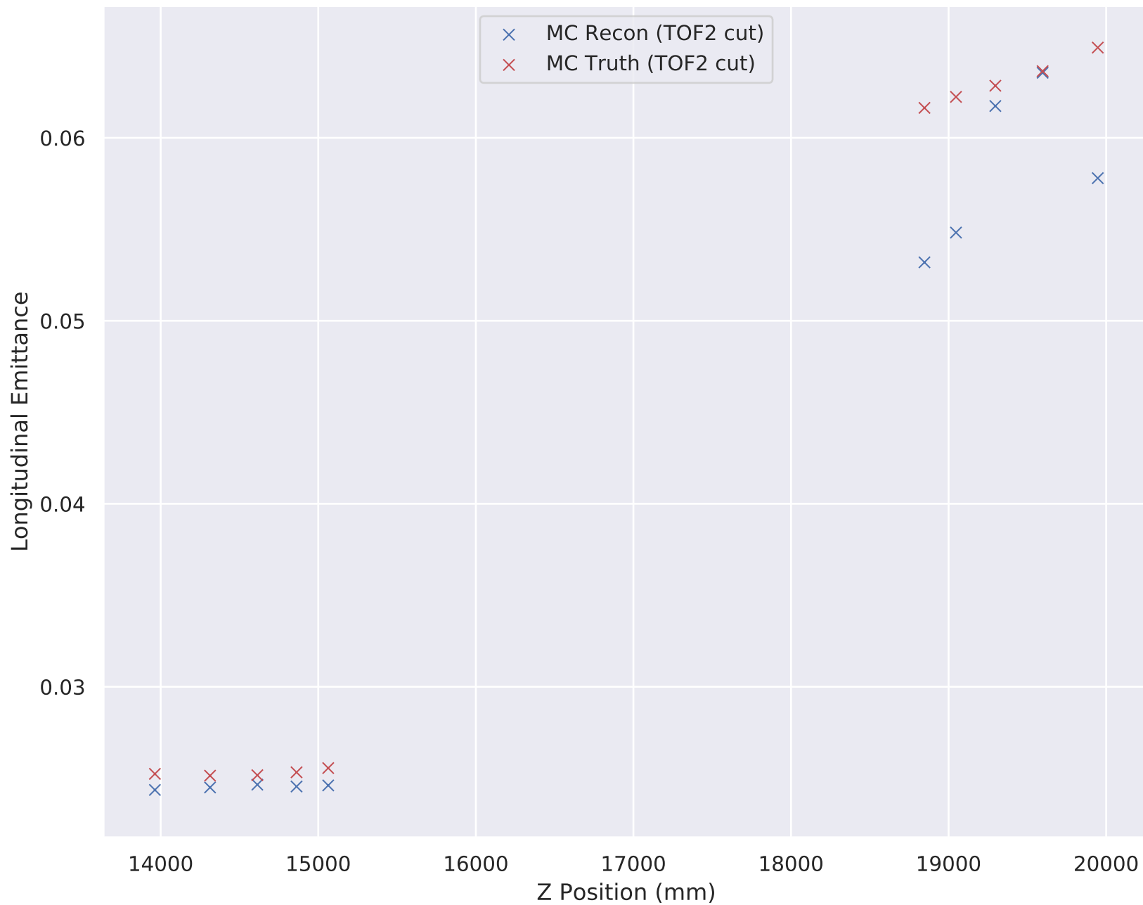
6-140 Wedge Solenoid Longitudinal Emittance (TOF2 cut)
