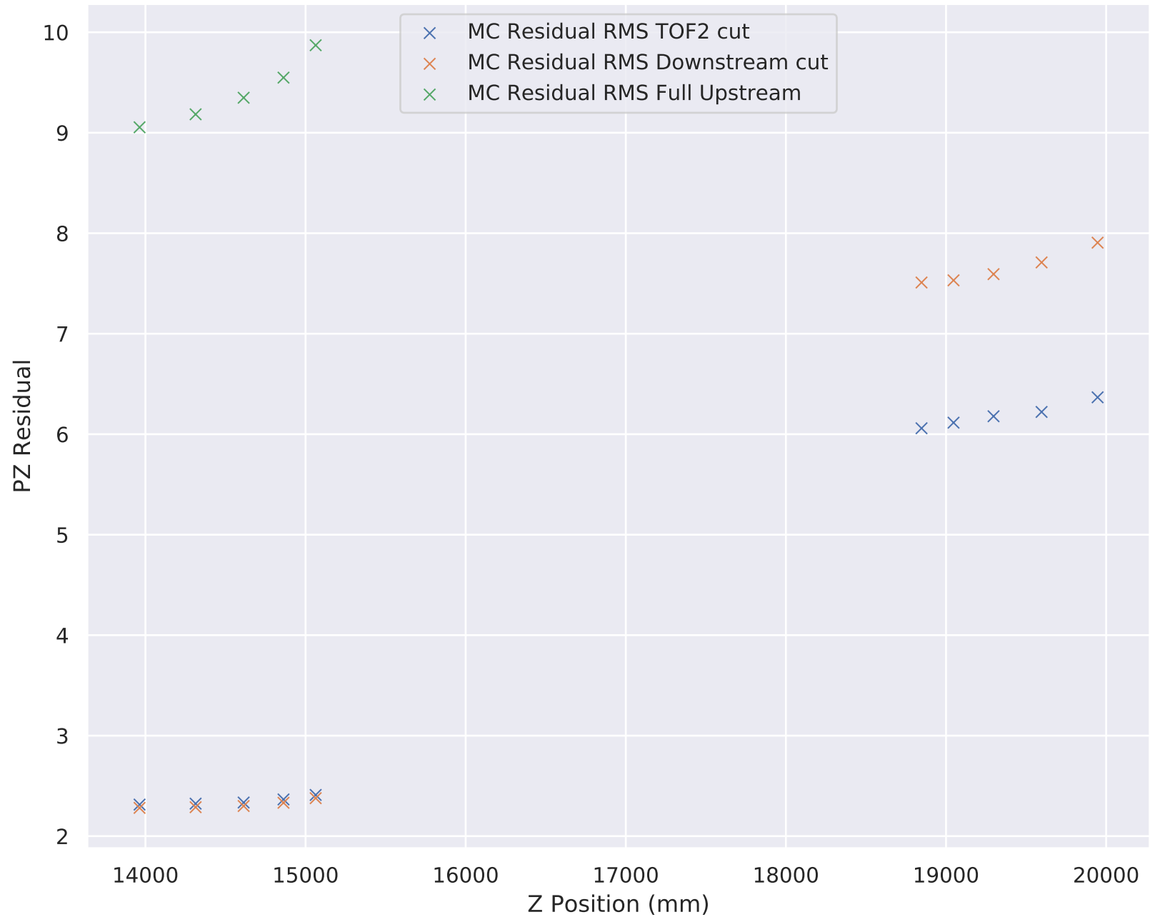
6-140 Wedge Solenoid PZ Residual RMS
