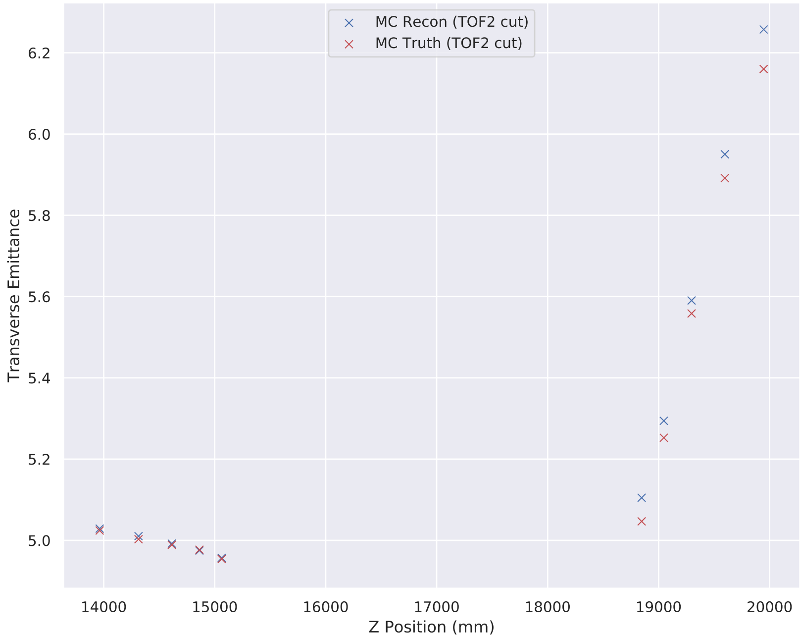
6-140 Wedge Solenoid Transverse Emittance (TOF2 cut)
