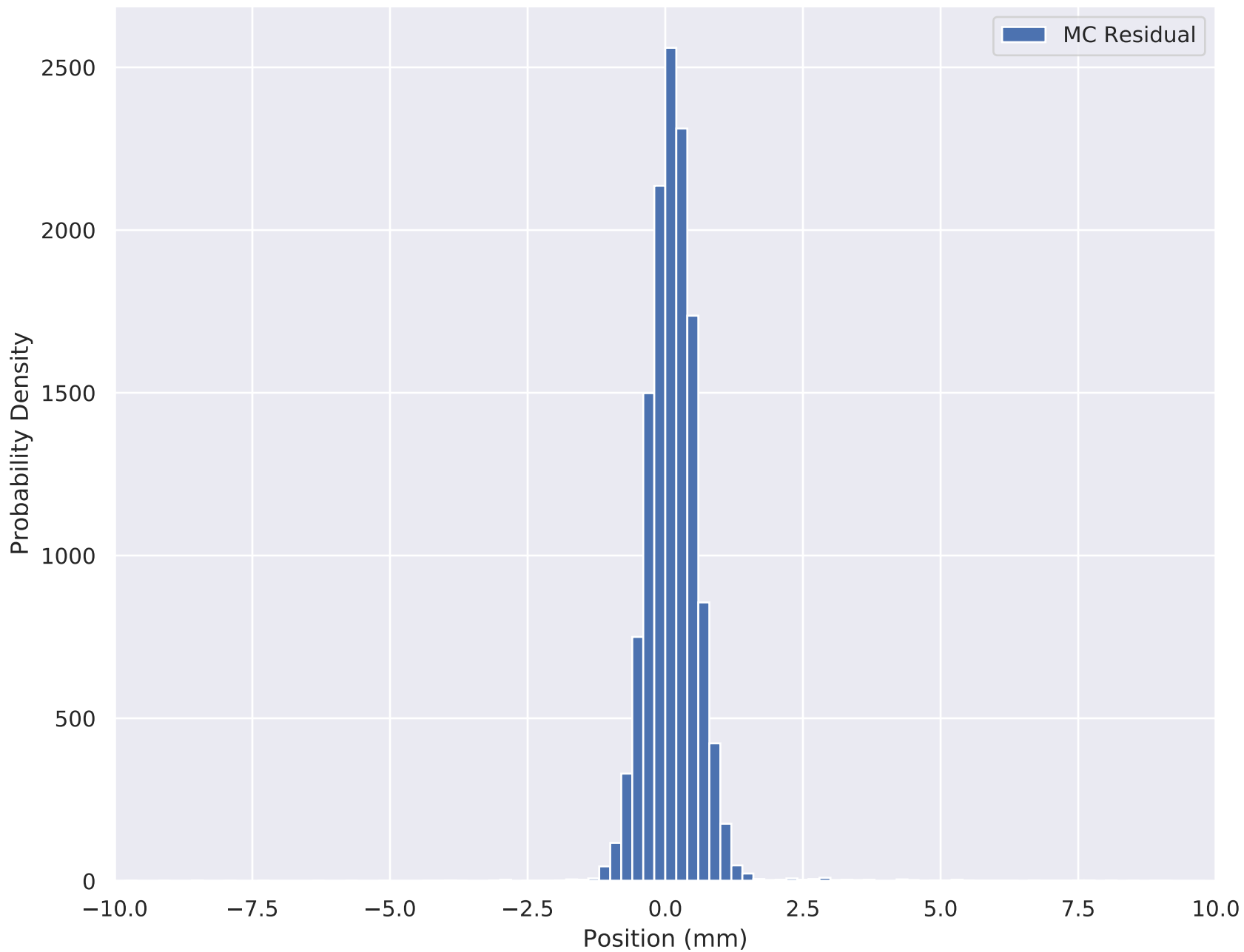
6-140 Wedge Solenoid X Residual (Downstream cut) TKD S1
