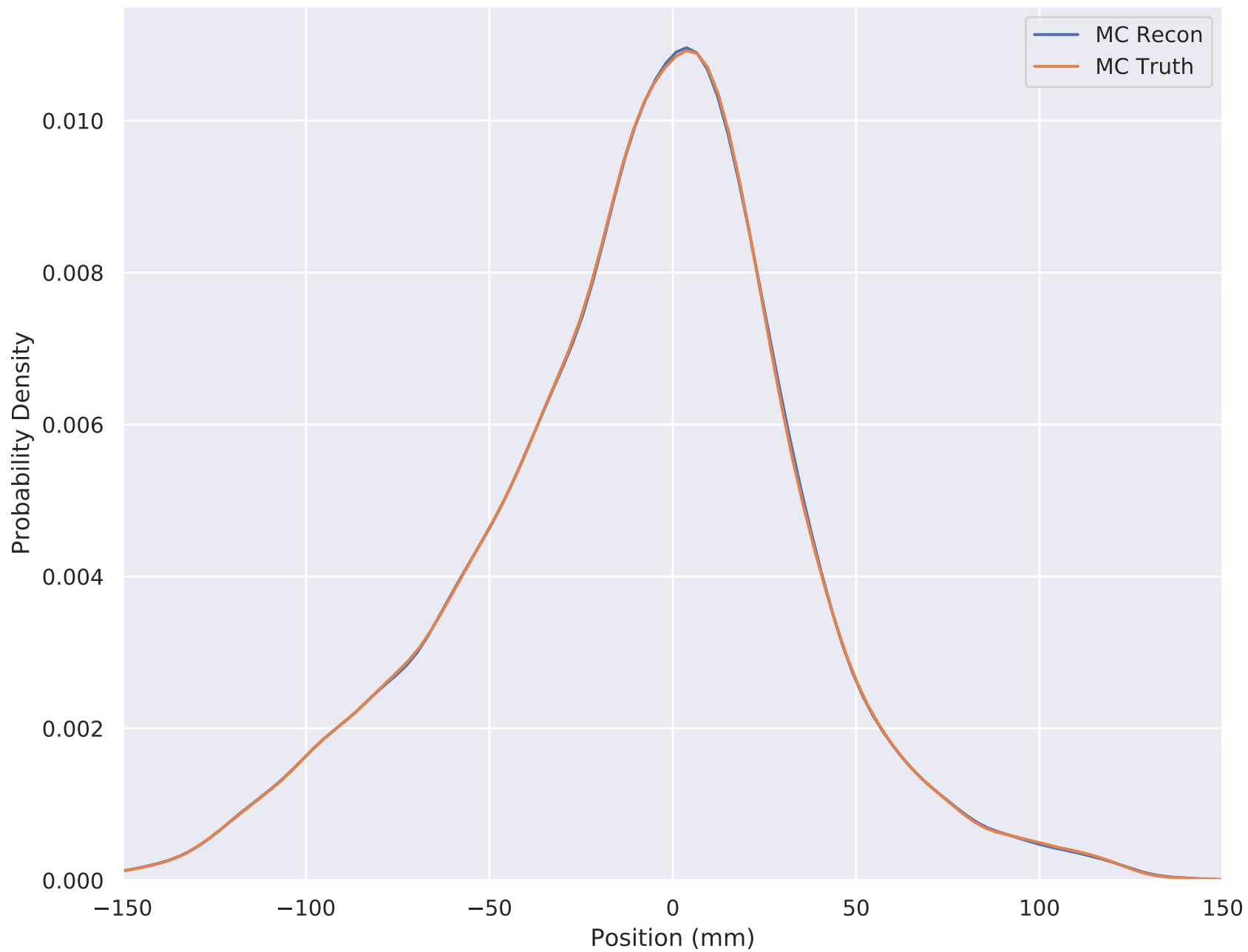
6-140 Wedge Solenoid X Position (Downstream cut) TKD S5
