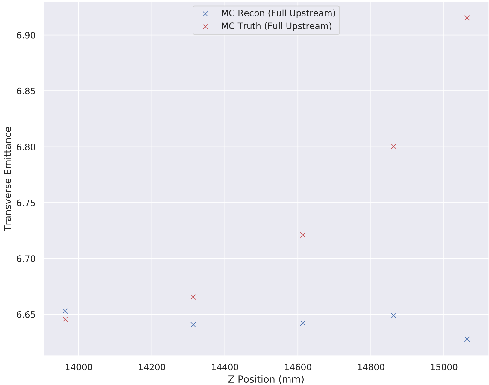
6-140 Wedge Solenoid Transverse Emittance (Full Upstream)
