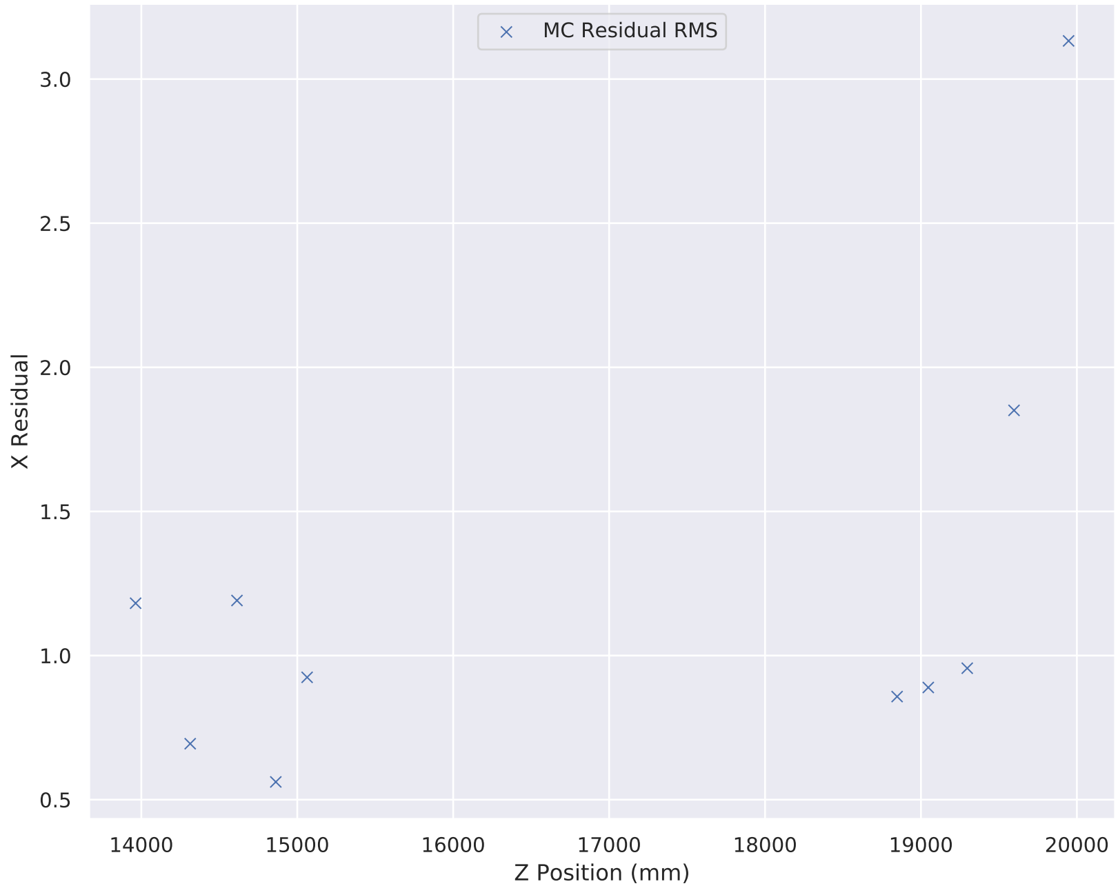
6-140 Wedge Solenoid X Residual RMS (Downstream cut)
