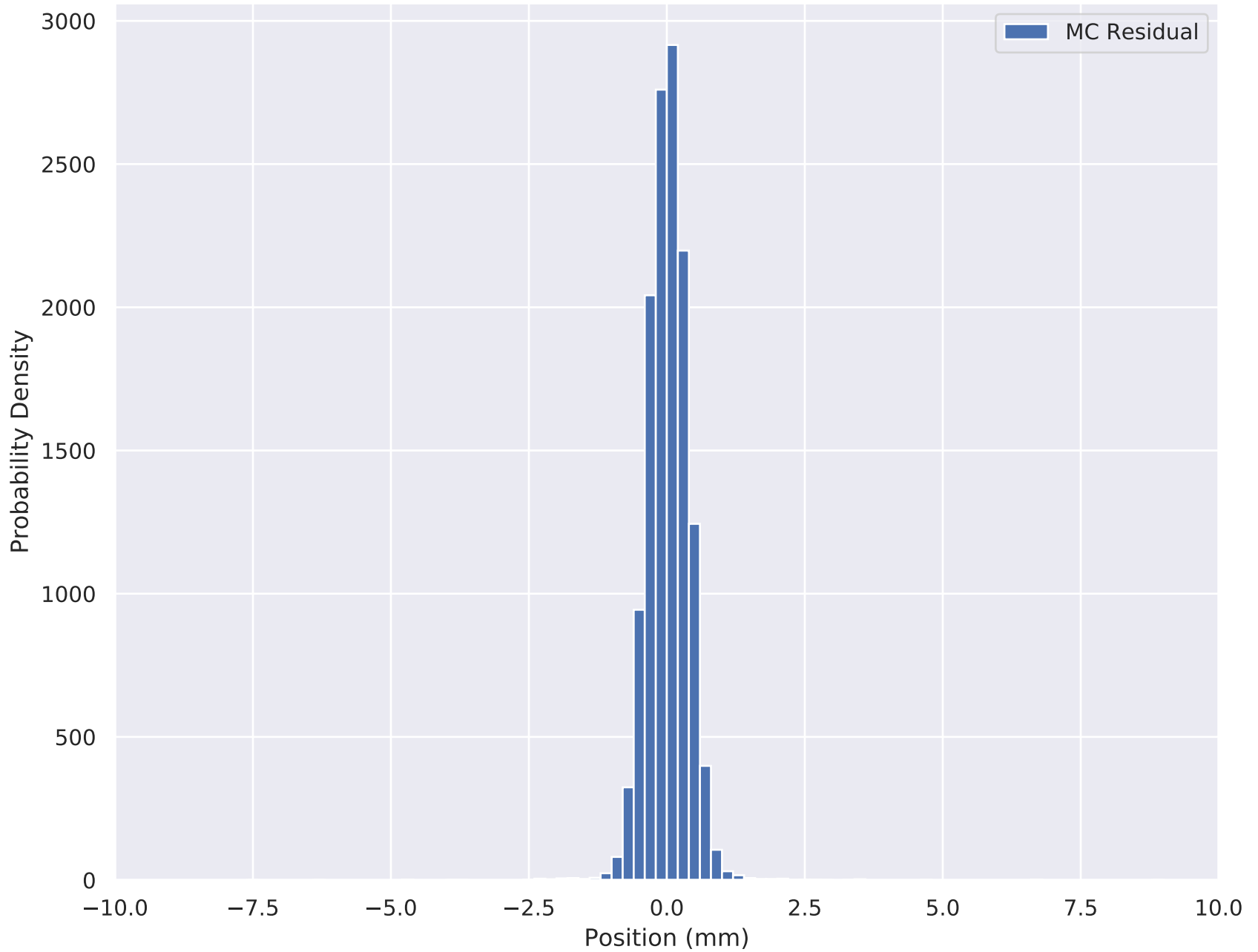
6-140 Wedge Solenoid X Residual (Downstream cut) TKU S2
