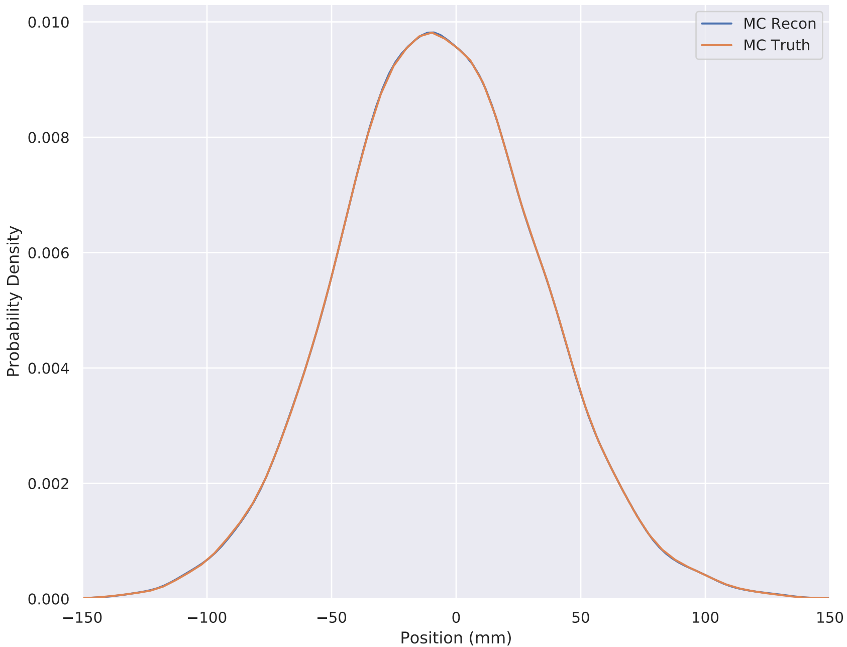
6-140 Wedge Solenoid X Position (Full Upstream) TKU S4
