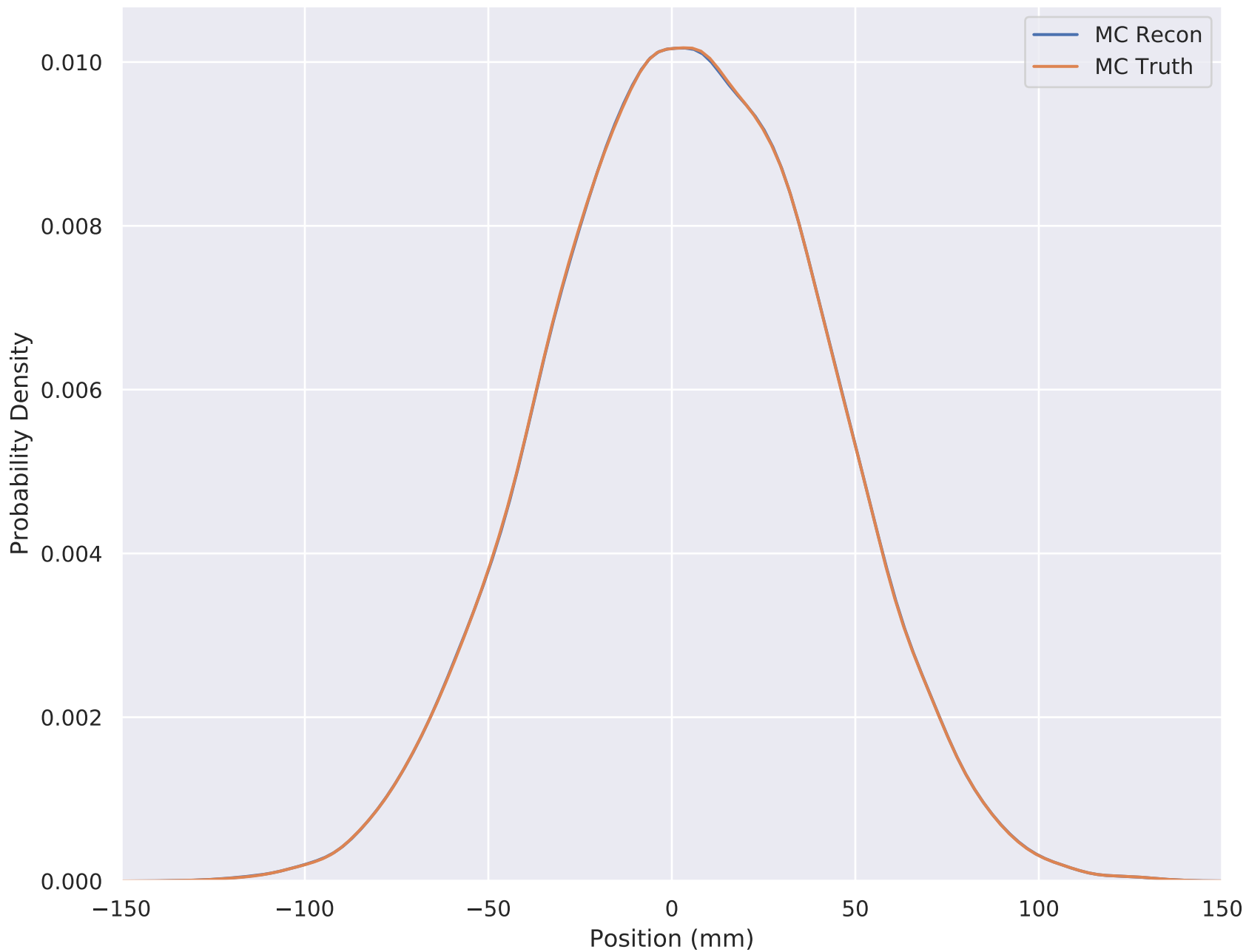
6-140 Wedge Solenoid X Position (Full Upstream) TKU S5
