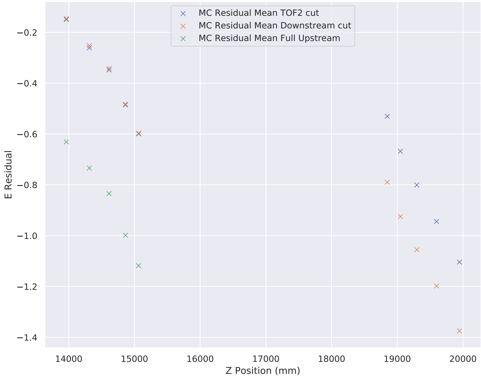
6-140 Wedge Solenoid E Residual Mean
