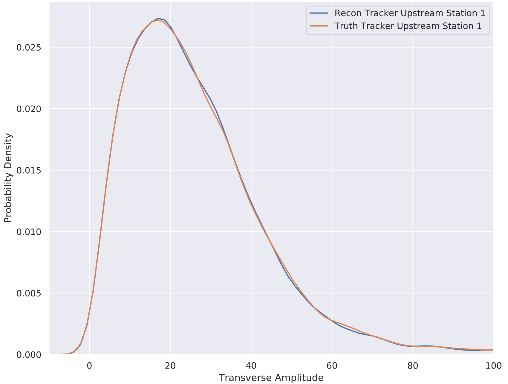
6-140 Wedge Solenoid Amplitude MC (Upstream)
