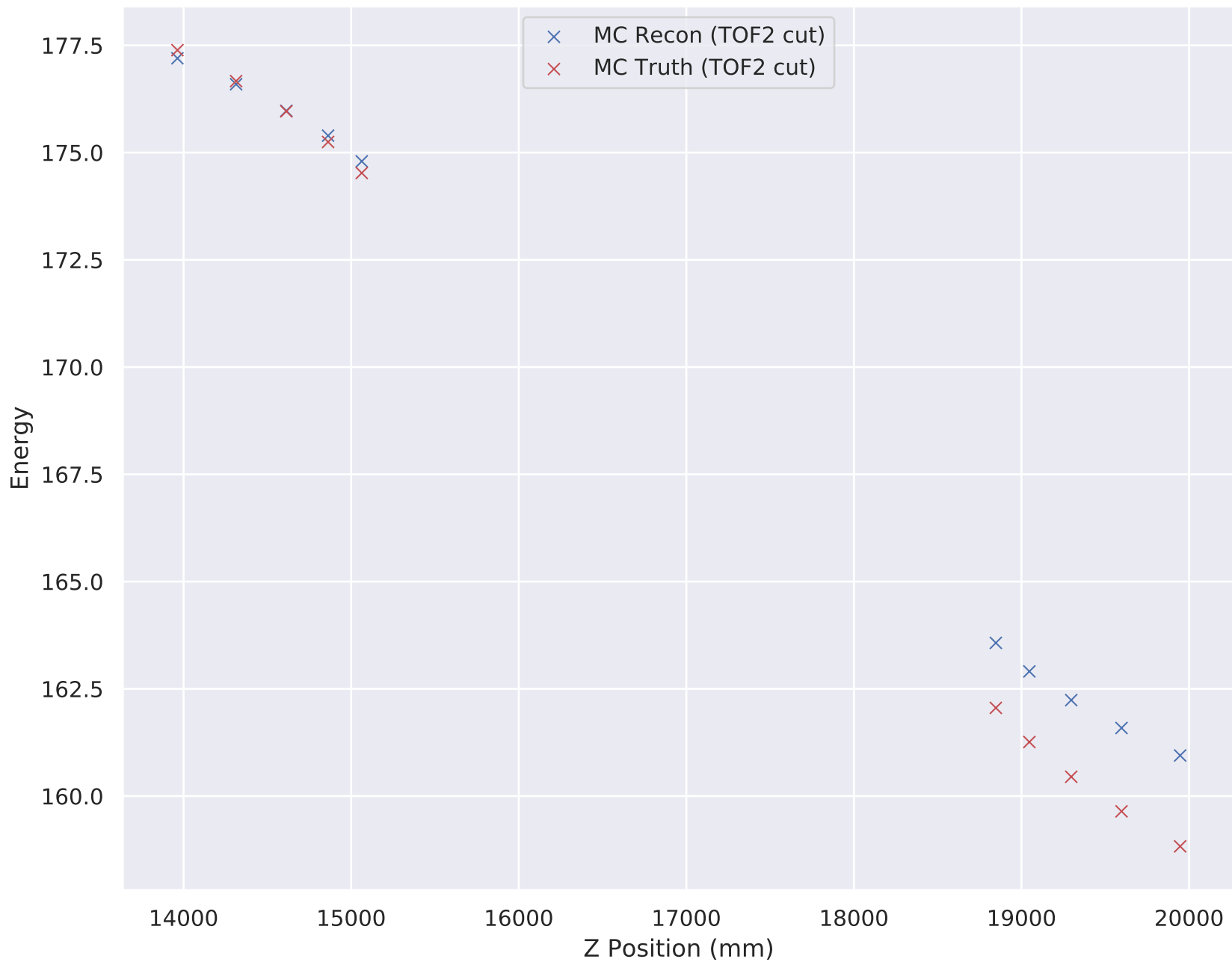
6-140 Wedge Solenoid Energy (TOF2 cut)
