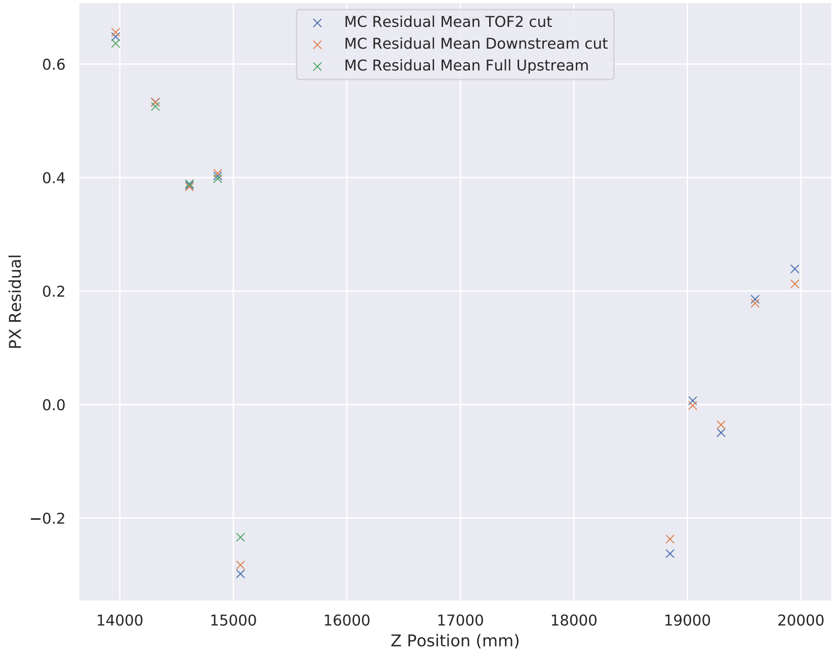
6-140 Wedge Solenoid PX Residual Mean
