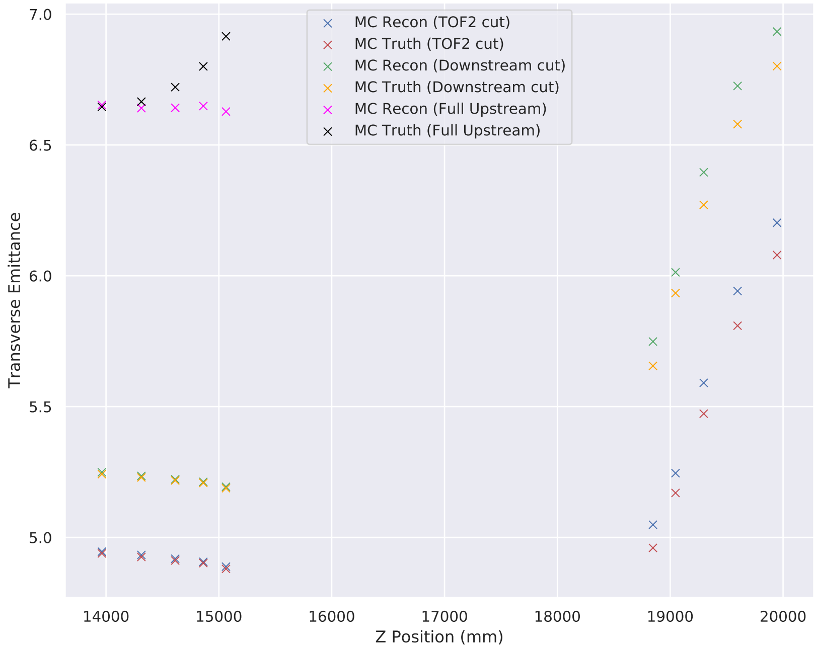
6-140 Wedge Solenoid Transverse Emittance
