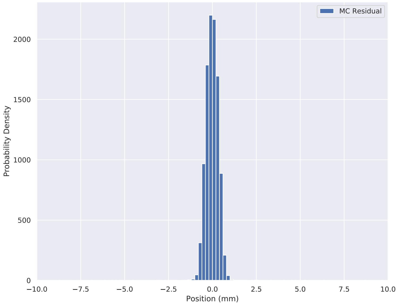
6-140 Wedge Solenoid X Residual (TOF2 cut) TKU S5
