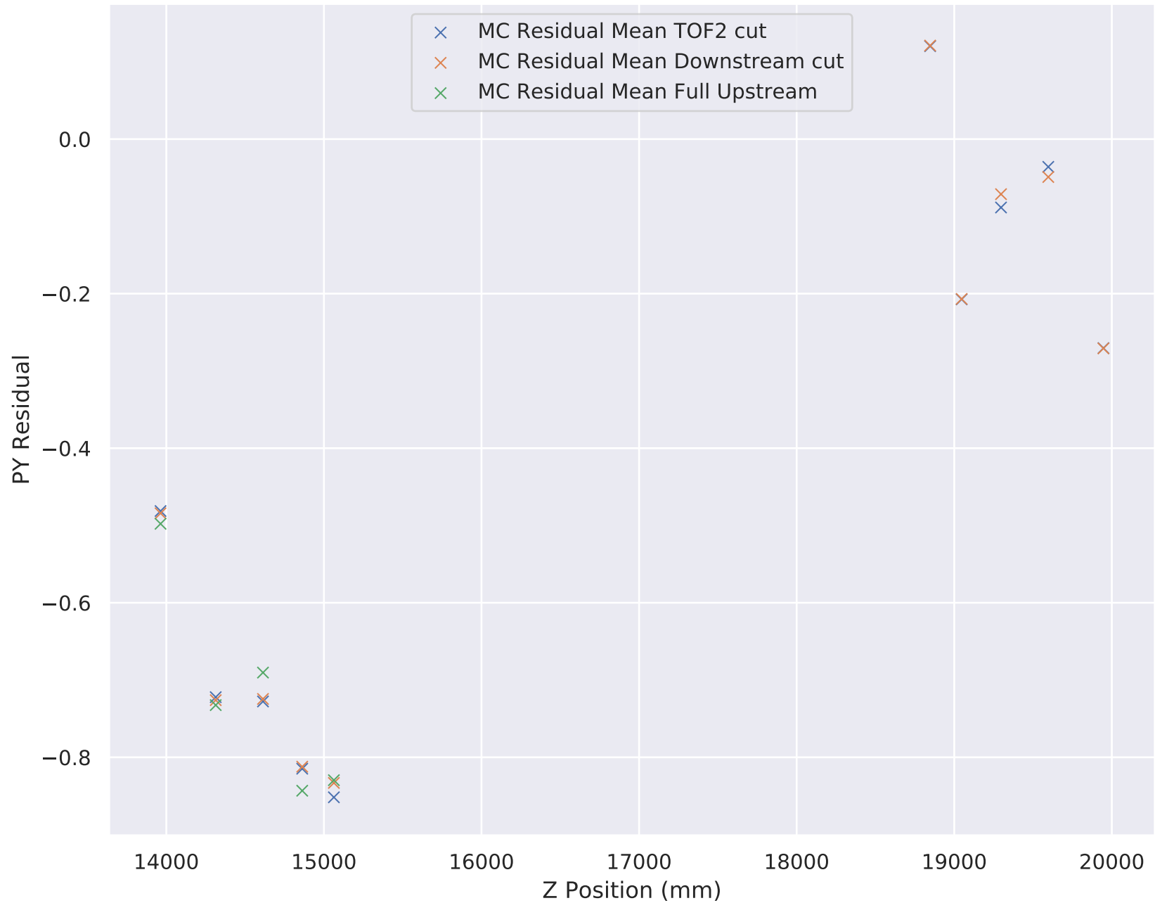
6-140 Wedge Solenoid PY Residual Mean
