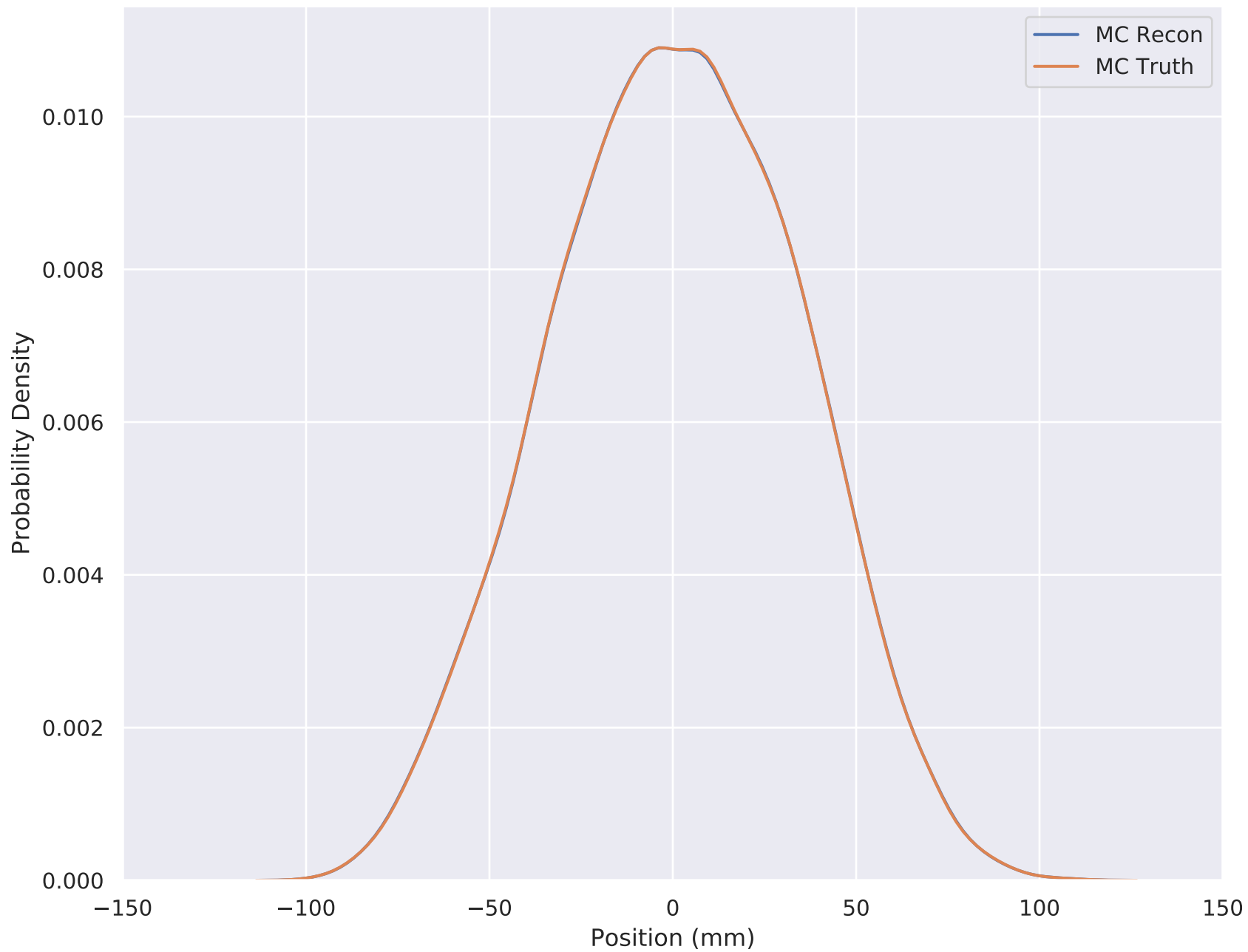
6-140 Wedge Solenoid X Position (Downstream cut) TKU S5
