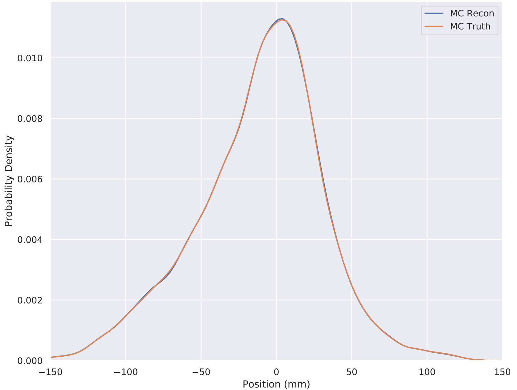
6-140 Wedge Solenoid X Position (TOF2 cut) TKD S5
