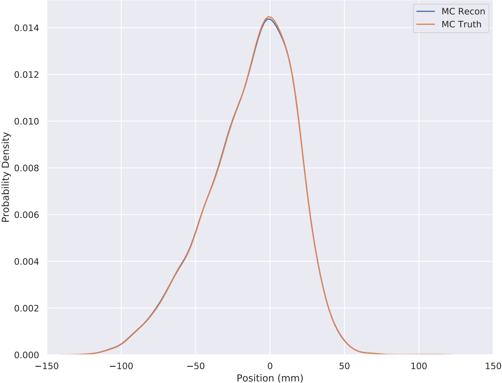
6-140 Wedge Solenoid X Position (TOF2 cut) TKD S1
