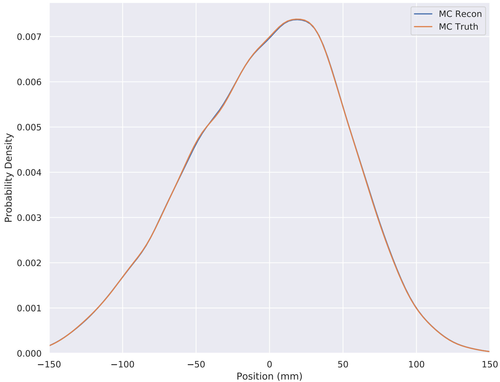
6-140 Wedge Solenoid X Position (TOF2 cut) TKD S4
