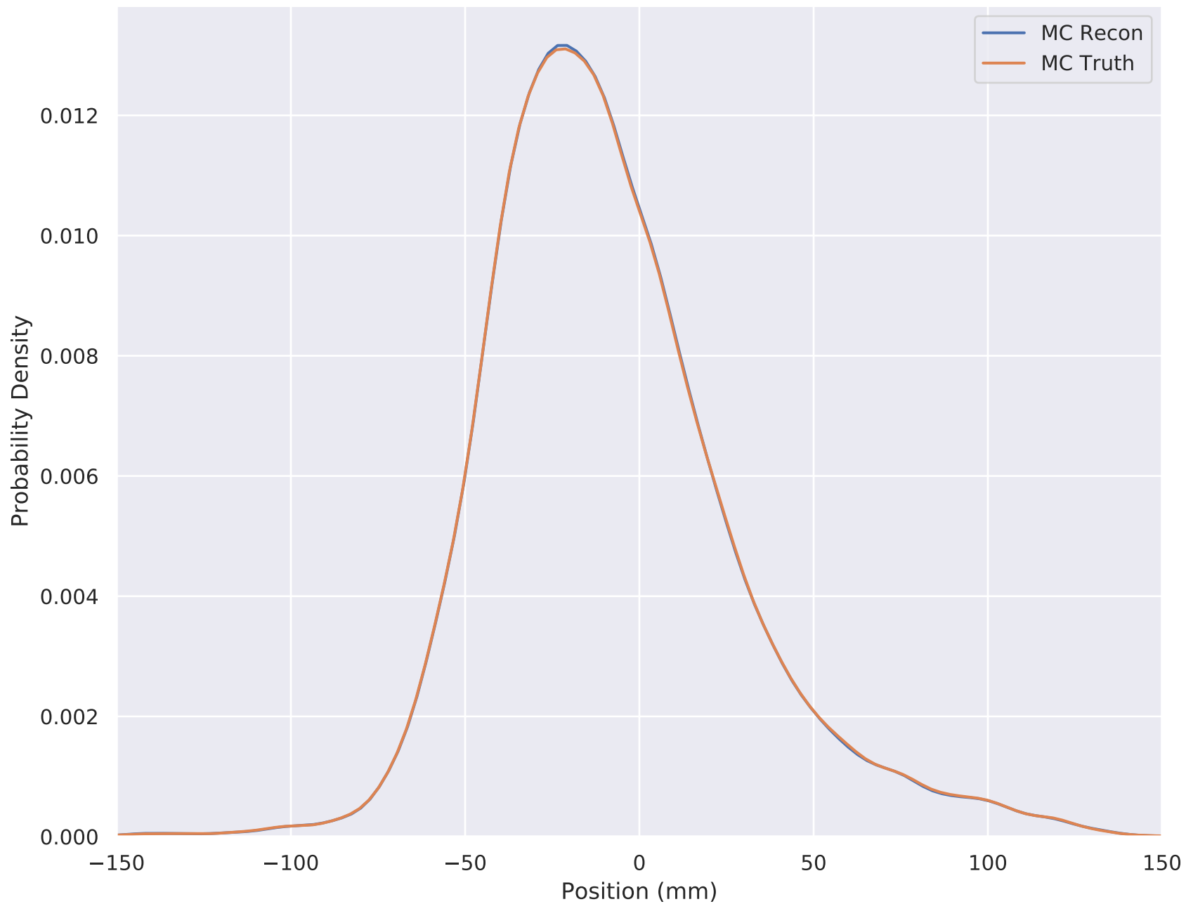
6-140 Wedge Solenoid X Position (Downstream cut) TKD S2
