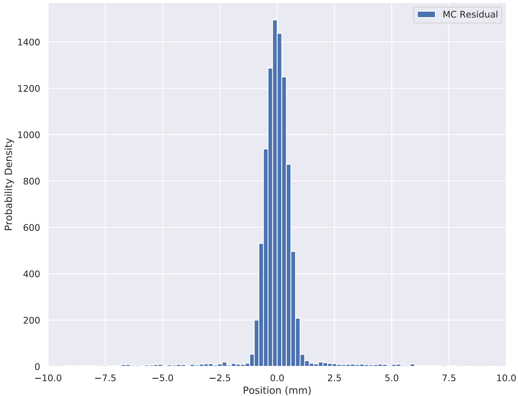
6-140 Wedge Solenoid X Residual (TOF2 cut) TKD S5
