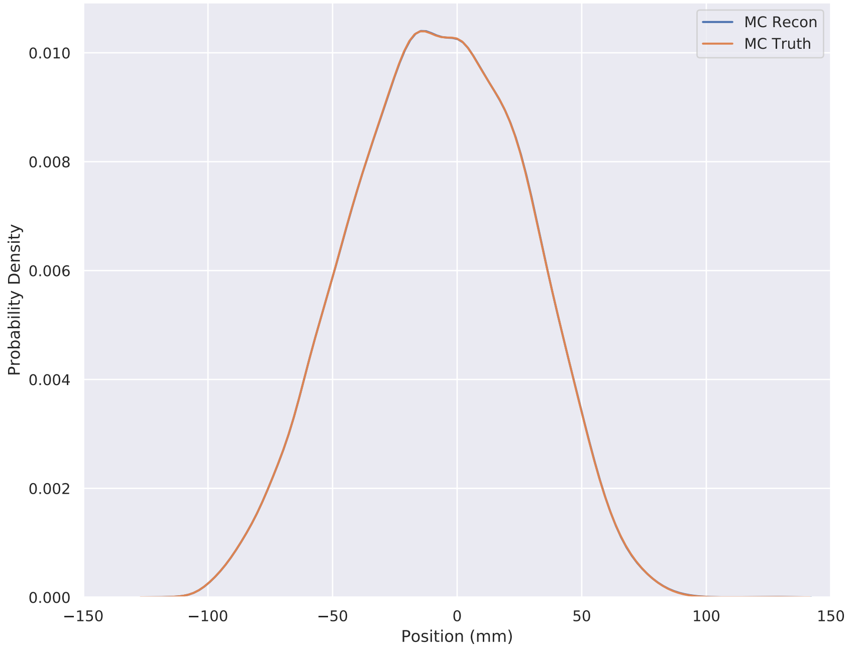
6-140 Wedge Solenoid X Position (Downstream cut) TKU S3
