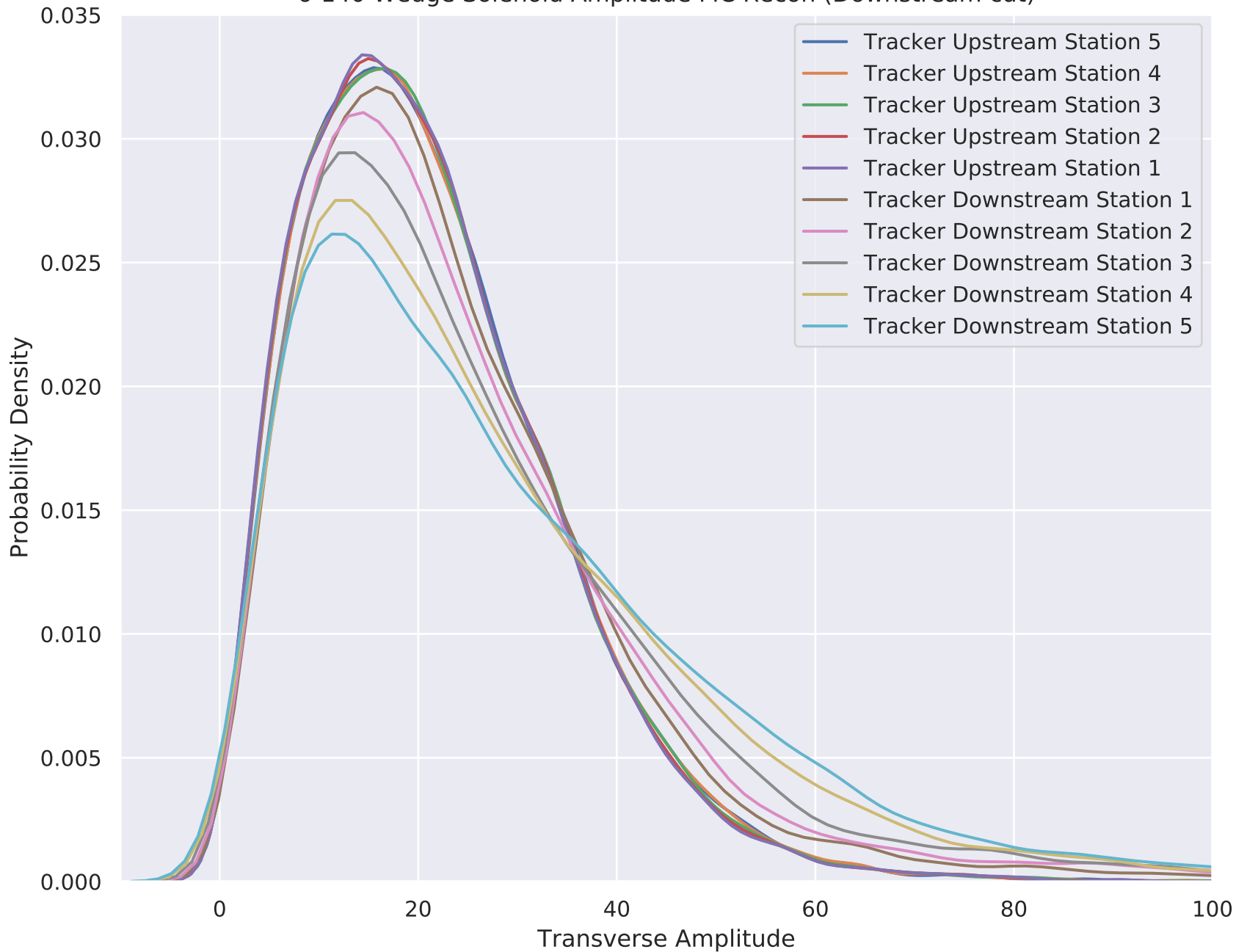
6-140 Wedge Solenoid Amplitude MC Recon (Downstream cut)
