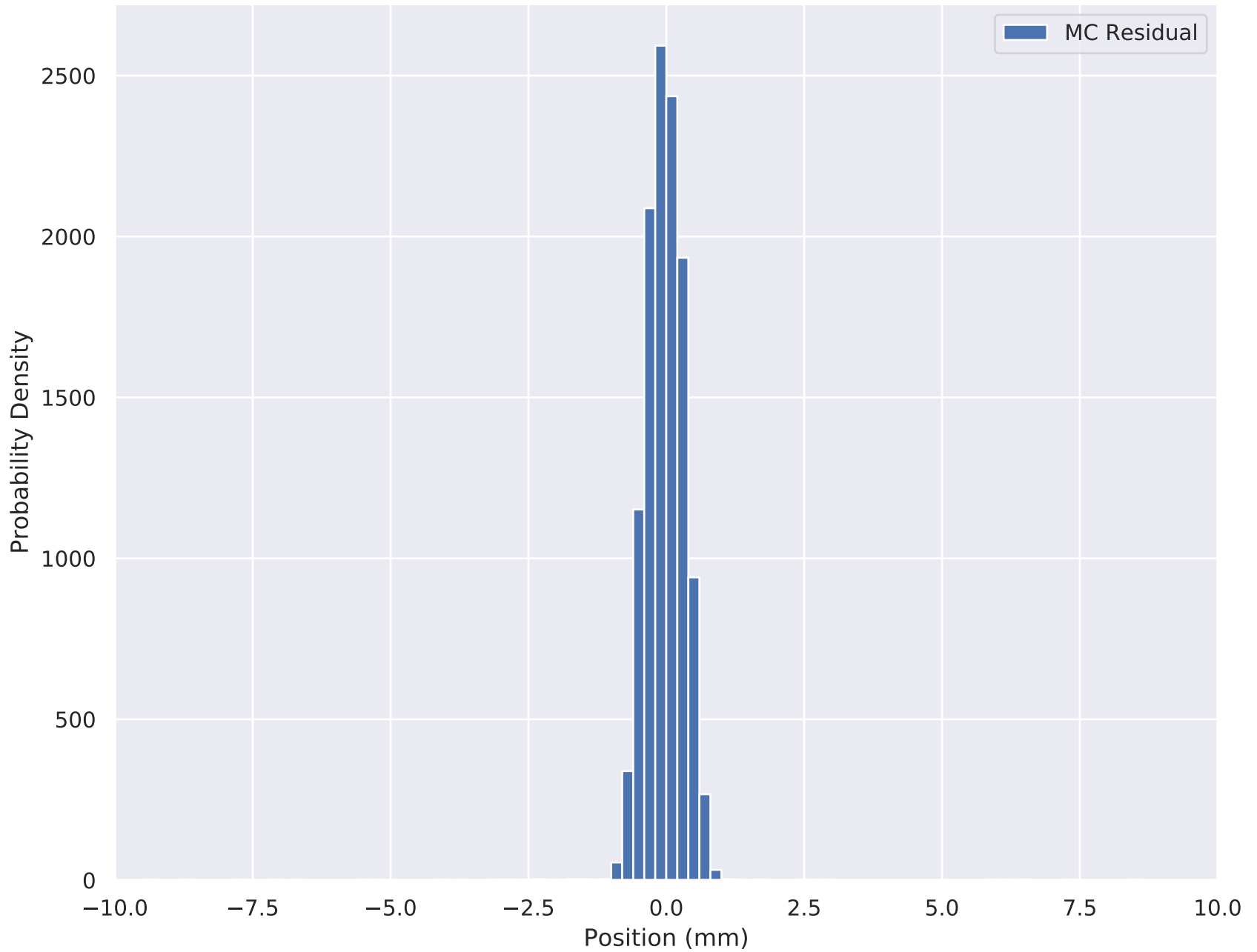
6-140 Wedge Solenoid X Residual (Downstream cut) TKU S5
