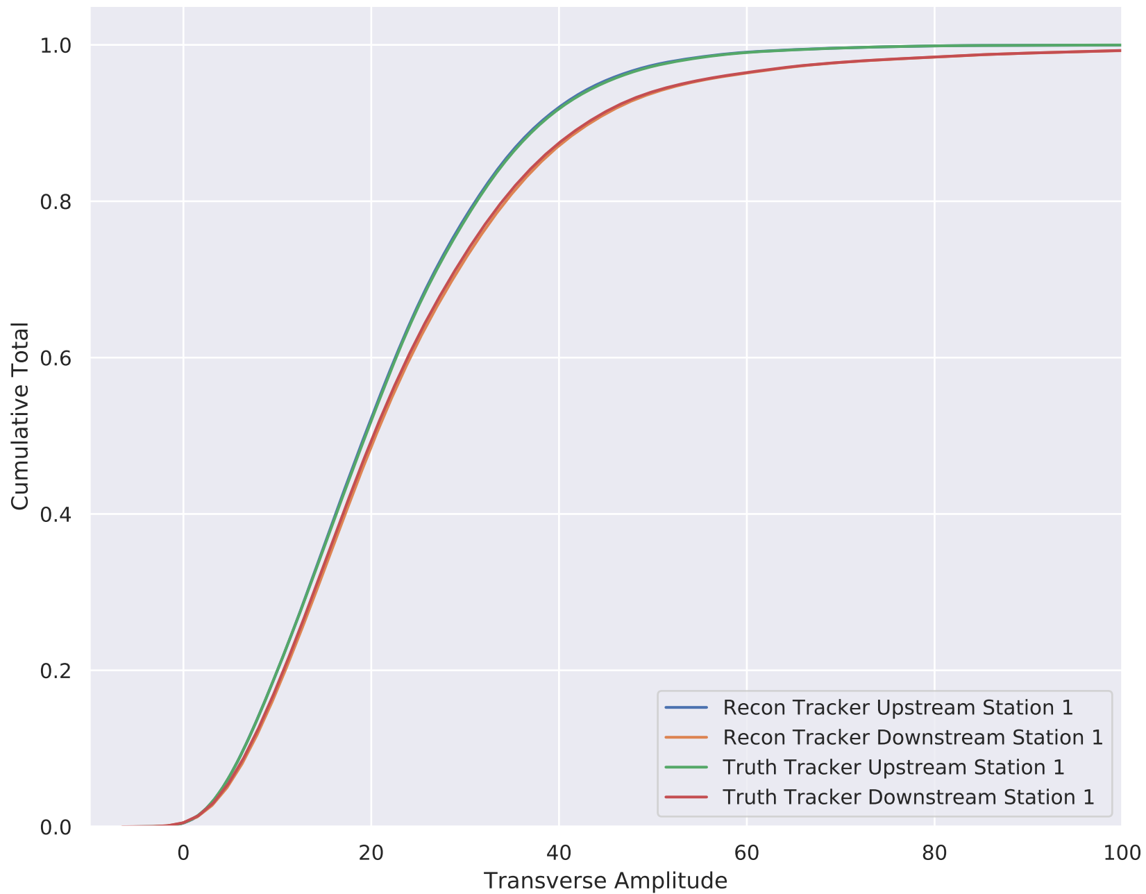
6-140 Wedge Solenoid Amplitude MC (Downstream cut)
