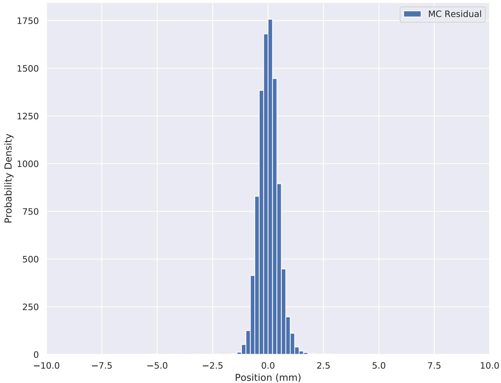
6-140 Wedge Solenoid X Residual (TOF2 cut) TKD S1
