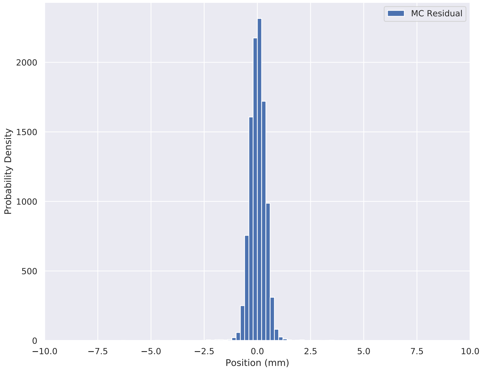
6-140 Wedge Solenoid X Residual (TOF2 cut) TKU S2
