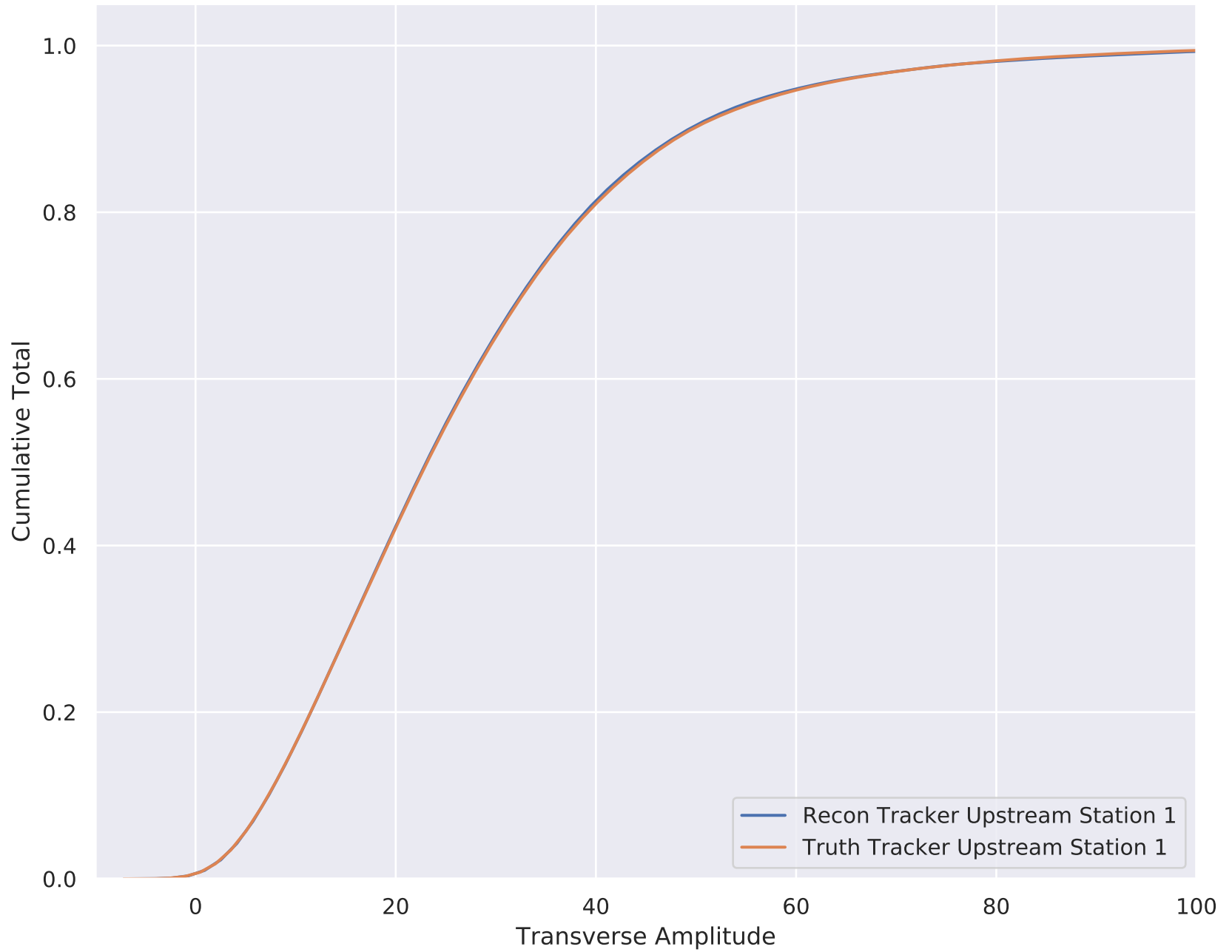
6-140 Wedge Solenoid Amplitude MC (Upstream)
