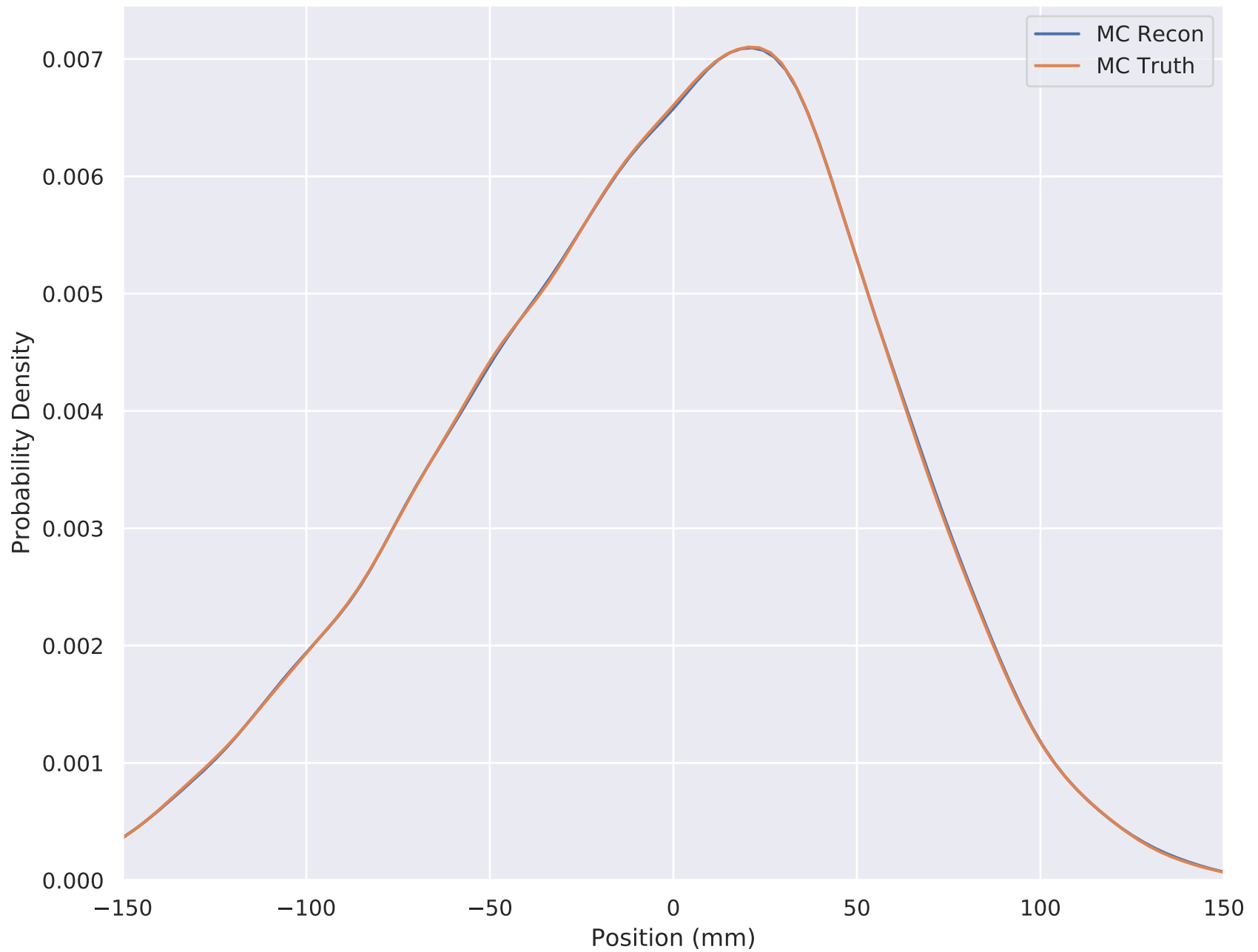
6-140 Wedge Solenoid X Position (Downstream cut) TKD S4
