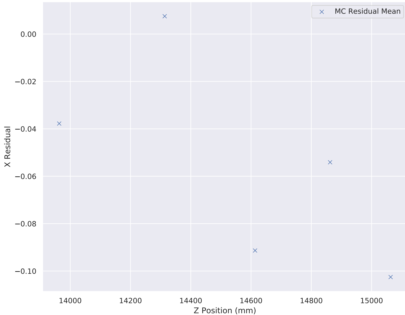
6-140 Wedge Solenoid X Residual Mean (Full Upstream)
