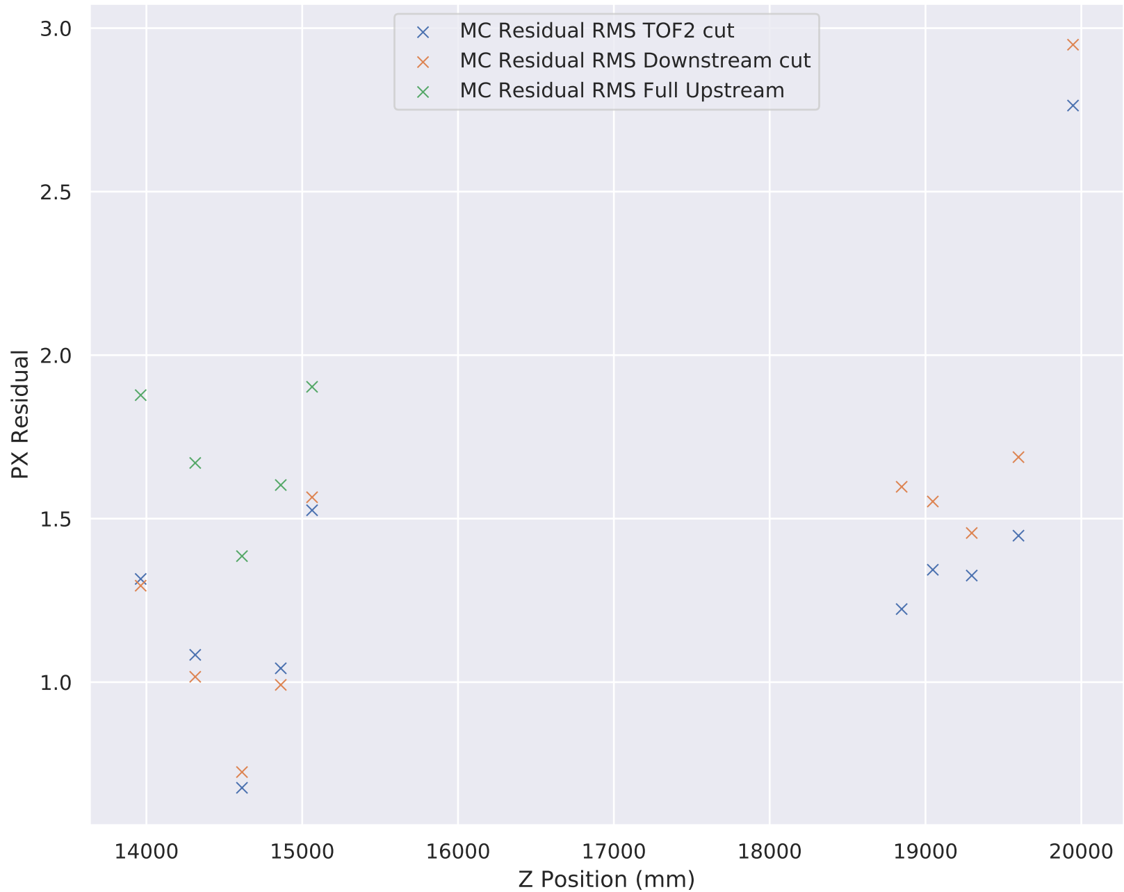
6-140 Wedge Solenoid PX Residual RMS
