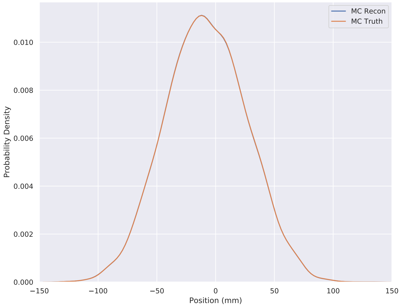
6-140 Wedge Solenoid X Position (TOF2 cut) TKU S4
