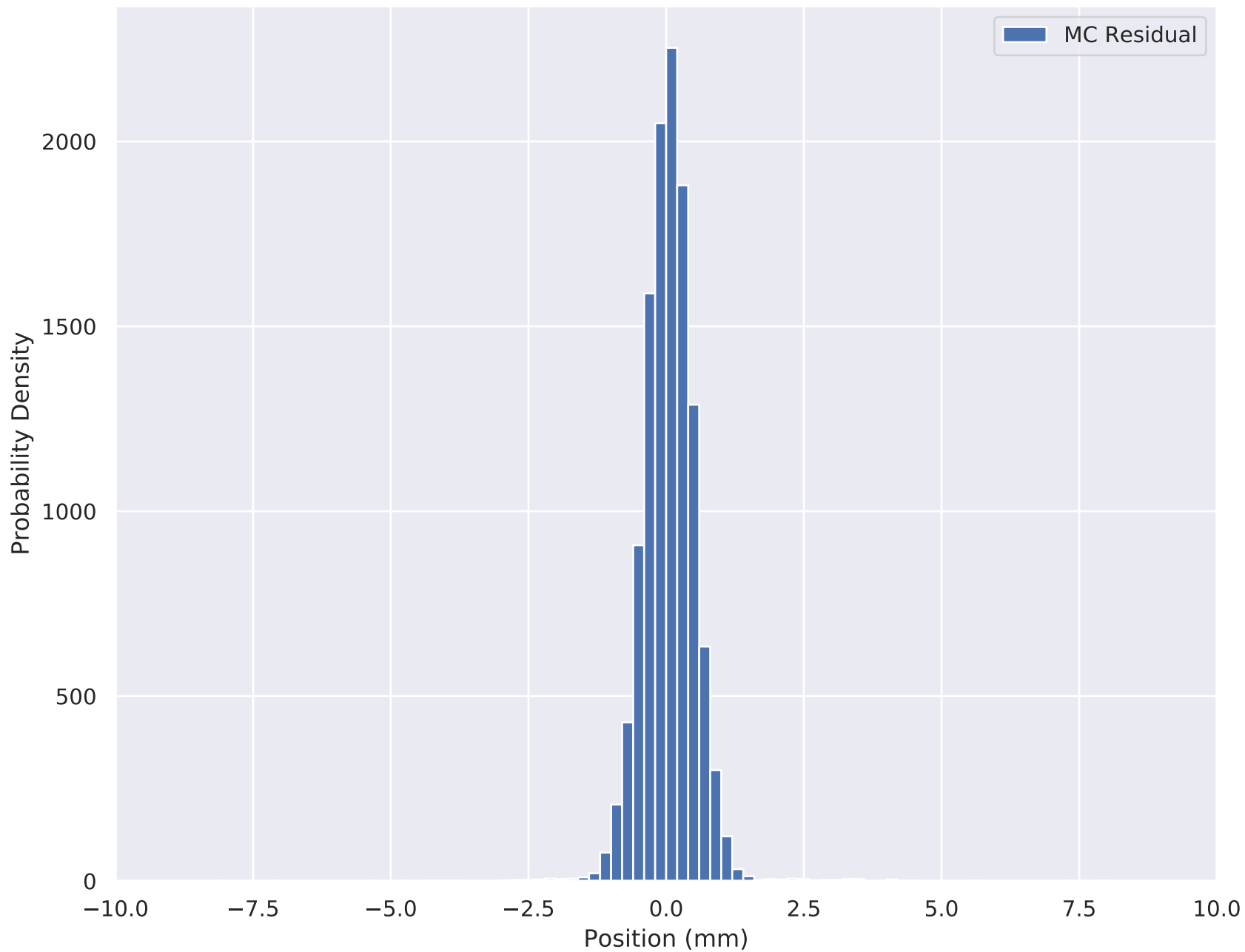
6-140 Wedge Solenoid X Residual (Downstream cut) TKD S2
