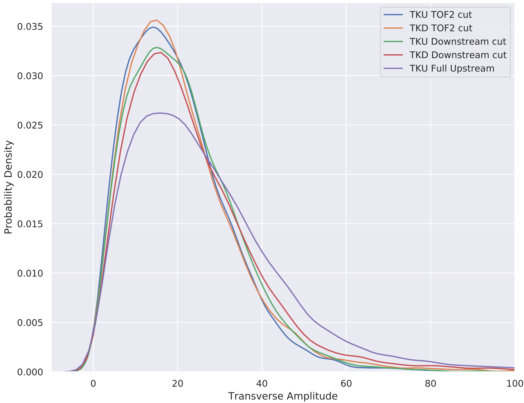
6-140 Wedge Solenoid Amplitudes MC Truth
