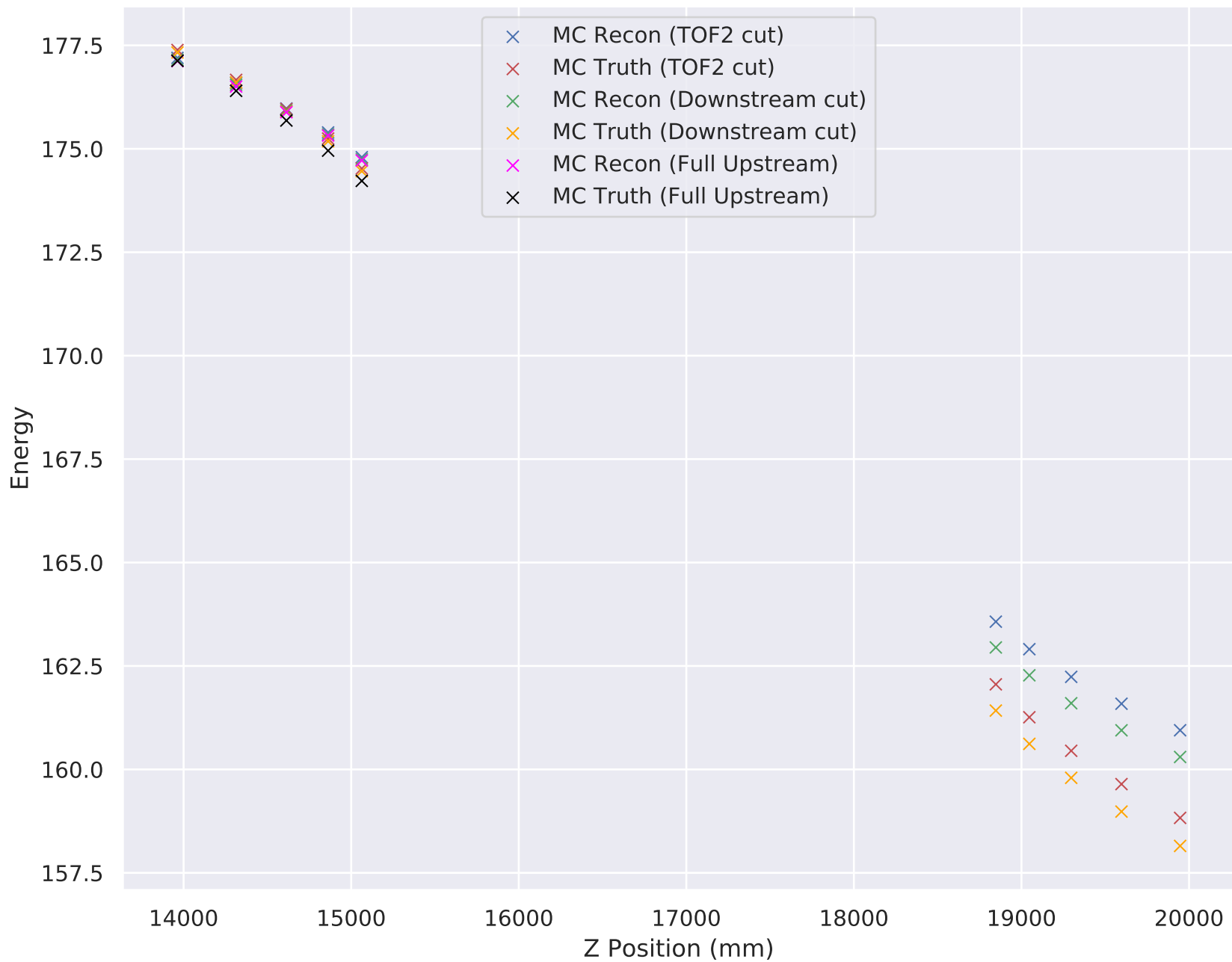
6-140 Wedge Solenoid Energy
