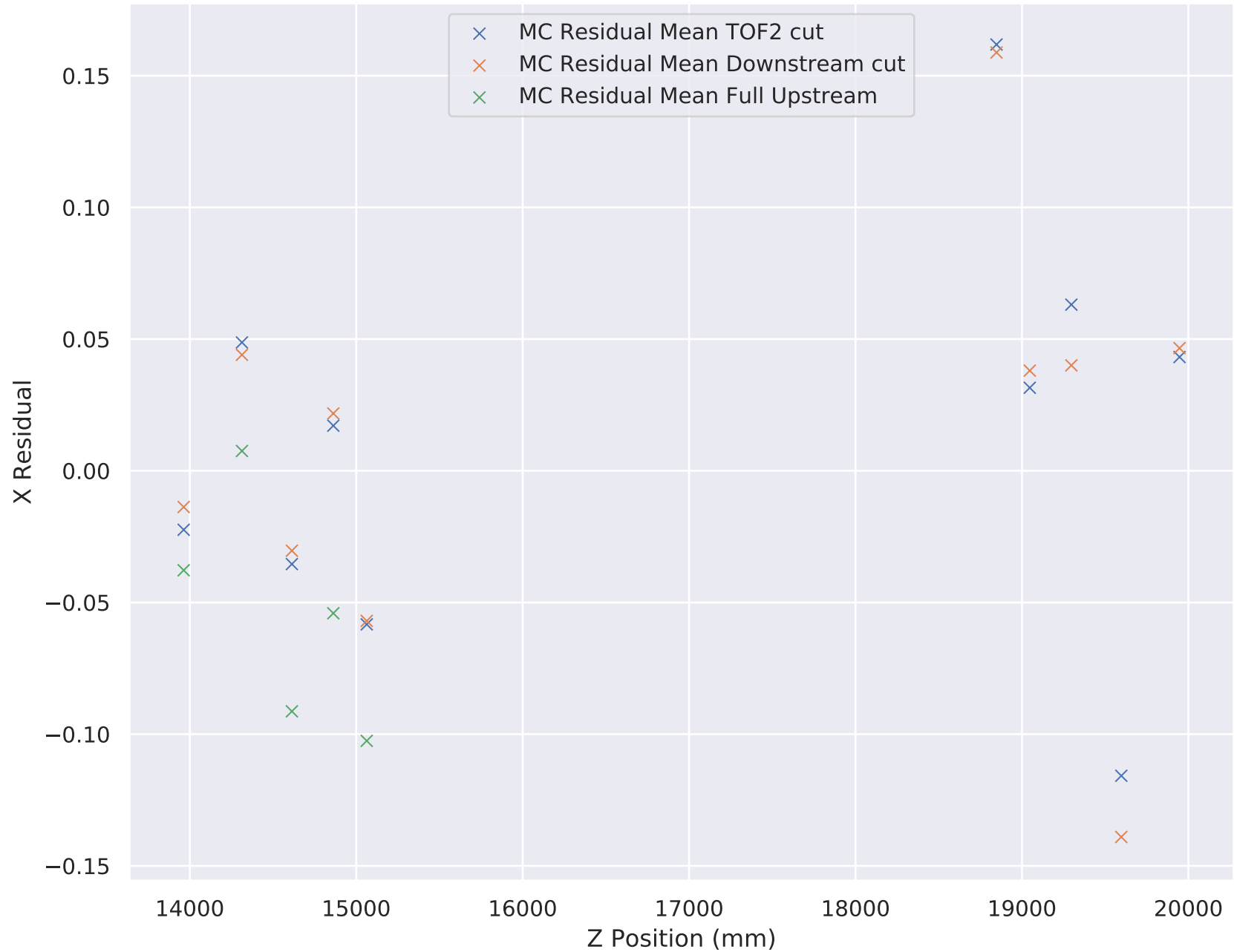
6-140 Wedge Solenoid X Residual Mean
