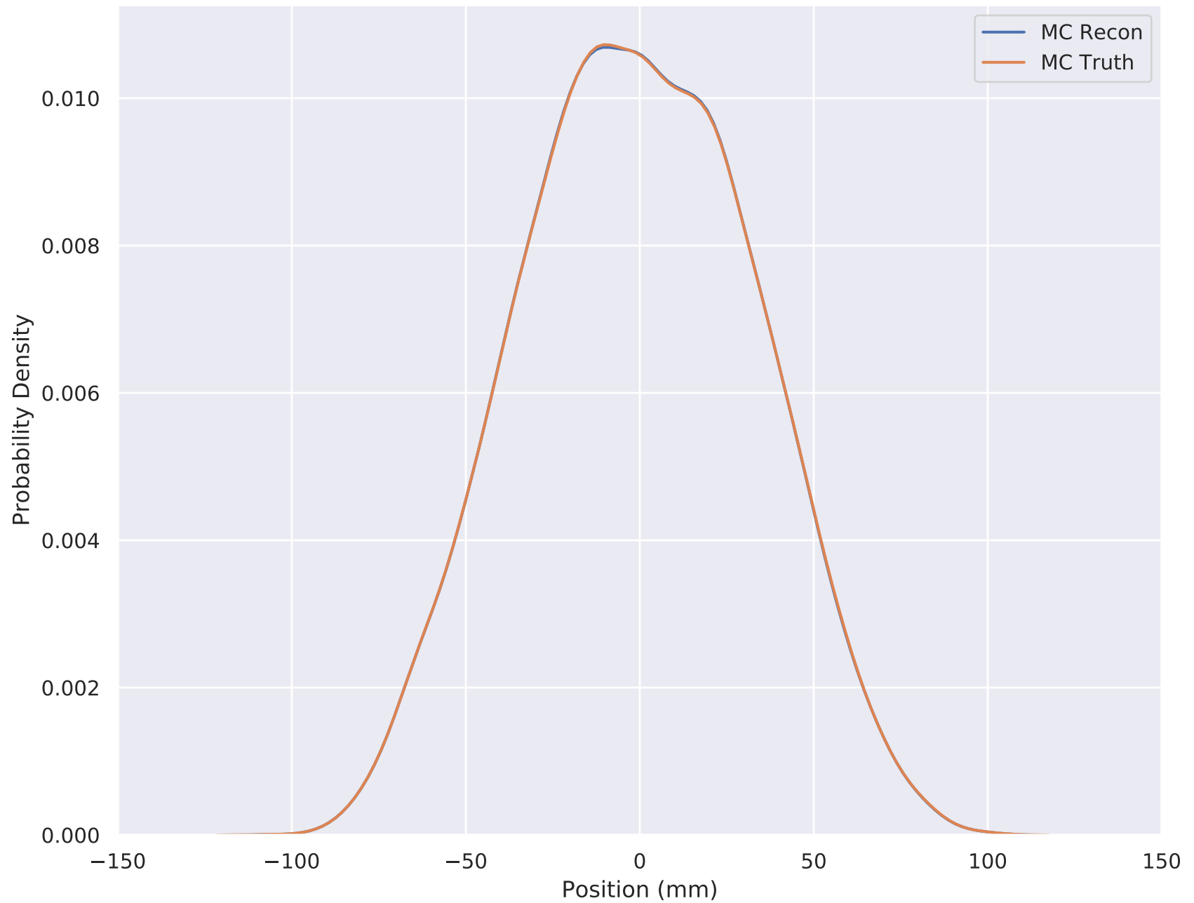
6-140 Wedge Solenoid X Position (Downstream cut) TKU S2
