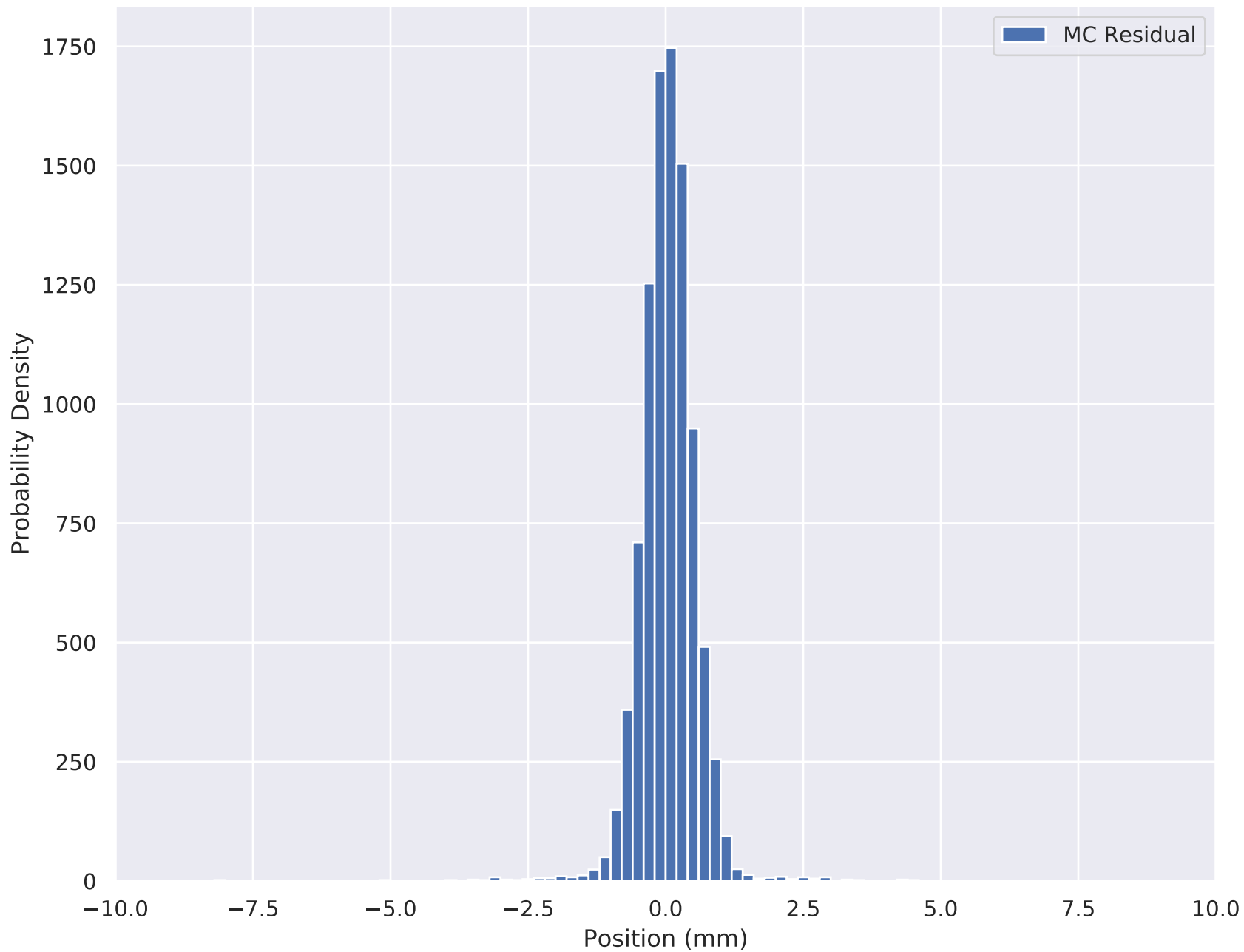
6-140 Wedge Solenoid X Residual (TOF2 cut) TKD S3
