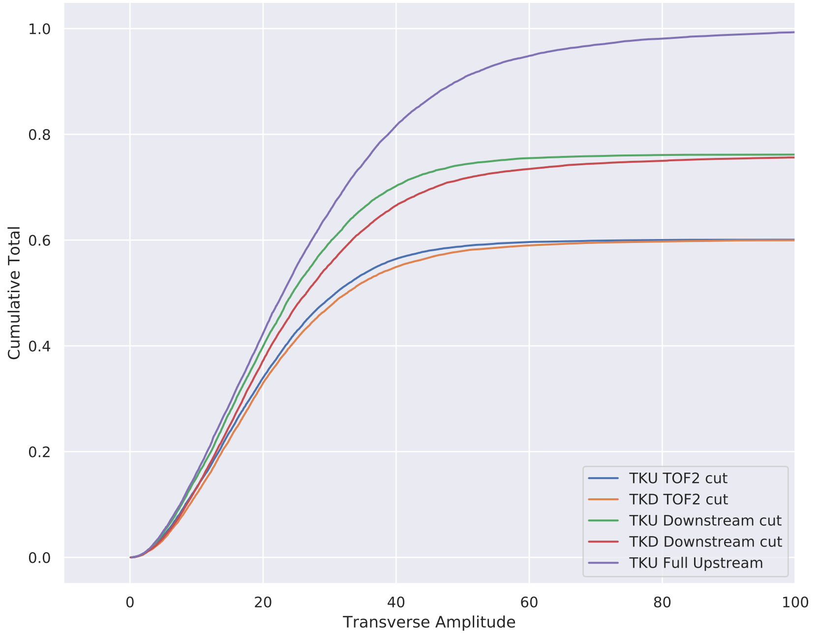
6-140 Wedge Solenoid Amplitudes MC Recon
