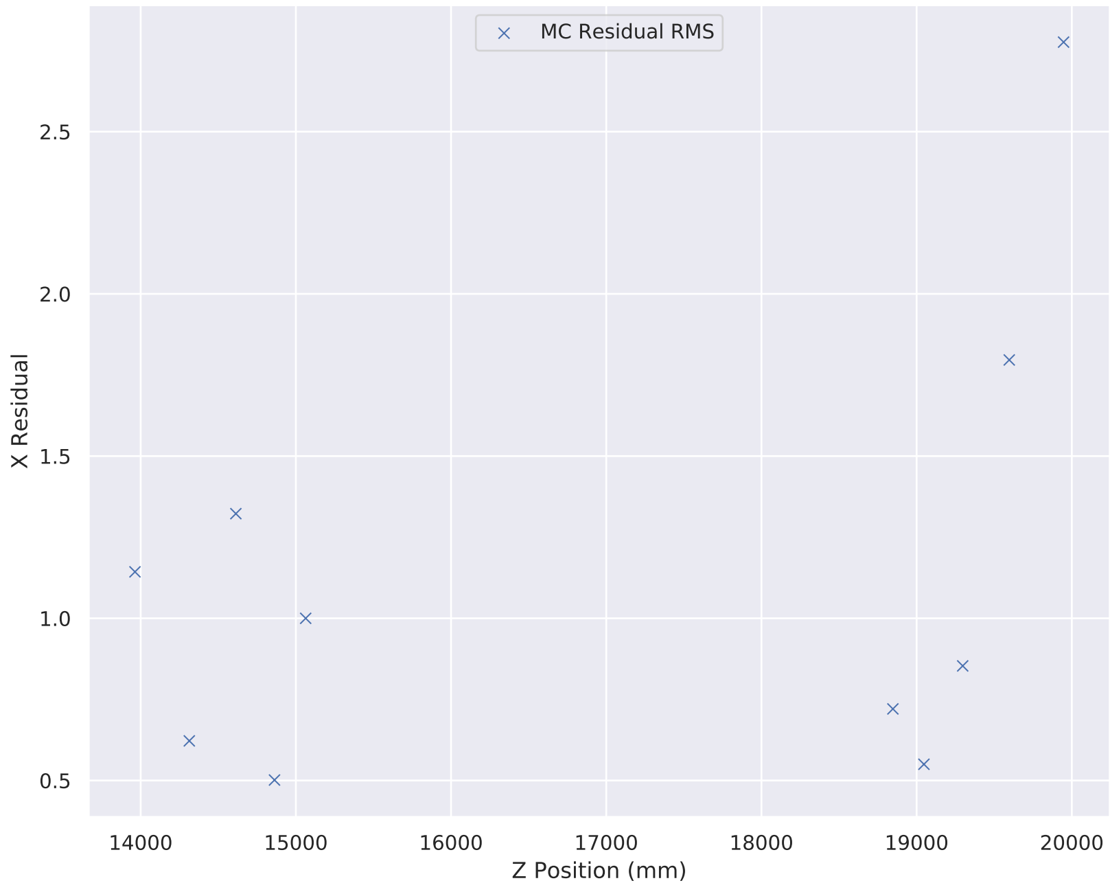
6-140 Wedge Solenoid X Residual RMS (TOF2 cut)
