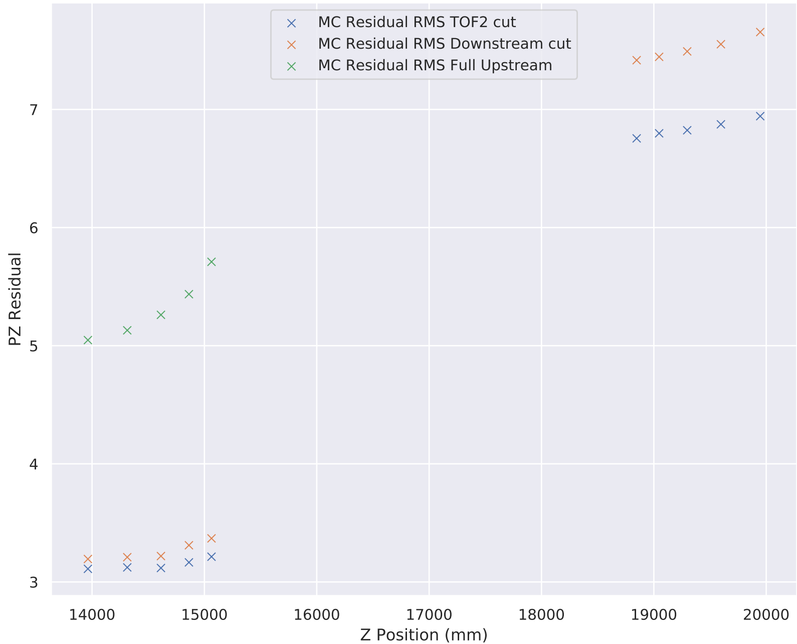
6-140 Wedge Solenoid PZ Residual RMS
