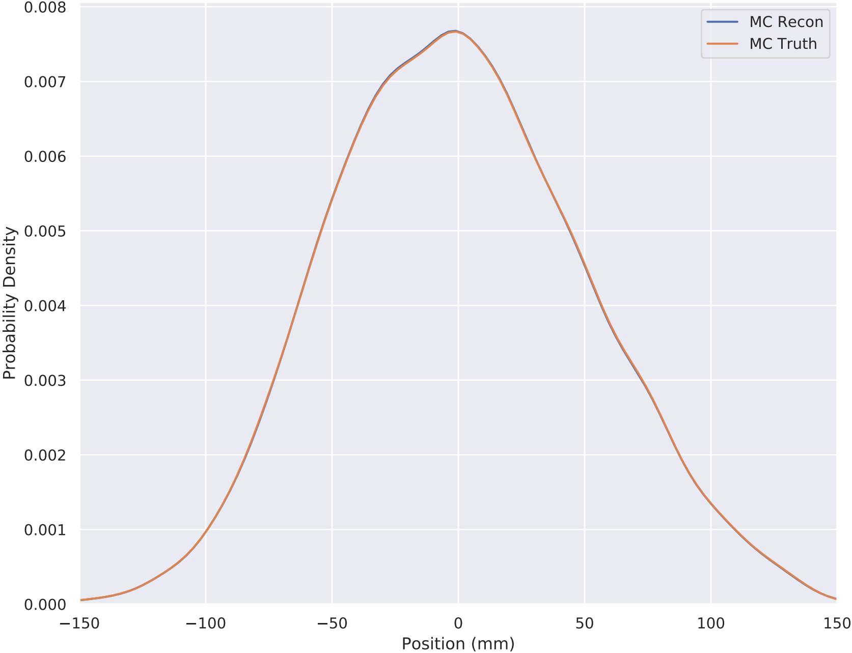
6-140 Wedge Solenoid X Position (TOF2 cut) TKD S3
