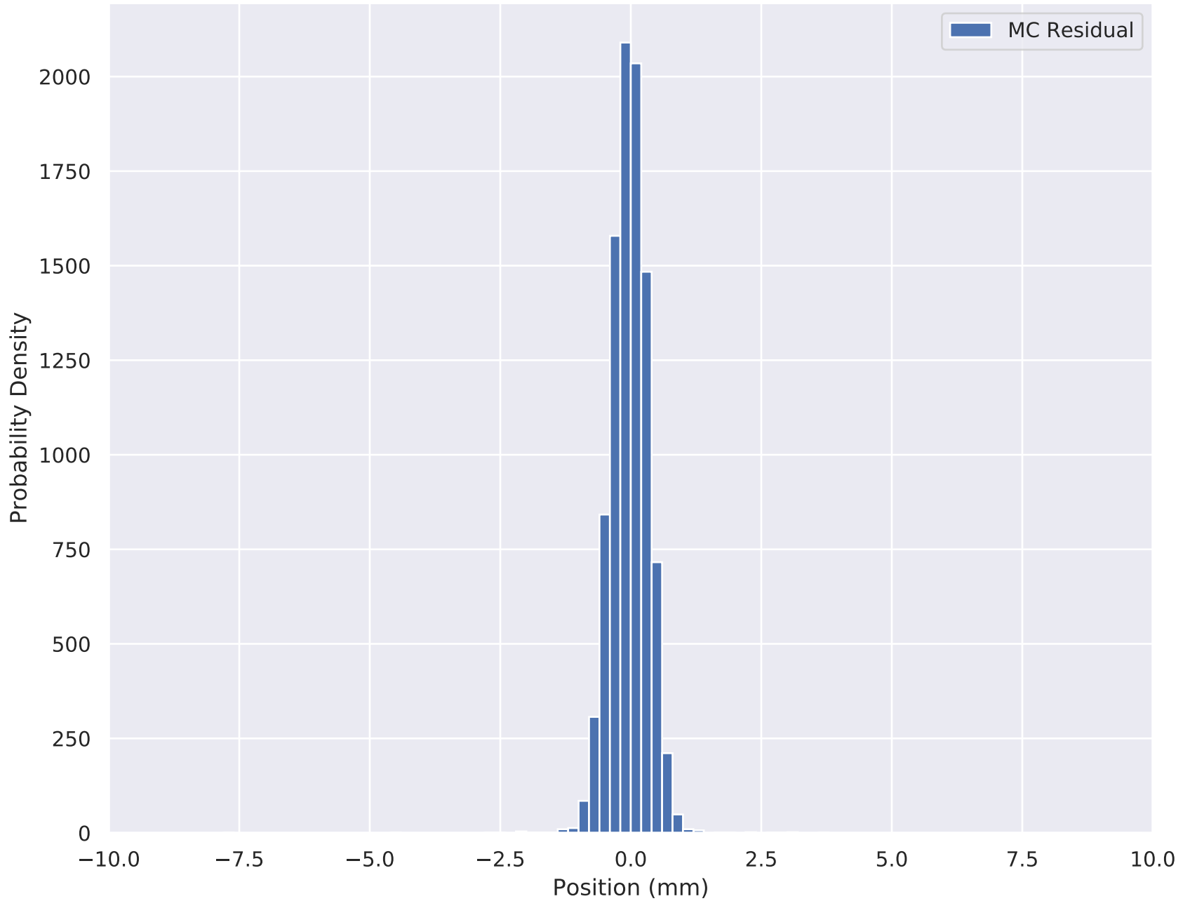
6-140 Wedge Solenoid X Residual (TOF2 cut) TKU S3
