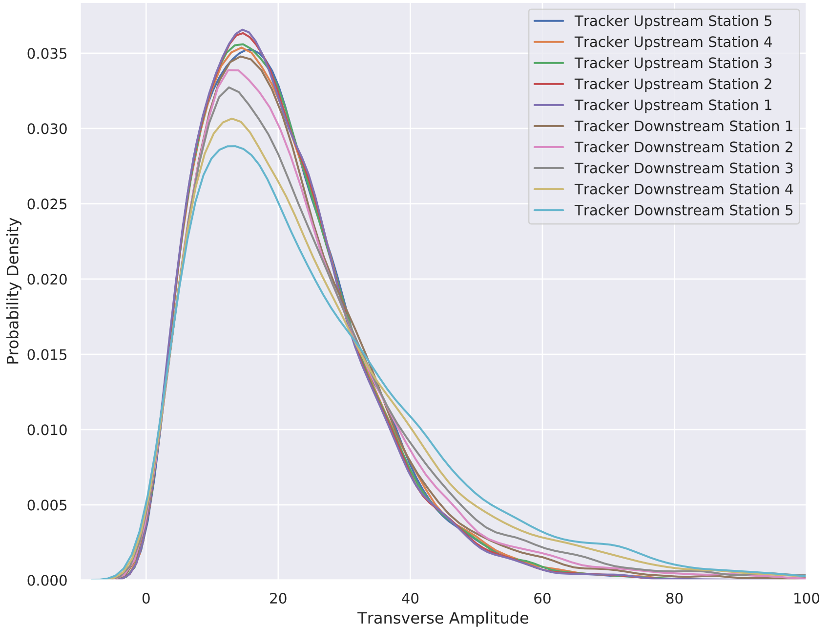
6-140 Wedge Solenoid Amplitude MC Recon (TOF2 cut)
