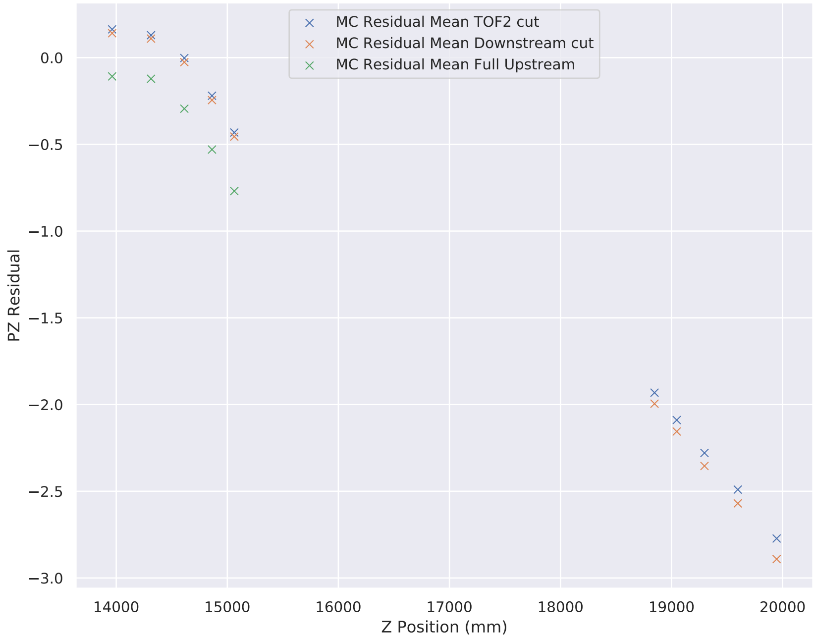
6-140 Wedge Solenoid PZ Residual Mean
