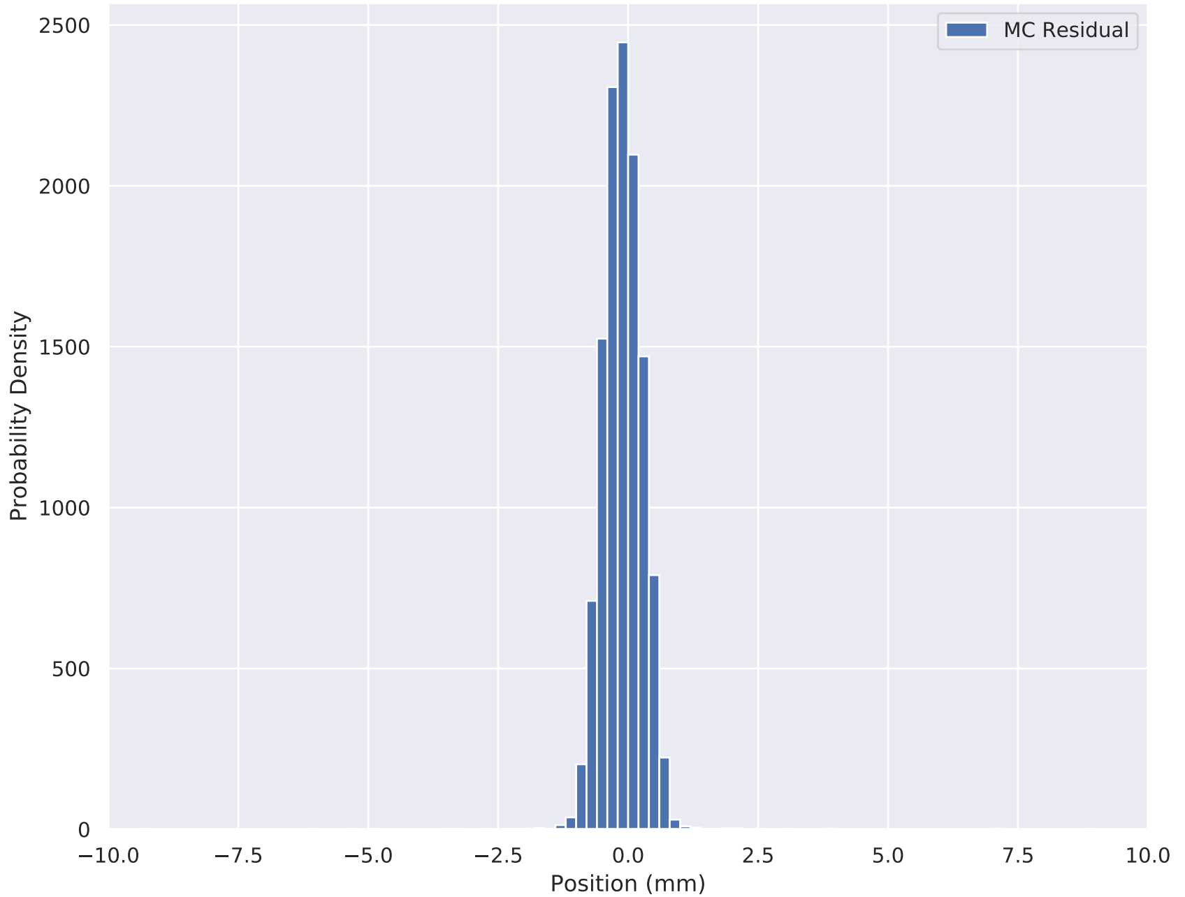
6-140 Wedge Solenoid X Residual (Downstream cut) TKU S1
