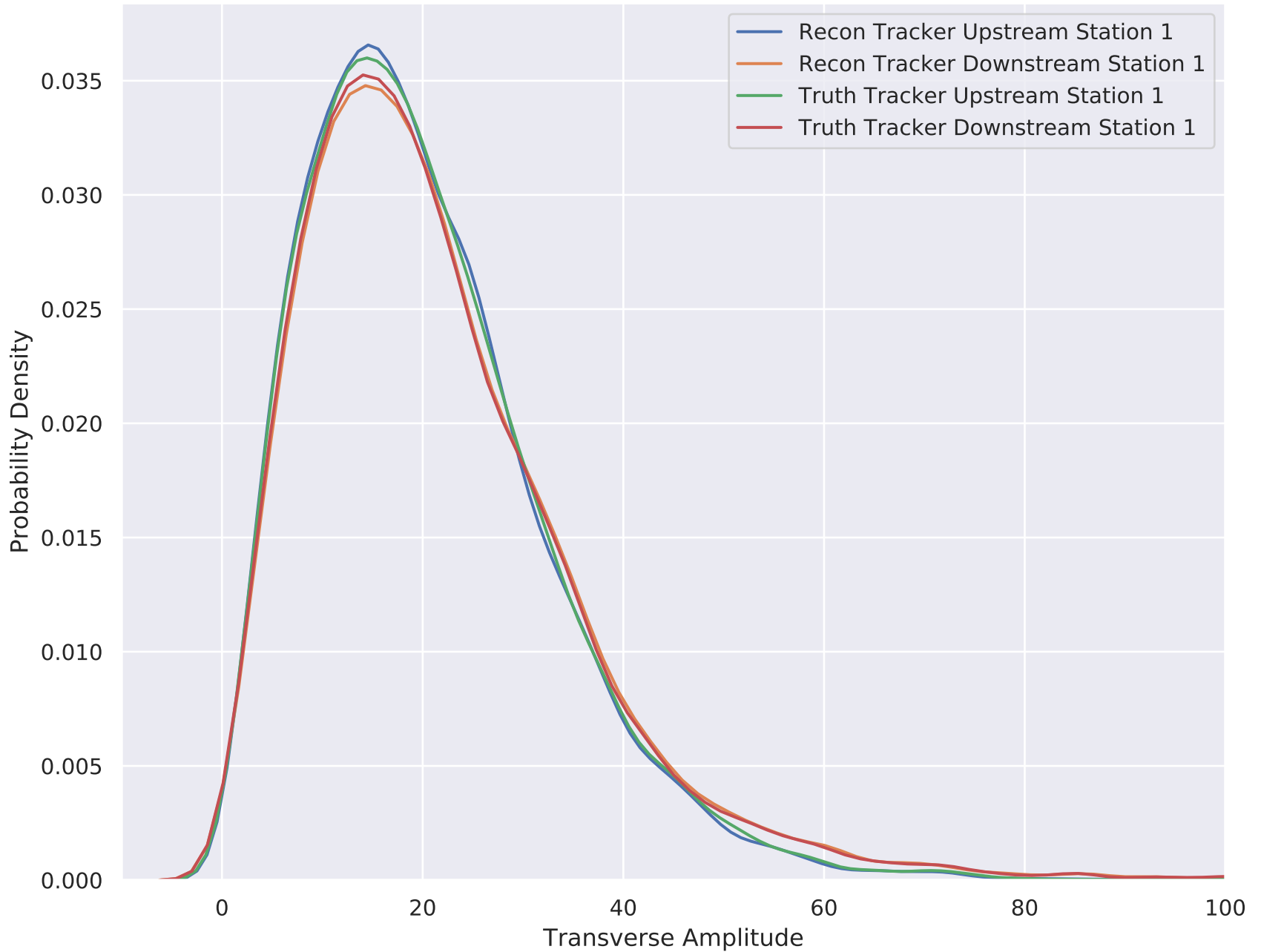
6-140 Wedge Solenoid Amplitude MC (TOF2 cut)
