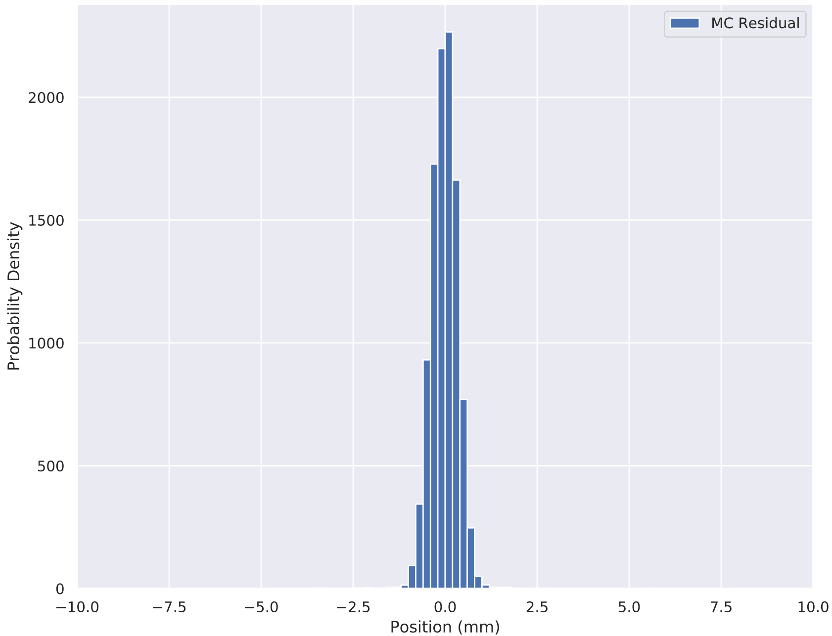
6-140 Wedge Solenoid X Residual (TOF2 cut) TKU S3
