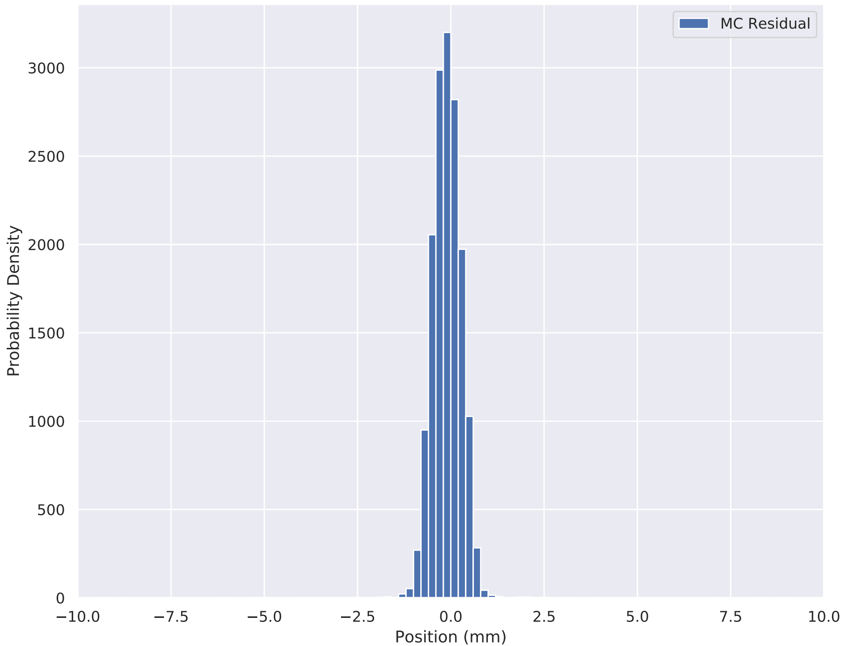
6-140 Wedge Solenoid X Residual (Full Upstream) TKU S1
