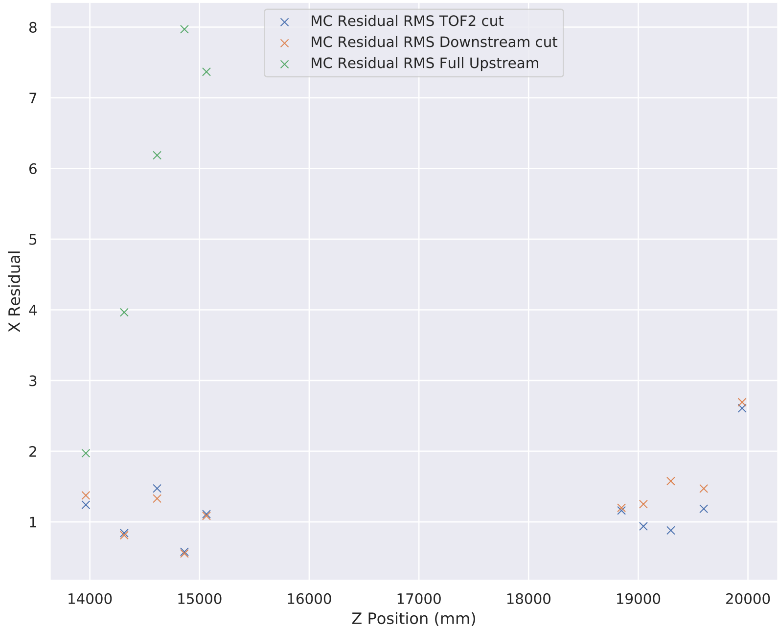
6-140 Wedge Solenoid X Residual RMS
