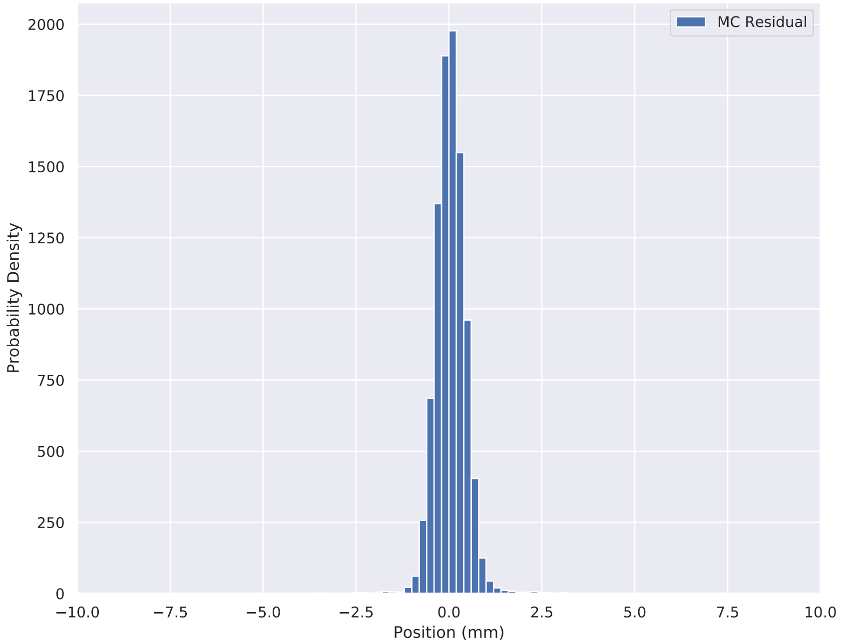
6-140 Wedge Solenoid X Residual (TOF2 cut) TKU S2
