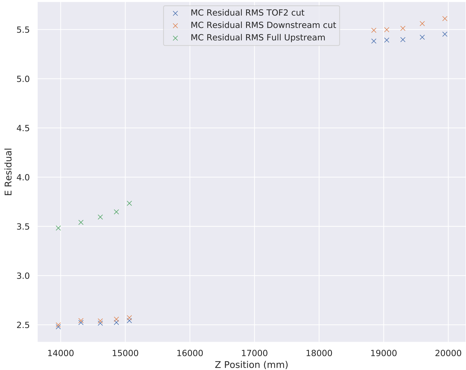
6-140 Wedge Solenoid E Residual RMS
