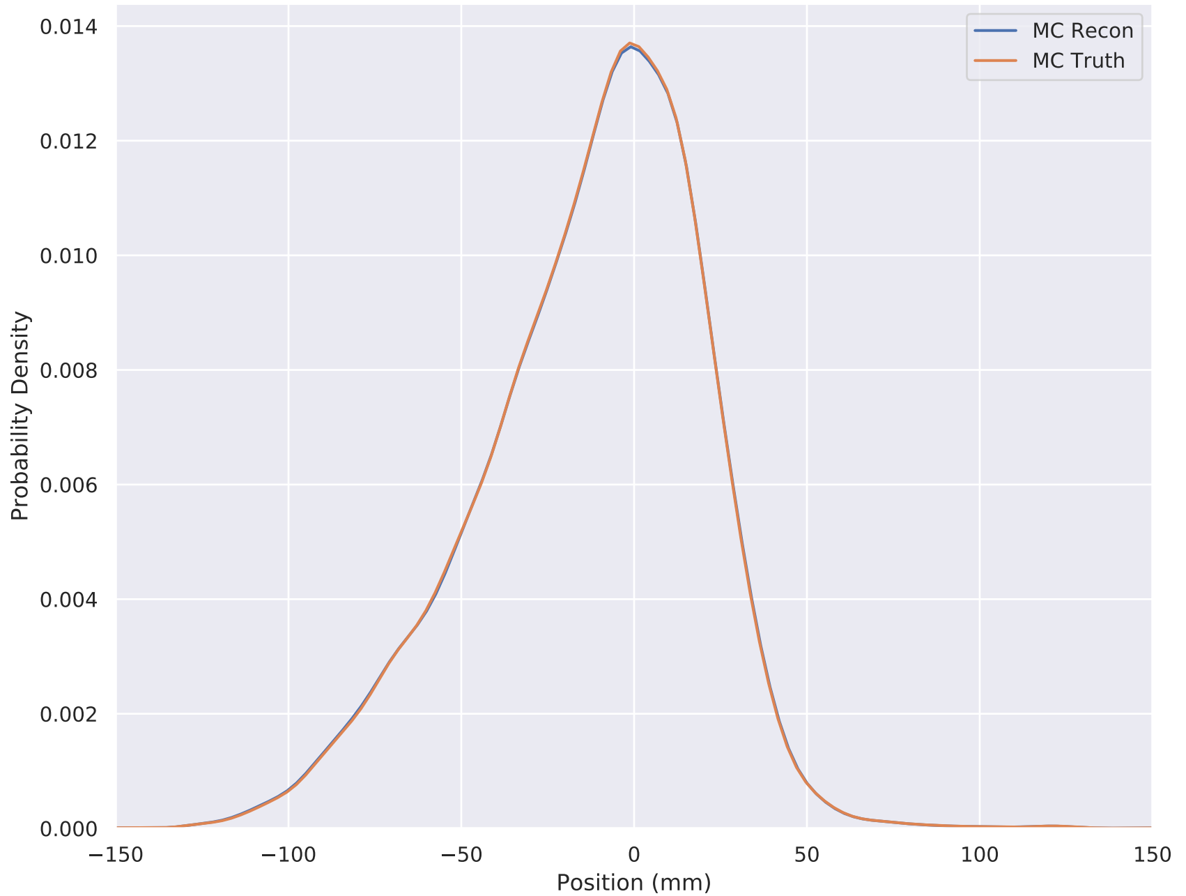
6-140 Wedge Solenoid X Position (Downstream cut) TKD S1
