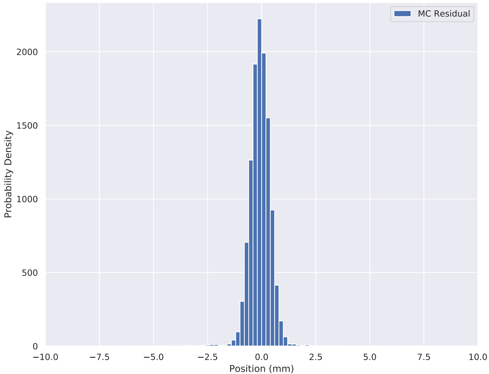
6-140 Wedge Solenoid X Residual (Downstream cut) TKD S4
