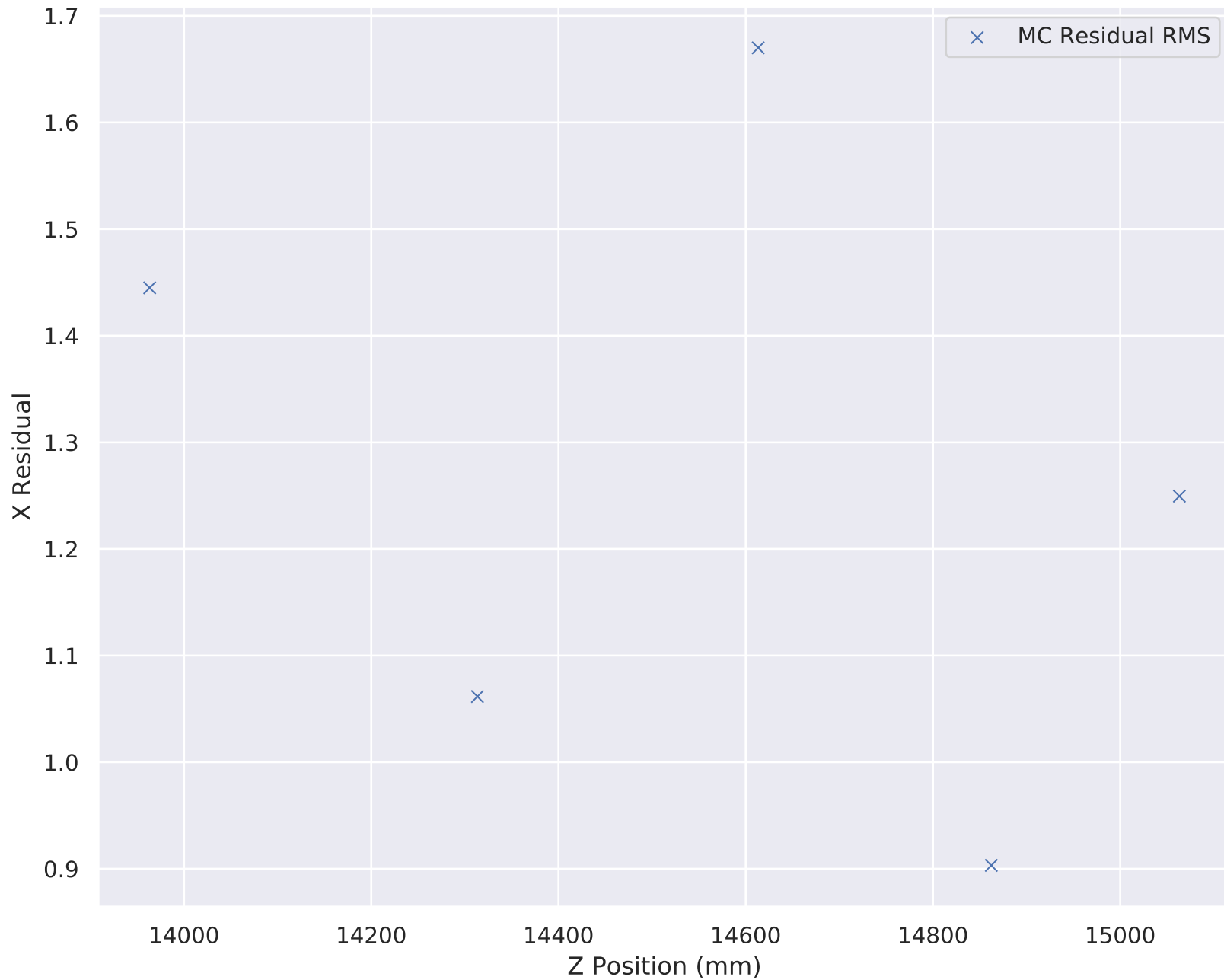
6-140 Wedge Solenoid X Residual RMS (Full Upstream)
