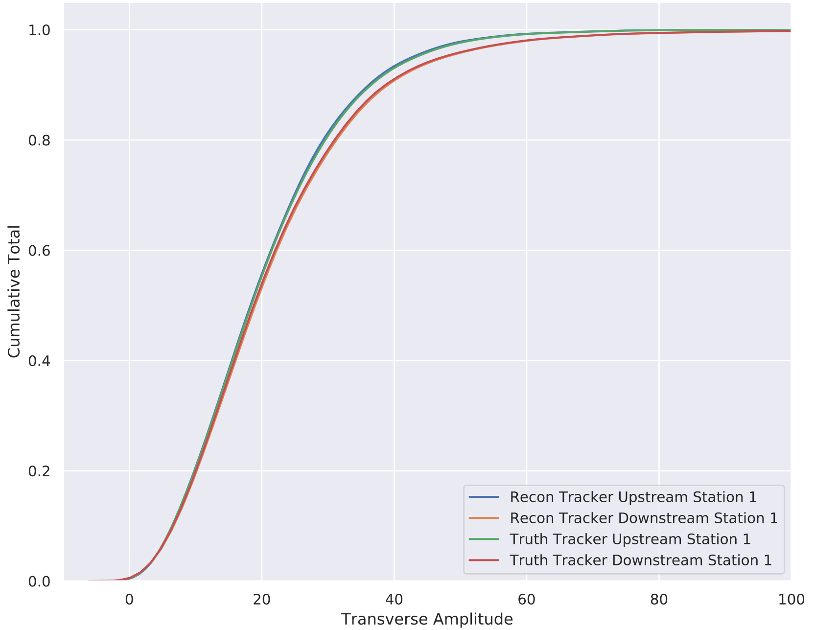
6-140 Wedge Solenoid Amplitude MC (TOF2 cut)
