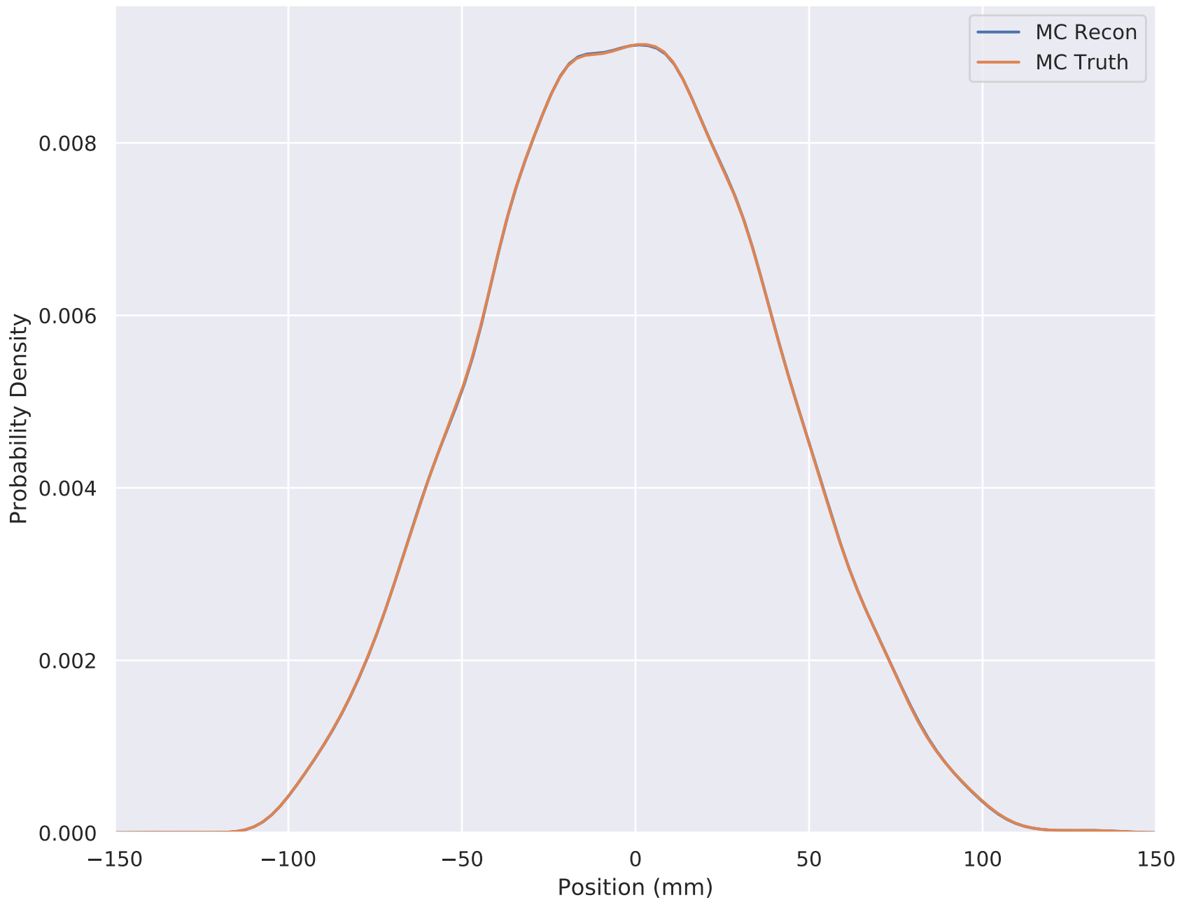
6-140 Wedge Solenoid X Position (Full Upstream) TKU S3
