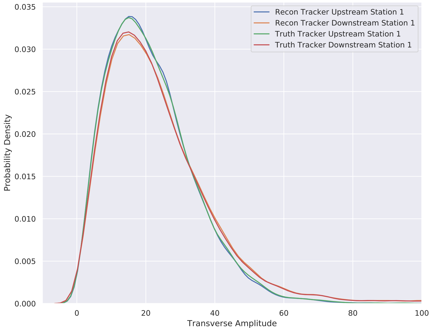
6-140 Wedge Solenoid Amplitude MC (Downstream cut)
