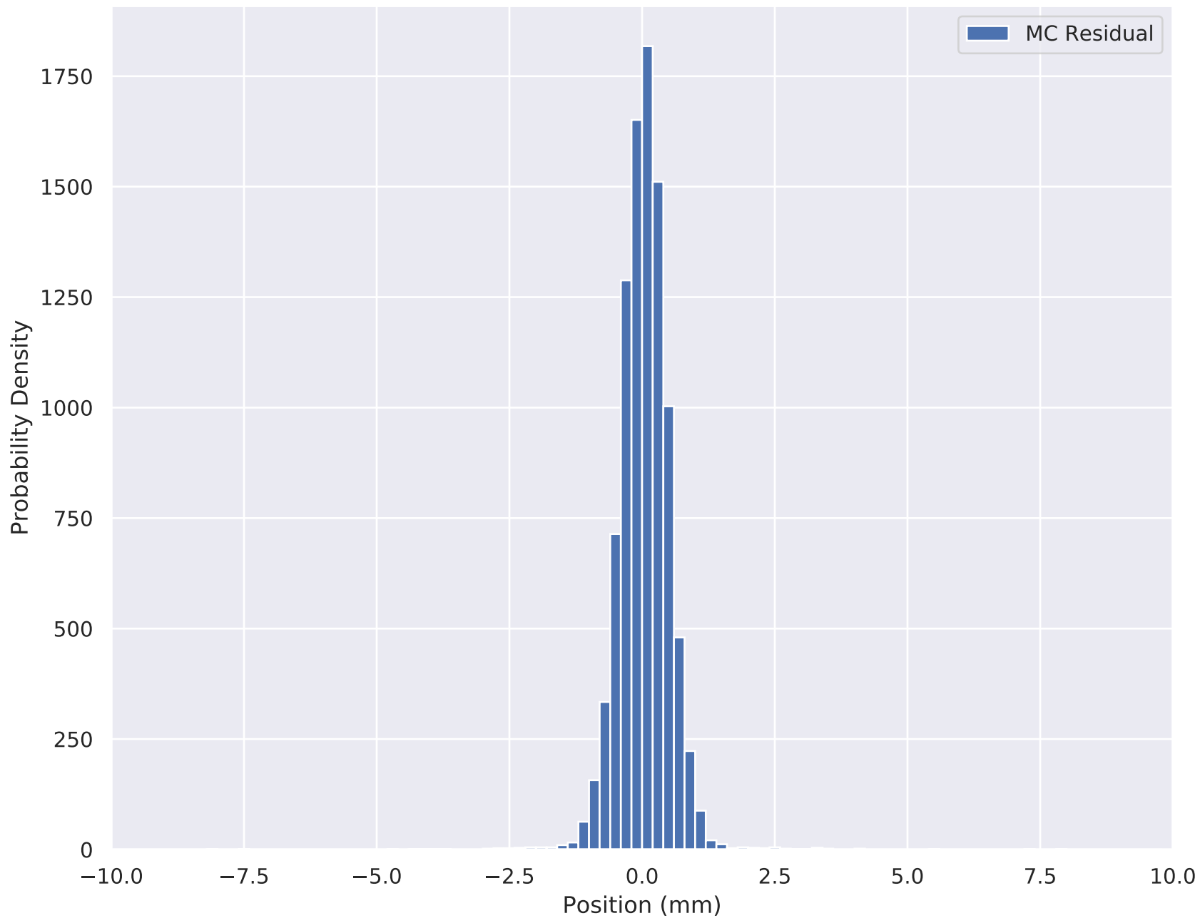
6-140 Wedge Solenoid X Residual (TOF2 cut) TKD S2
