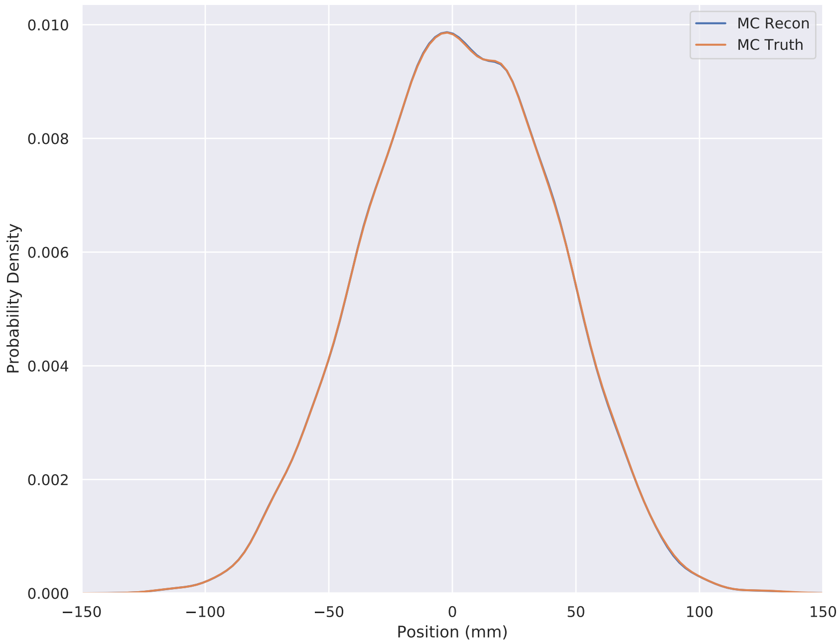
6-140 Wedge Solenoid X Position (Full Upstream) TKU S2
