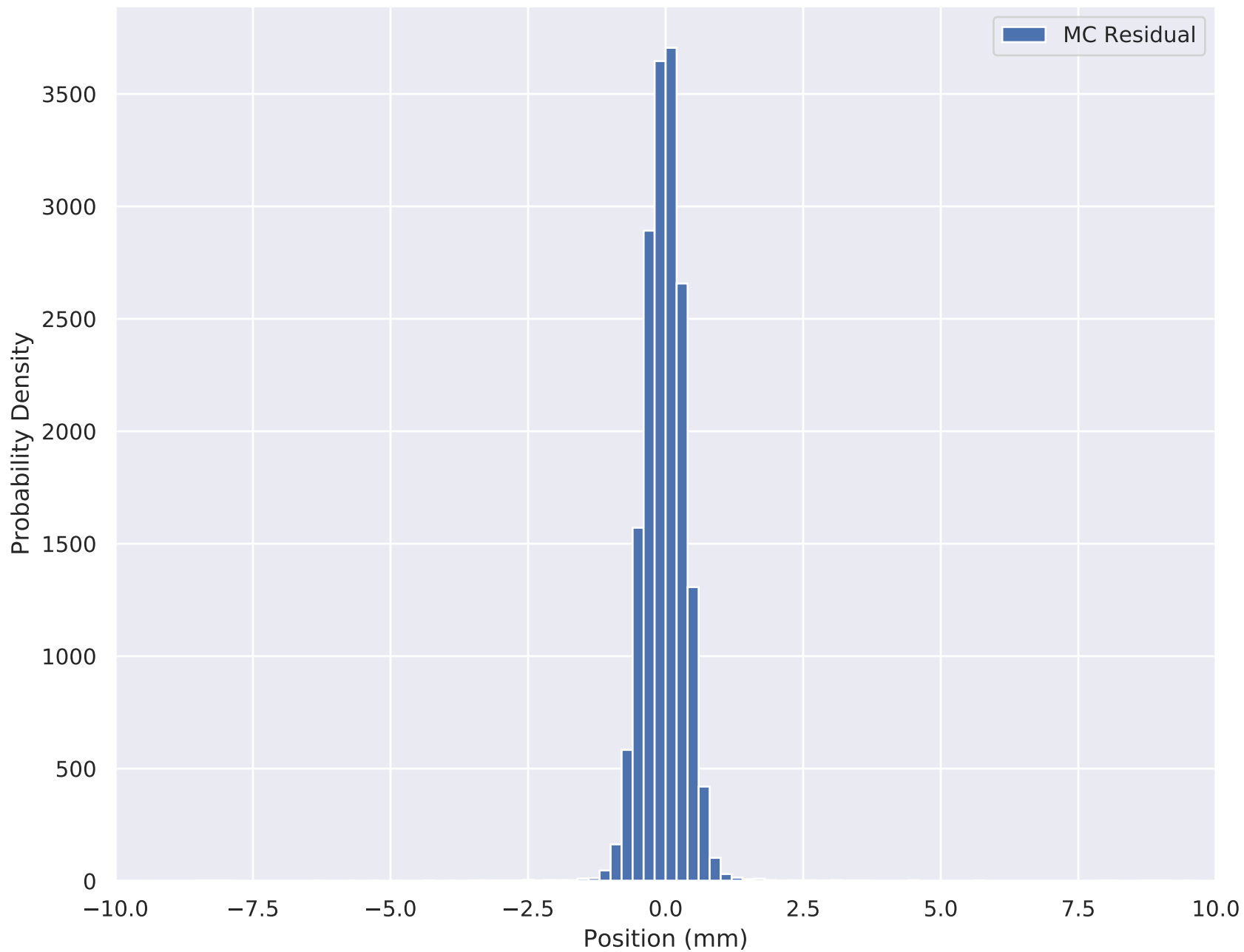
6-140 Wedge Solenoid X Residual (Full Upstream) TKU S3
