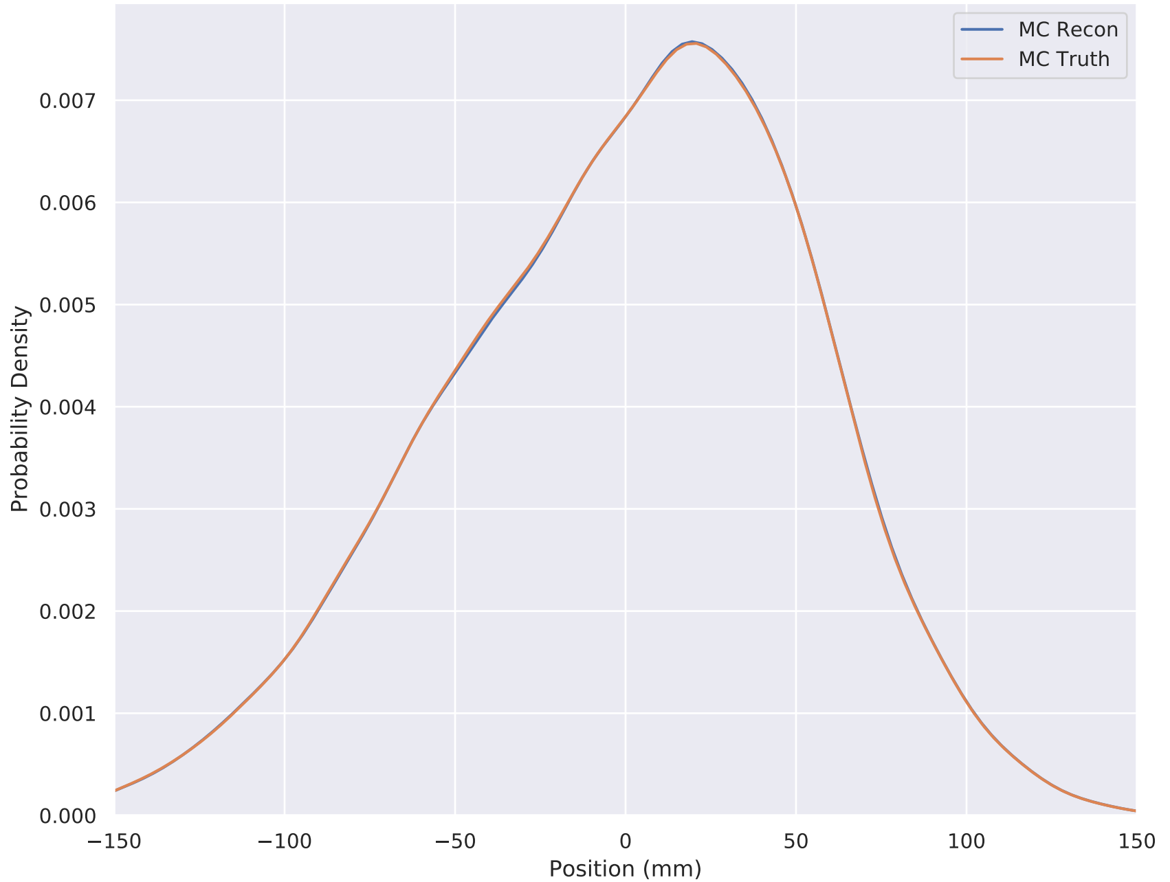
6-140 Wedge Solenoid X Position (TOF2 cut) TKD S4
