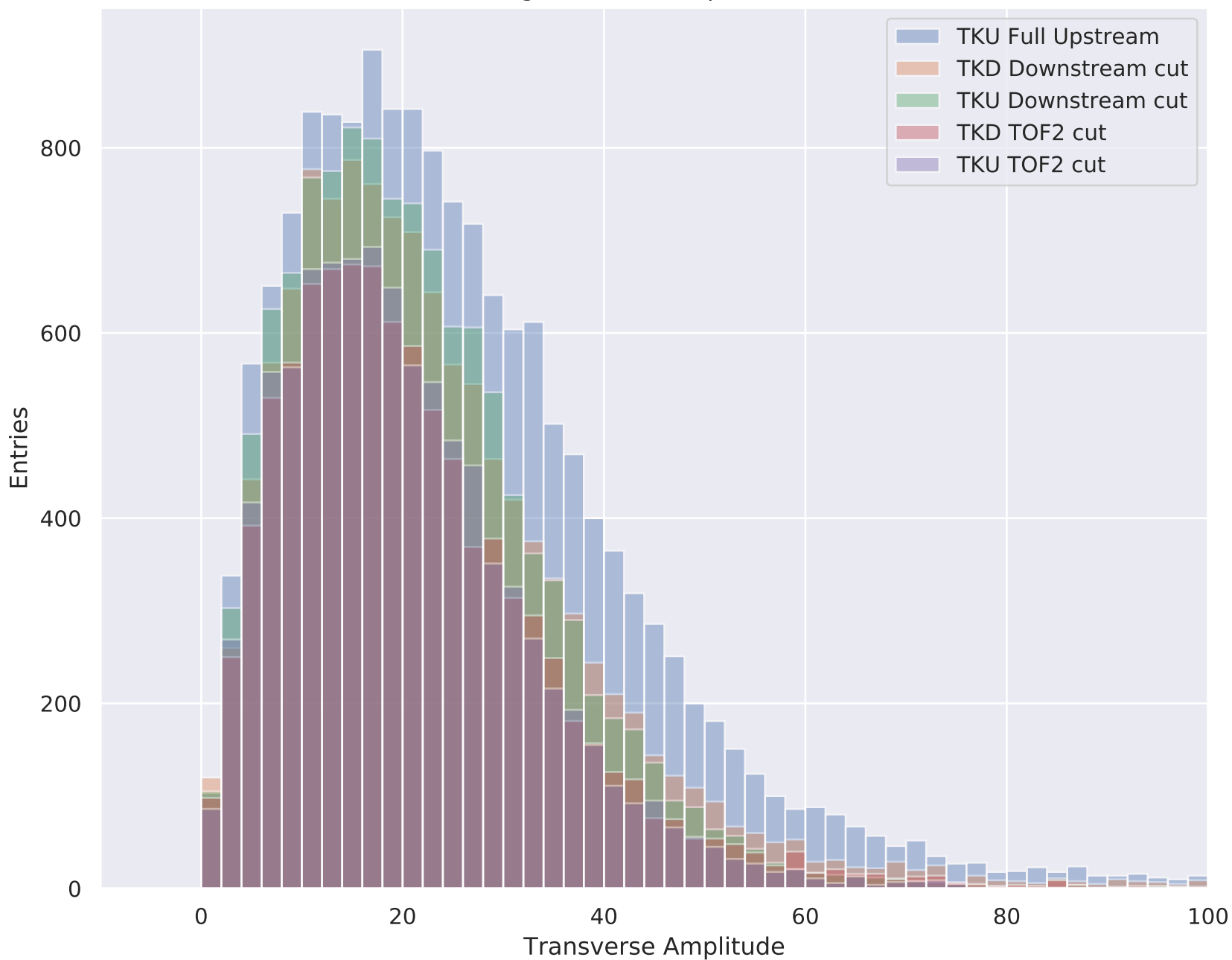
6-140 Wedge Solenoid Amplitudes MC Truth
