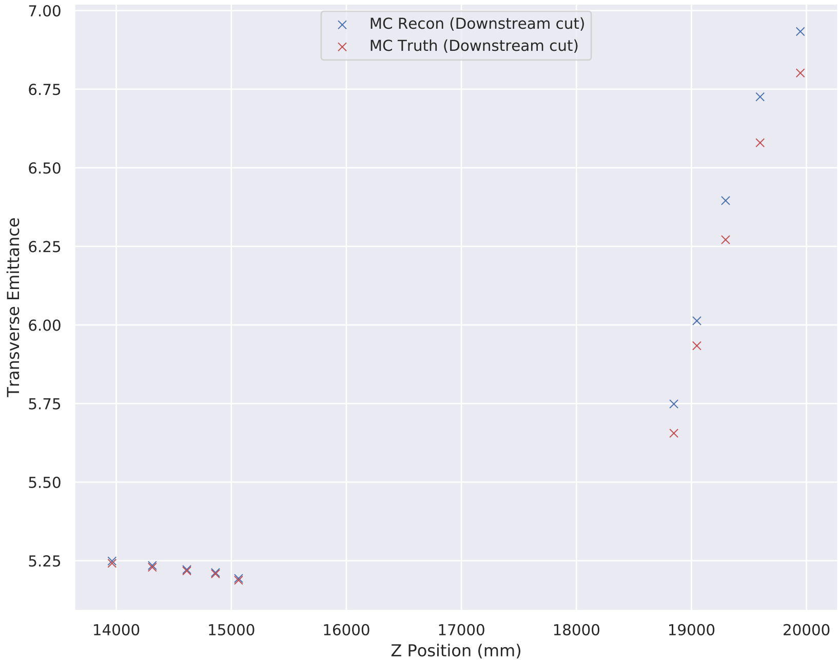
6-140 Wedge Solenoid Transverse Emittance (Downstream cut)
