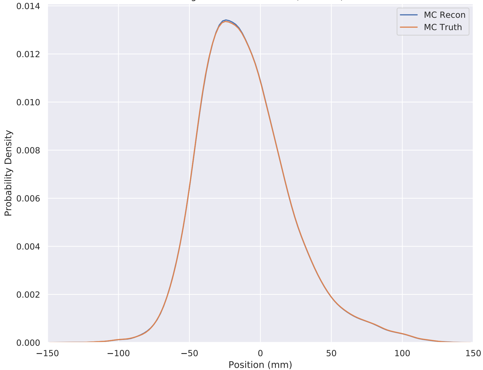
6-140 Wedge Solenoid X Position (TOF2 cut) TKD S2
