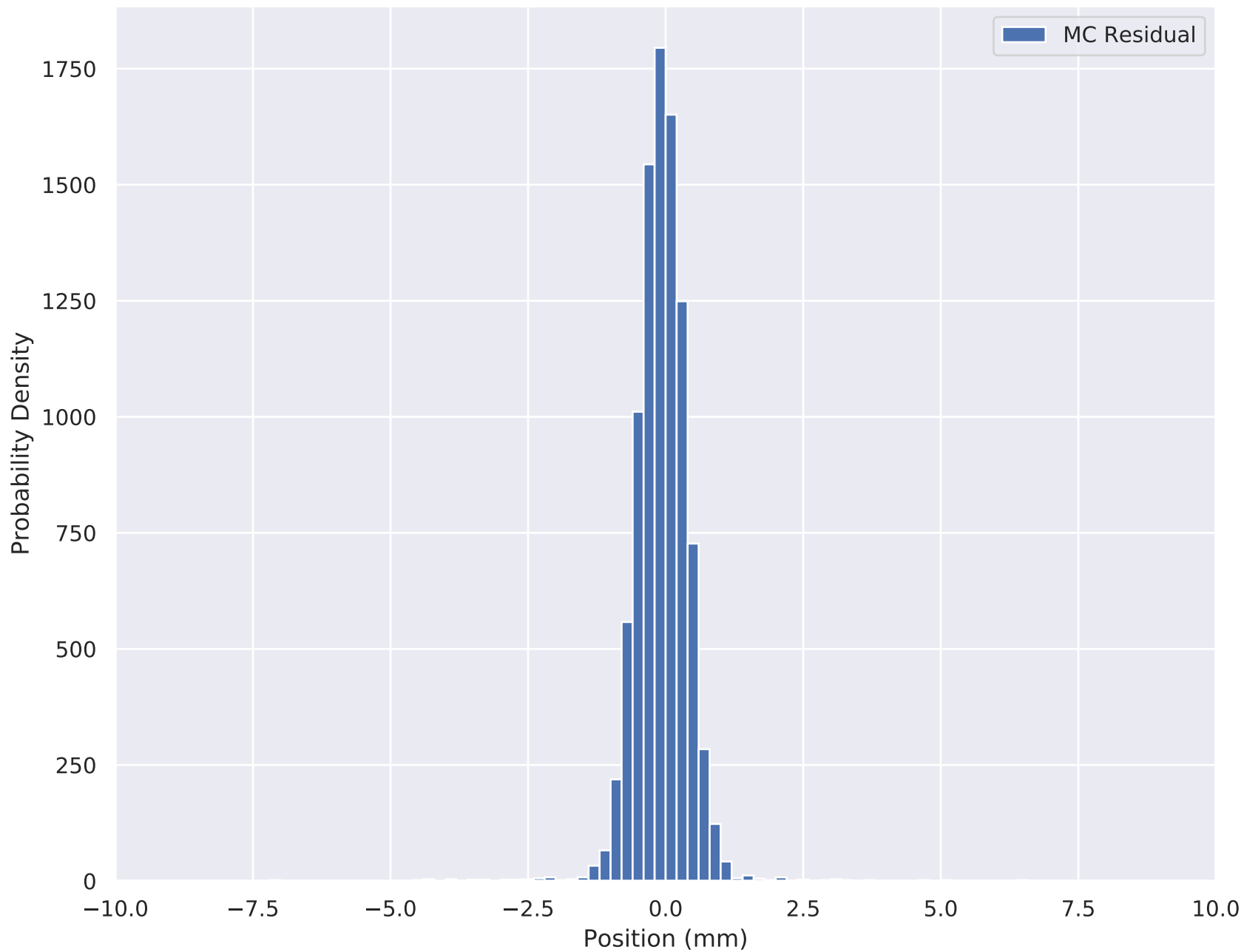
6-140 Wedge Solenoid X Residual (TOF2 cut) TKD S4
