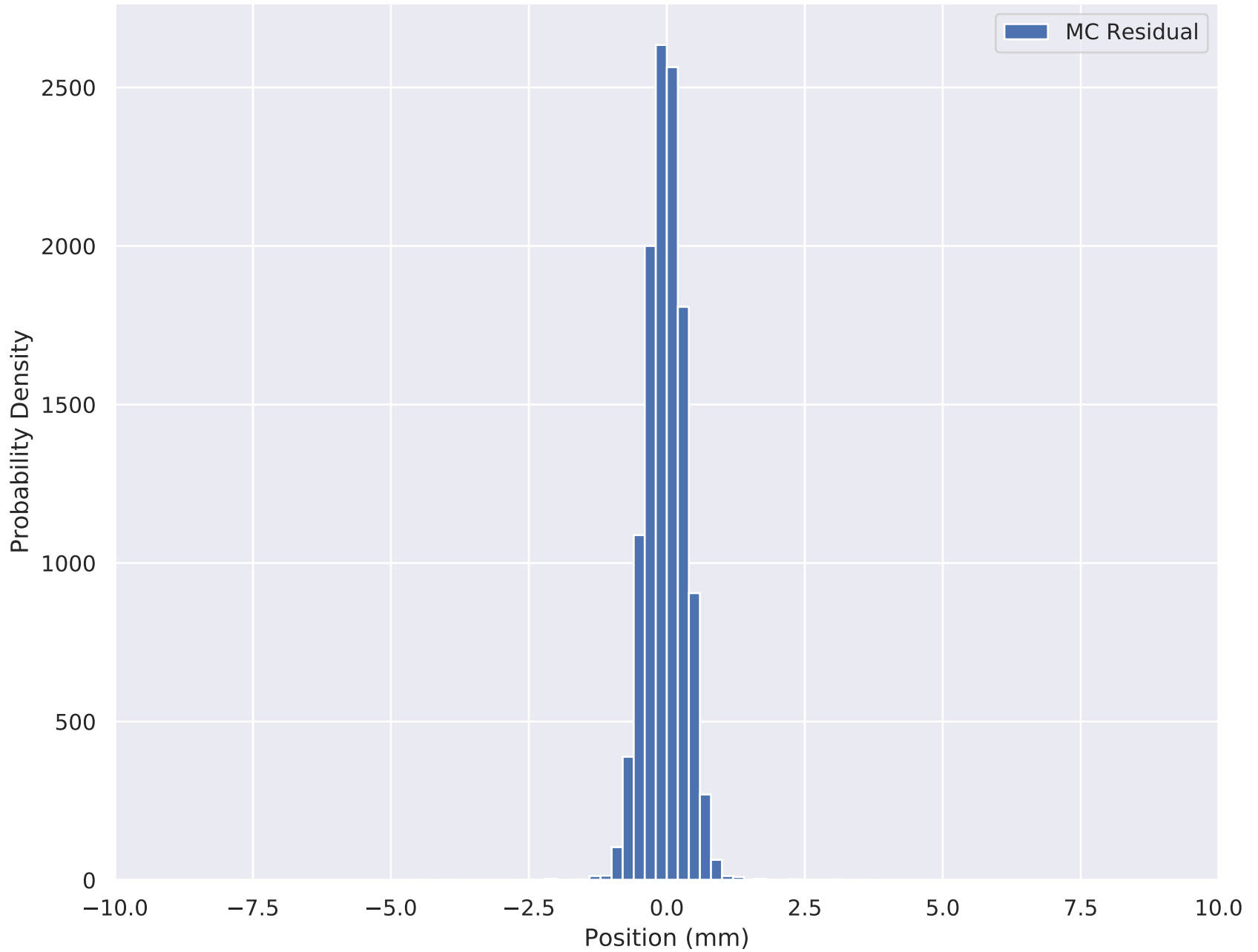
6-140 Wedge Solenoid X Residual (Downstream cut) TKU S3
