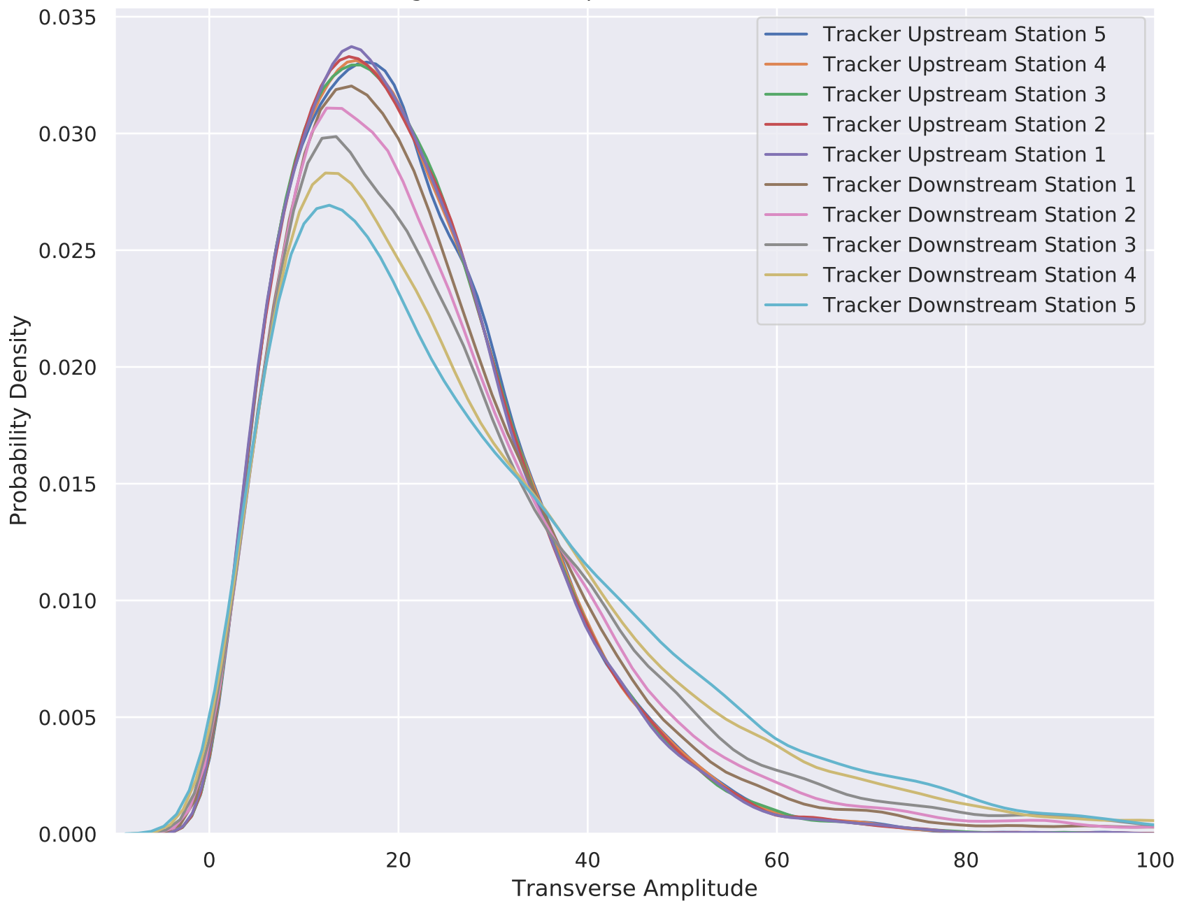
6-140 Wedge Solenoid Amplitude MC Truth (Downstream cut)
