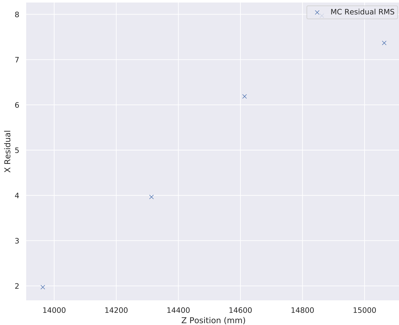
6-140 Wedge Solenoid X Residual RMS (Full Upstream)
