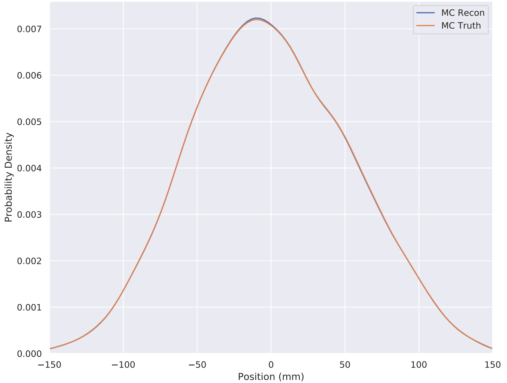
6-140 Wedge Solenoid X Position (Downstream cut) TKD S3
