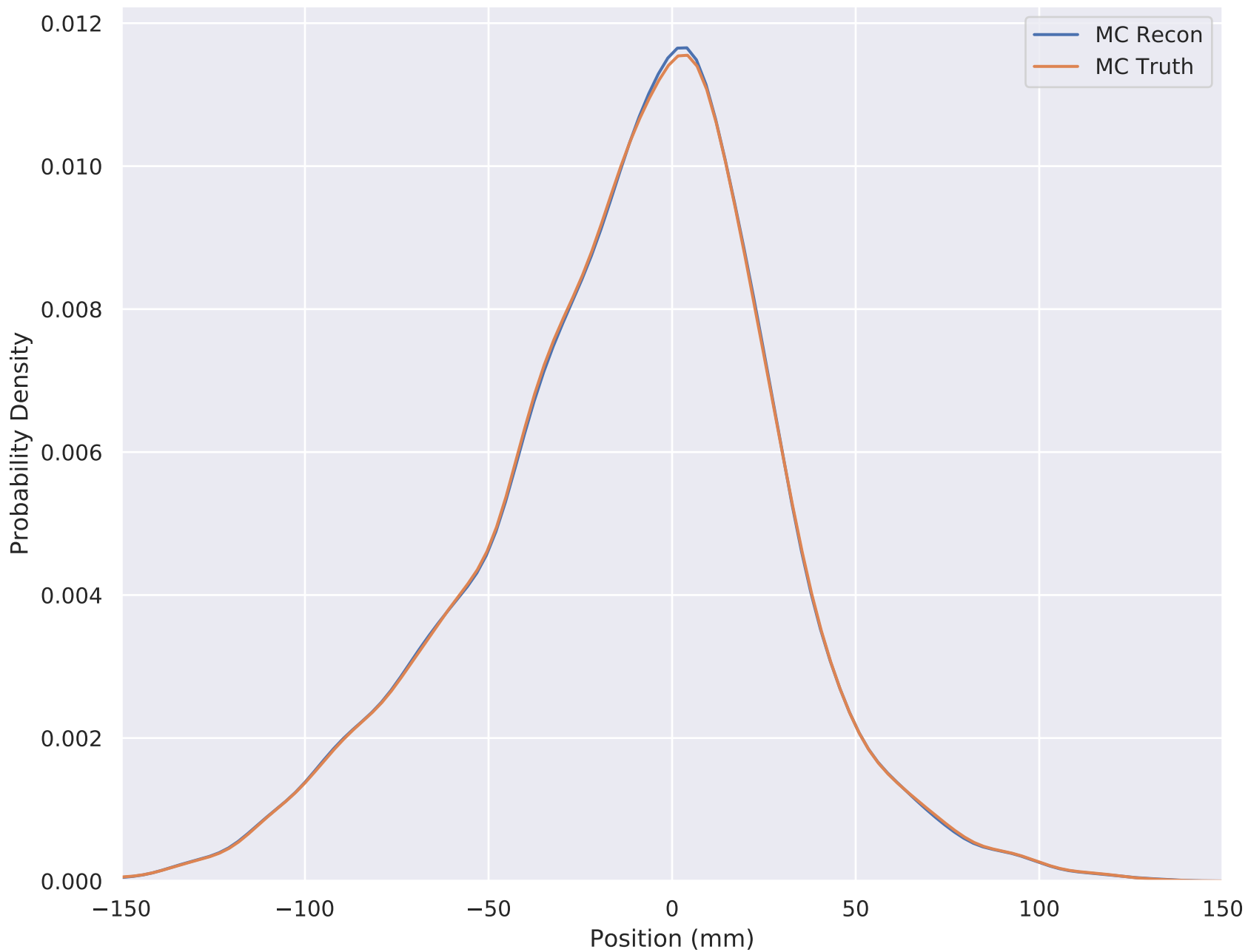
6-140 Wedge Solenoid X Position (TOF2 cut) TKD S5
