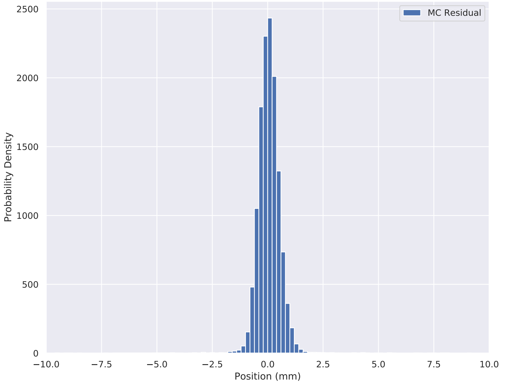
6-140 Wedge Solenoid X Residual (Downstream cut) TKD S3
