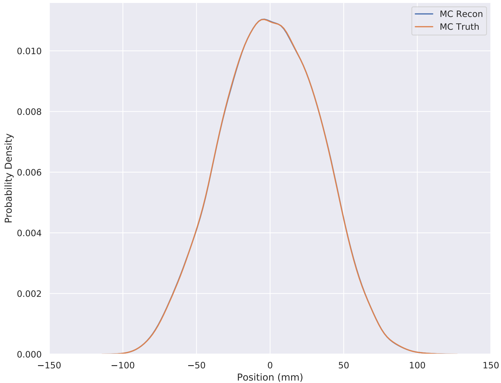
6-140 Wedge Solenoid X Position (TOF2 cut) TKU S5
