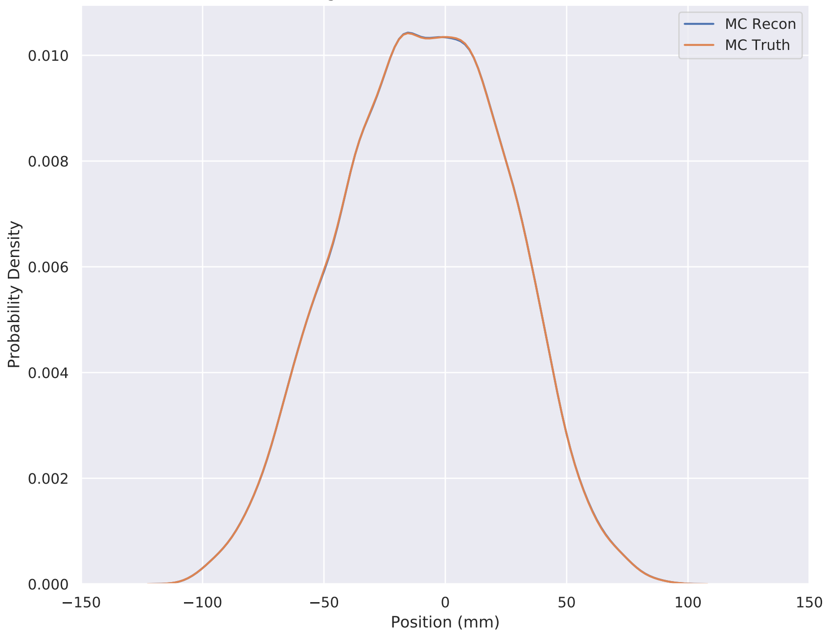
6-140 Wedge Solenoid X Position (TOF2 cut) TKU S3
