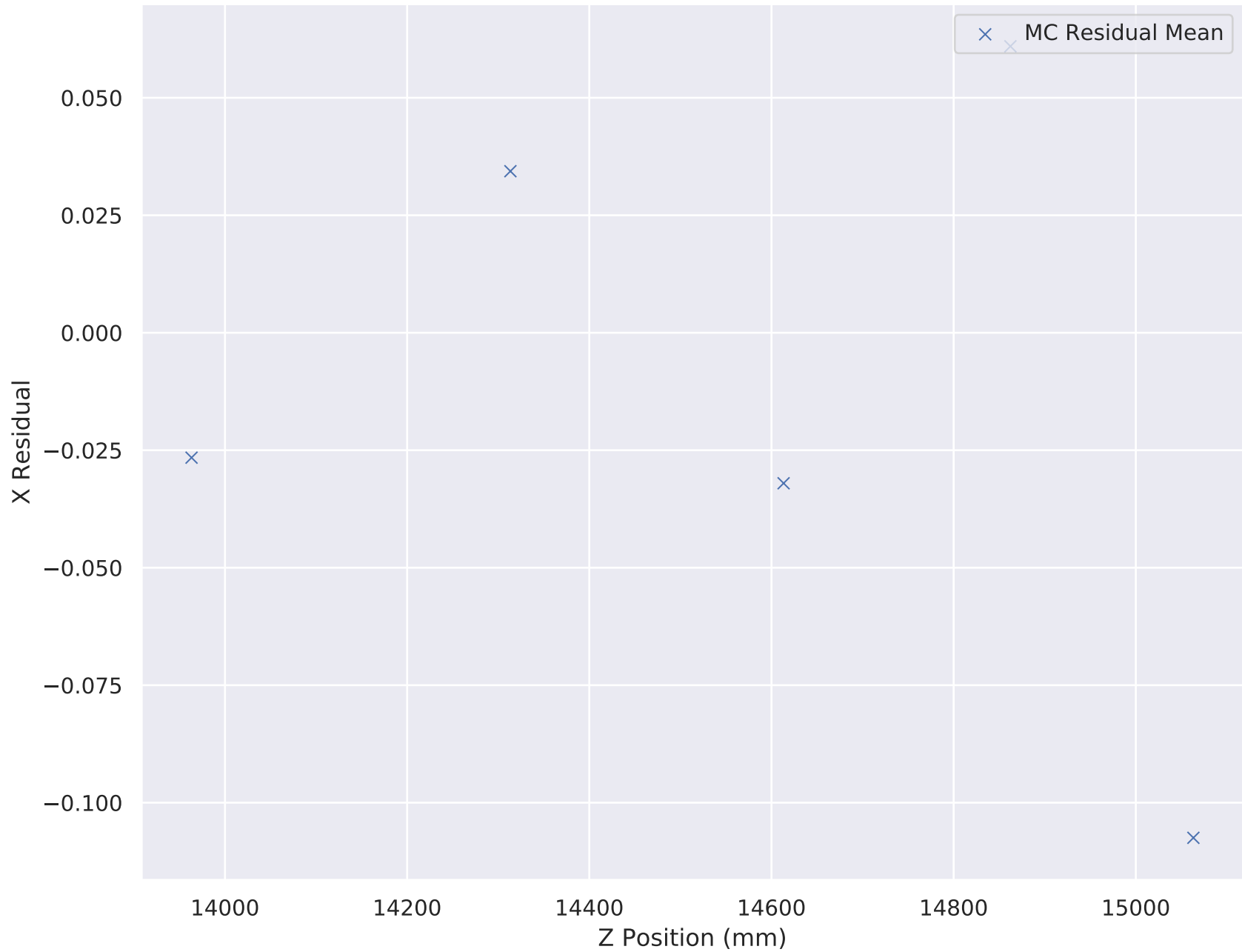
6-140 Wedge Solenoid X Residual Mean (Full Upstream)
