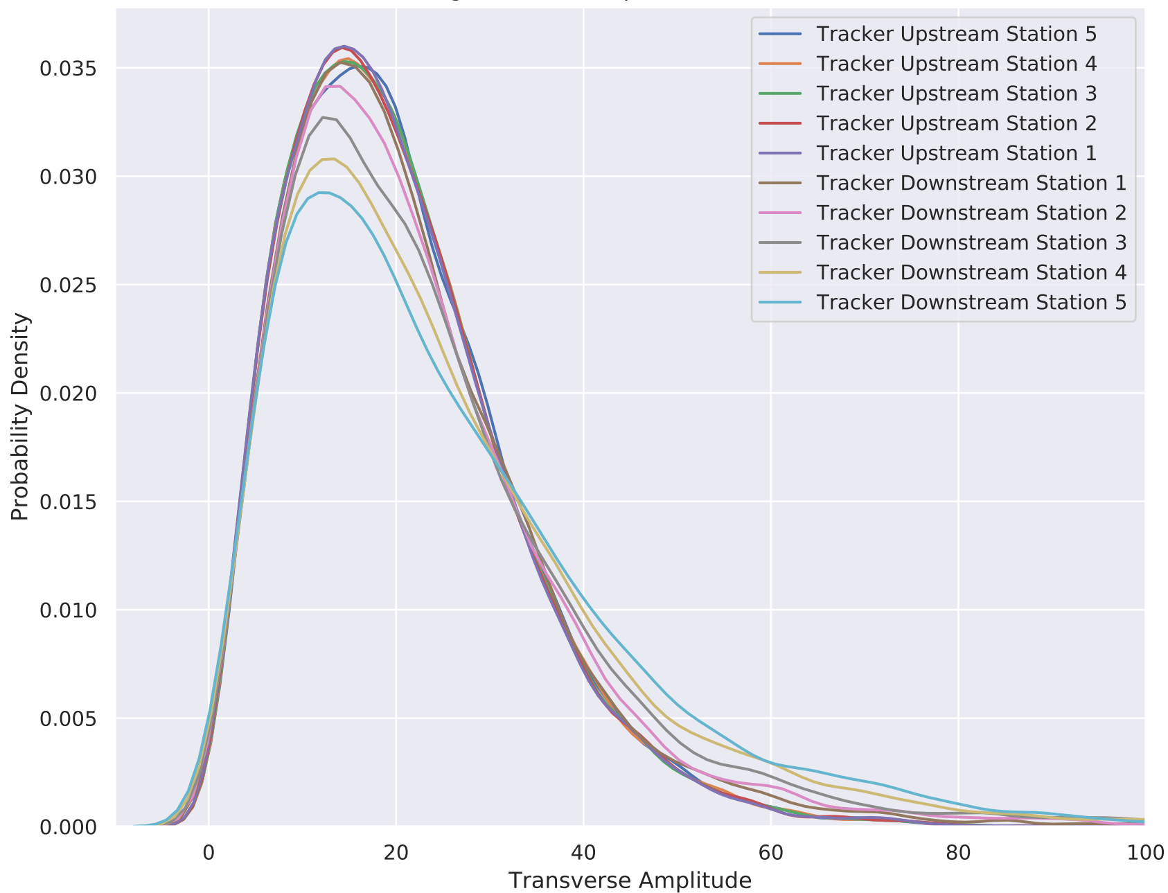
6-140 Wedge Solenoid Amplitude MC Truth (TOF2 cut)
