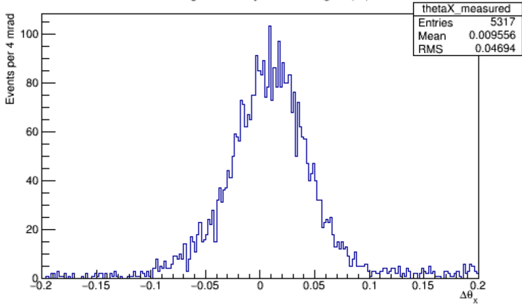
Change in Projected Angle (X)
