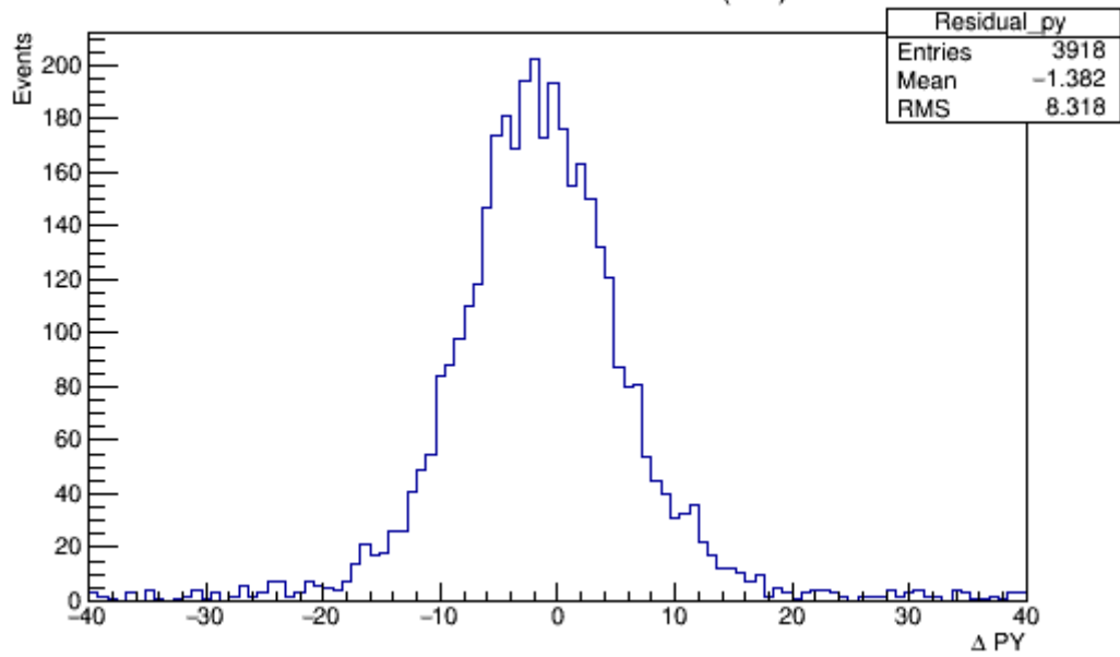
Difference in Momentum (PY)
