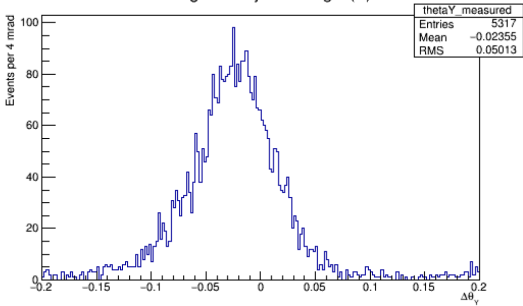
Change in Projected Angle (Y)
