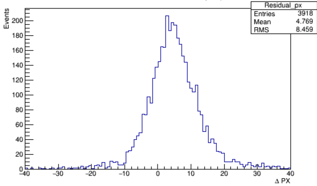
Difference in Momentum (PX)
