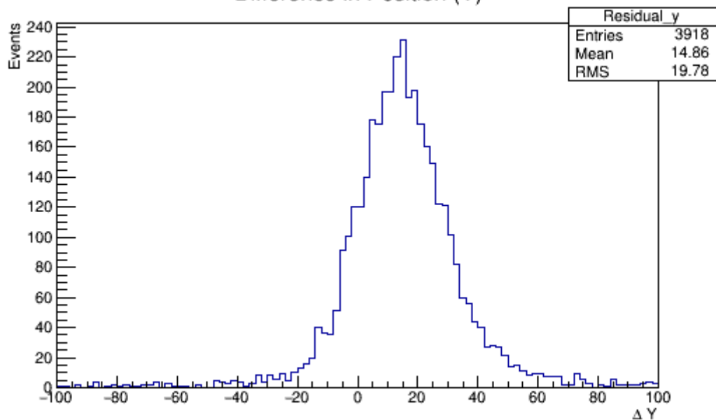
Difference in Position (Y)
