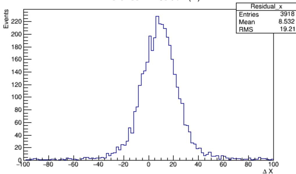
Difference in Position (X)
