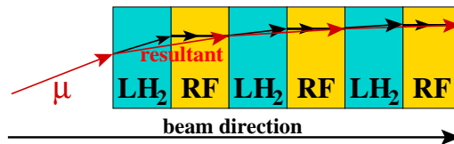
Figure 1: Ionization cooling: Muons traverse the absorber losing energy via dE/dx , and RF replaces longitudinal component of momentum.
