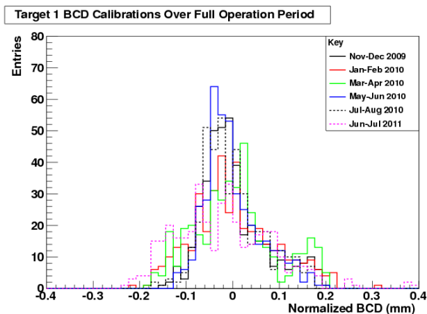
Figure 1: The spread of beam-centre distance (BCD) at maximum depth for target calibrations throughout running of the present target in ISIS.
