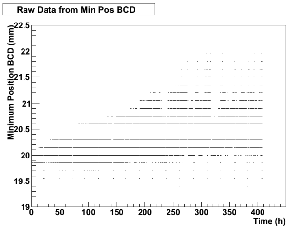
Figure 3: Minimum target distance from beam centre over a prolonged run. 420 hours corresponds to \sim 1.1 M cycles. Note the variation of \sim 1 mm is small compared with both the strike of \sim 44 mm and fluctuations in ISIS beam size.
