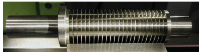
Figure 4: The new former for the target. Each coil will be wound directly onto the former, improving alignment and cooling of the magnetic assembly.
