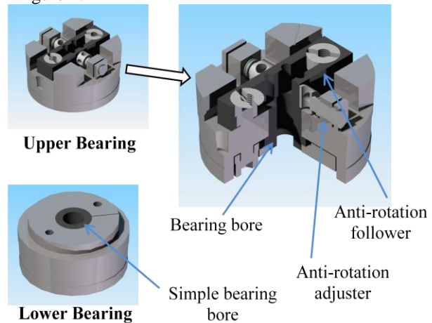
Figure 2: Upper and lower bearings, showing the VESPEL ® inserts.
