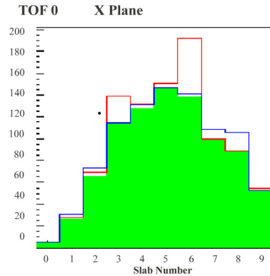
Figure 4: Histogram showing the slab hits due to PMT coincidence (green), as well as the TDC signals for PMT0 (red) and PMT1 (blue) for all slabs in the x plane of TOF0.
