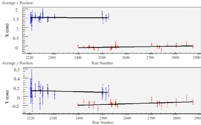
Figure 2: Average x (top) and y (bottom) beam position for TOF0. Blue indicates negative polarity beam line and red indicates positive polarity.
