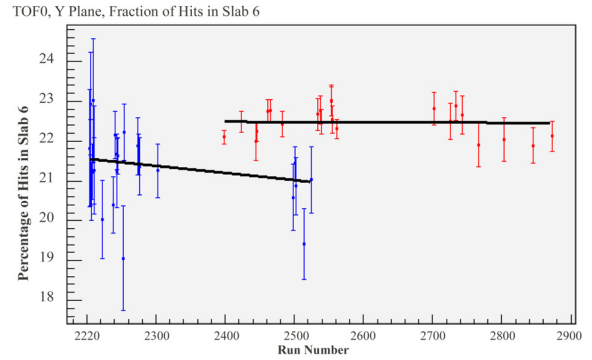
Figure 3: The percentage of all the hits in the TOF0 y plane that is recorded in slab 6. Blue corresponds to negative polarity runs; red corresponds to positive polarity.
