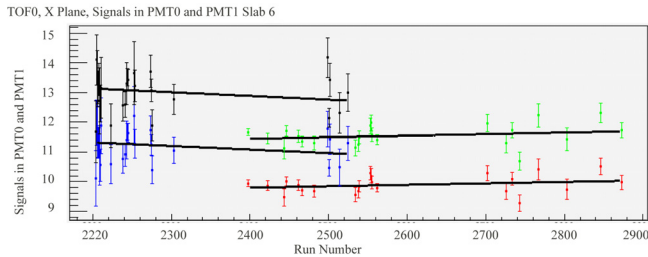
Figure 5: The percentage of signals in PMT0 and PMT1 for slab 6 in the x plane of TOF0. Green and black correspond to PMT0 signals for positive and negative runs respectively. Red and blue correspond to PMT1 signals for positive and negative runs respectively. There is a greater difference between the number of signals in each PMT for this slab than for most others.
