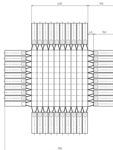
Figure 1: Schematic of TOF0. PMTs shown at either end of each strip. Coincidence between 4 PMTs (2 from each plane) is necessary for a space point[7].
