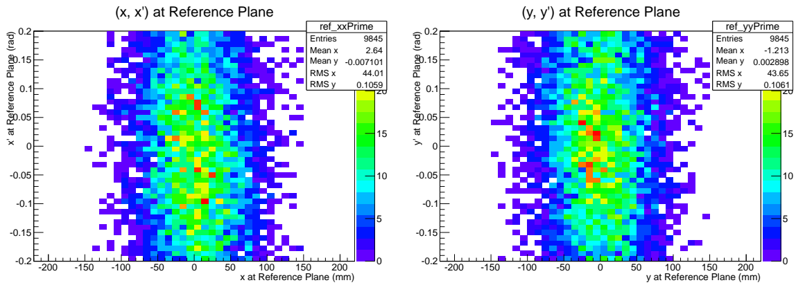
Figure 6: Transverse phase space, of an unselected beam, at the tracker reference plane. Left: Horizontal phase space, right: vertical phase space
