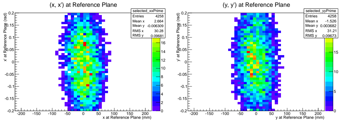
Figure 7: Transverse phase space of a selected “matched” beam at the tracker reference plane. Left: horizontal phase space, right: vertical phase space
