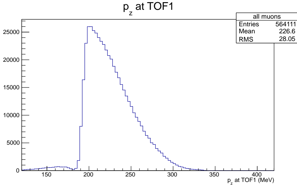
Figure 3: Longitudinal momentum distribution of all muons at TOF1, selected by time-of-flight, in the baseline beam Step I data.
