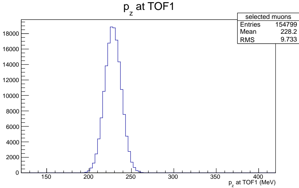
Figure 4: Longitudinal momentum distribution of muons at TOF1 after a Gaussian selection with \langle p_z \rangle = 228 \text{ MeV}/c and \sigma_{pz} = 10 \text{ MeV}/c
