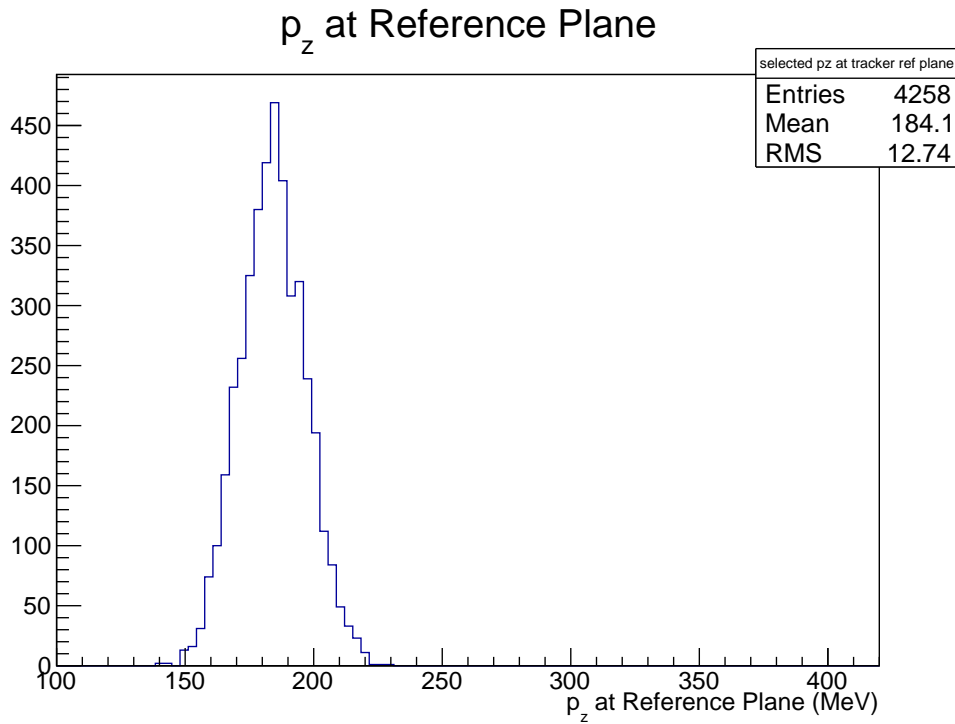
Figure 8: Longitudinal momentum distribution of a selected “matched” beam after the brass-tungsten diffuser, at the tracker reference plane.
