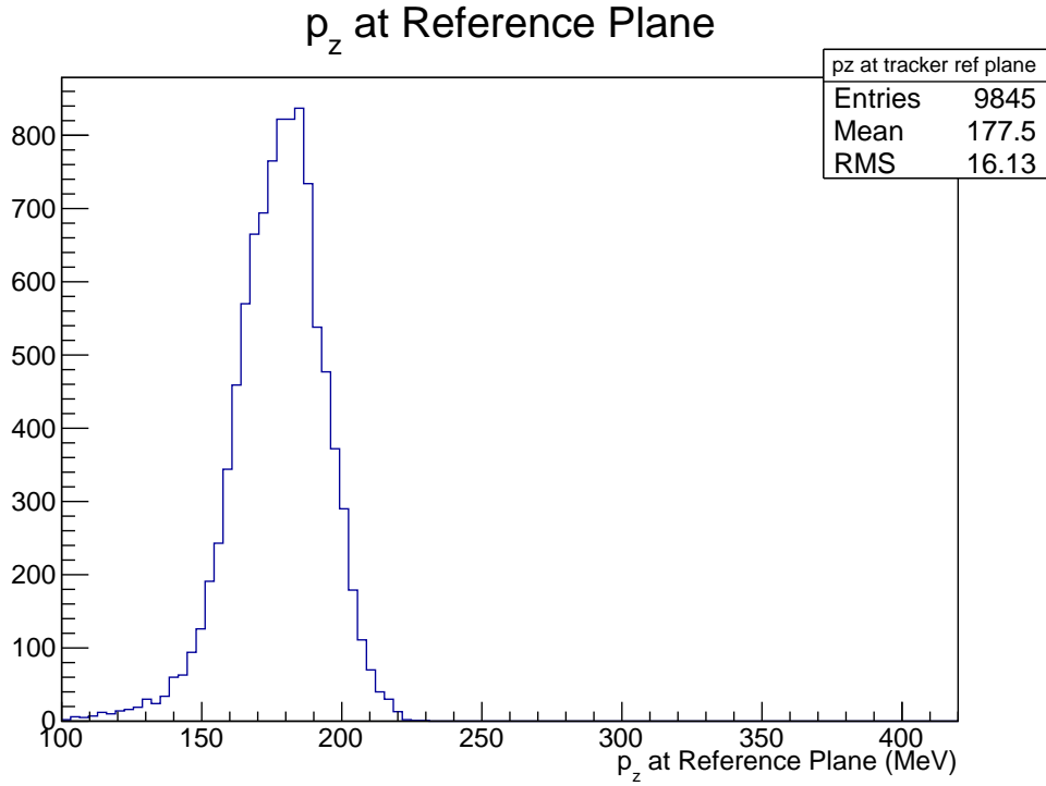
Figure 5: Longitudinal momentum distribution, after the brass-tungsten diffuser, at the tracker reference plane.
