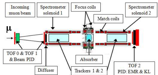
Figure 3: Step IV configuration of the MICE Experiment.
