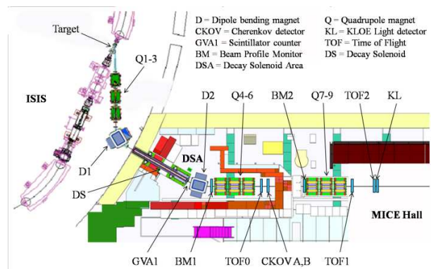
Figure 2: A schematic of the MICE beam line showing the magnetic lattice and detectors. The distance between GVA1 and TOF0 is approximately 6 meters. The proton absorbers are located just after D1 and before DS
