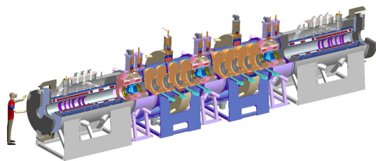
Figure 1: The MICE cooling channel and spectrometers
