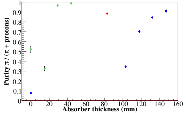
Figure 5: The purity of the beam as a function of absorber thickness for the 140 (green), 200 (red) and 240 (blue) MeV/c beam line settings
