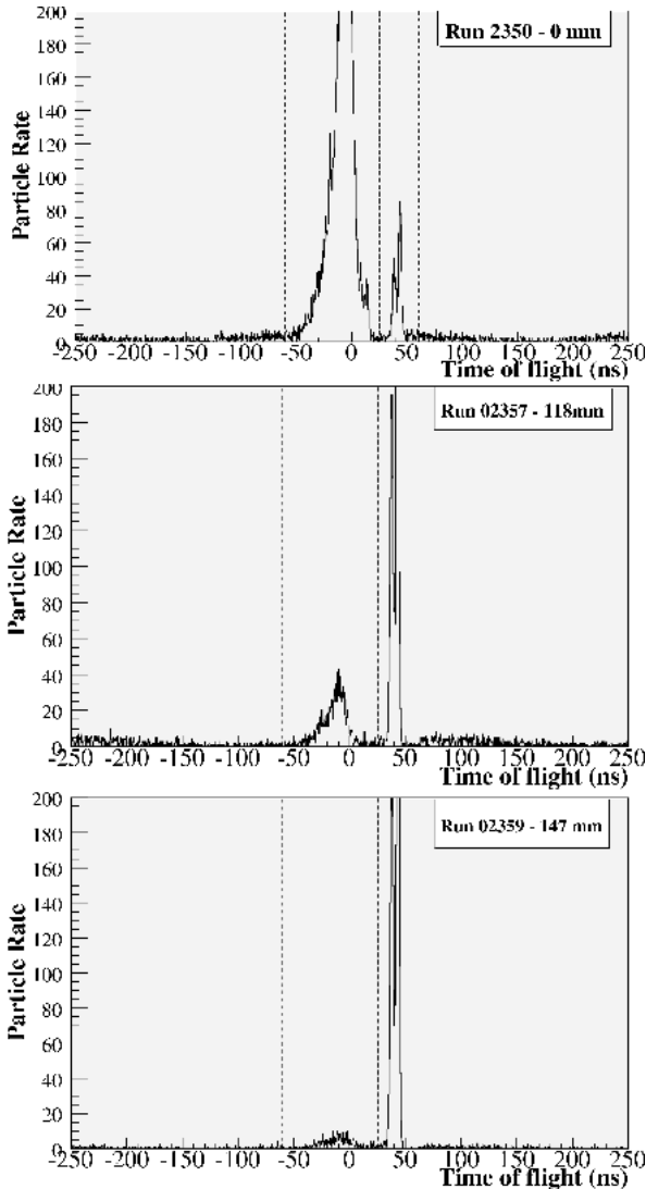
Figure 4: Particle rate for the time of flight between GVA1 and TOF0 for the 240 MeV/c beam line setting. The left population consists of protons, and the right population is muons/pions/positrons. The time of flight appears “negative” for some particles due to an offset between the TOF0 gate and GVA1 TDC. The proton absorber thickness is increased moving from top to bottom.
