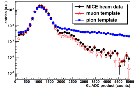
Figure 6 Determination of MICE muon beam purity using the KL detector. A pion contamination in the muon beam at or below the 1% level is determined [10].
