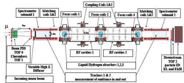
Figure 1 Layout of MICE
