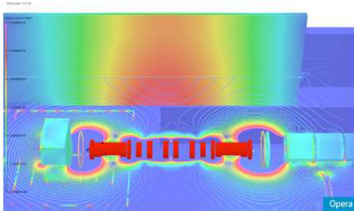
Figure 9 Stray magnetic field in the MICE hall, step VI.
