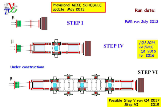
Figure 2 MICE implementation in steps
