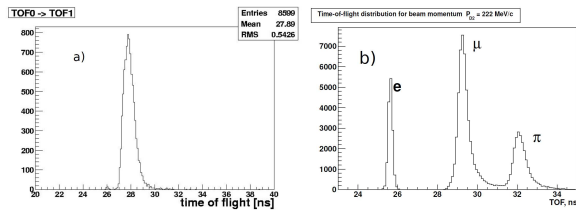
Figure 4 Time of flight (TOF1-TOF0) for (a) the ‘muon beam’ ( P_2 \sim 0.6 P_1 ) and (b) a pion beam ( P_2 \sim P_1 ).
