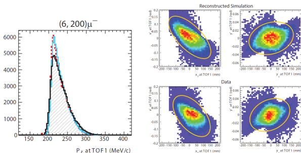
Figure 5 Left: beam momentum in the nominal MICE muon beam. Red, blue and black shaded distributions are simulation, reconstructed simulation and data respectively. Right: Horizontal ( x, x' ) and vertical ( y, y' ) trace space distributions at TOF1 for simulation (top) and data (bottom) in the MICE nominal muon beam [9].
