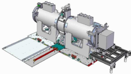
Figure 7 MICE Step IV (engineering drawing)
