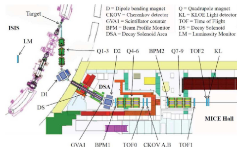
Figure 3 Layout of the MICE beam-line at ISIS.
