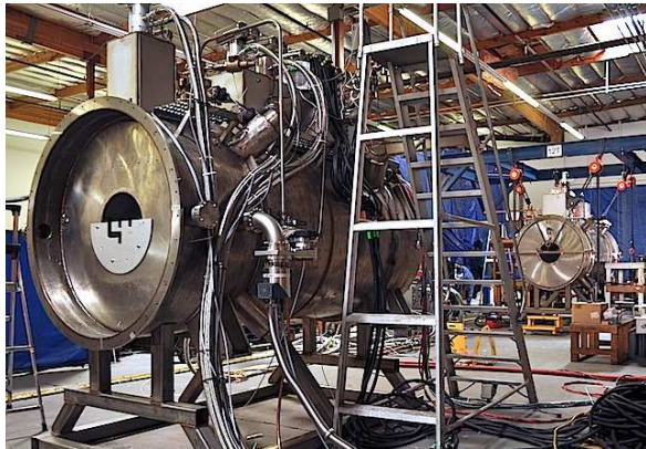
Figure 8 Spectrometer solenoids at Wang NMR, Inc. of Livermore, CA.
